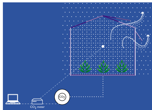
Figure 2-3: Increased CO 2 concentration, due to CO 2 enrichment Source: Elly Nederhoff, 2004
