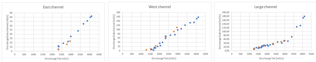
Figure 2.1.5: Discharge partitioning between main channel and side channels. In blue, the measurements of 2001-2002, in yellow the measurements of 2018-2019. In that latter period, the maximal discharge was 2938 m 3 /s for the main channel (x-axis).
