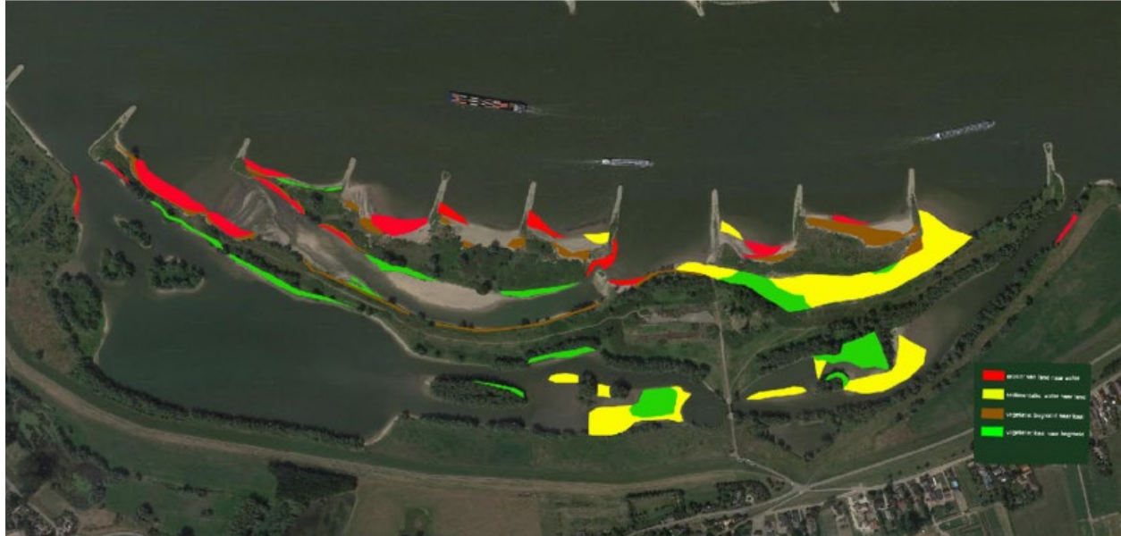
Figure 2.1.3: A result from the detailed study on the Gameraen side channel system. Red indicates erosion, yellow is sedimentation, green is emerged vegetation and brown is disappeared vegetation, always between 2000 and 2019.
