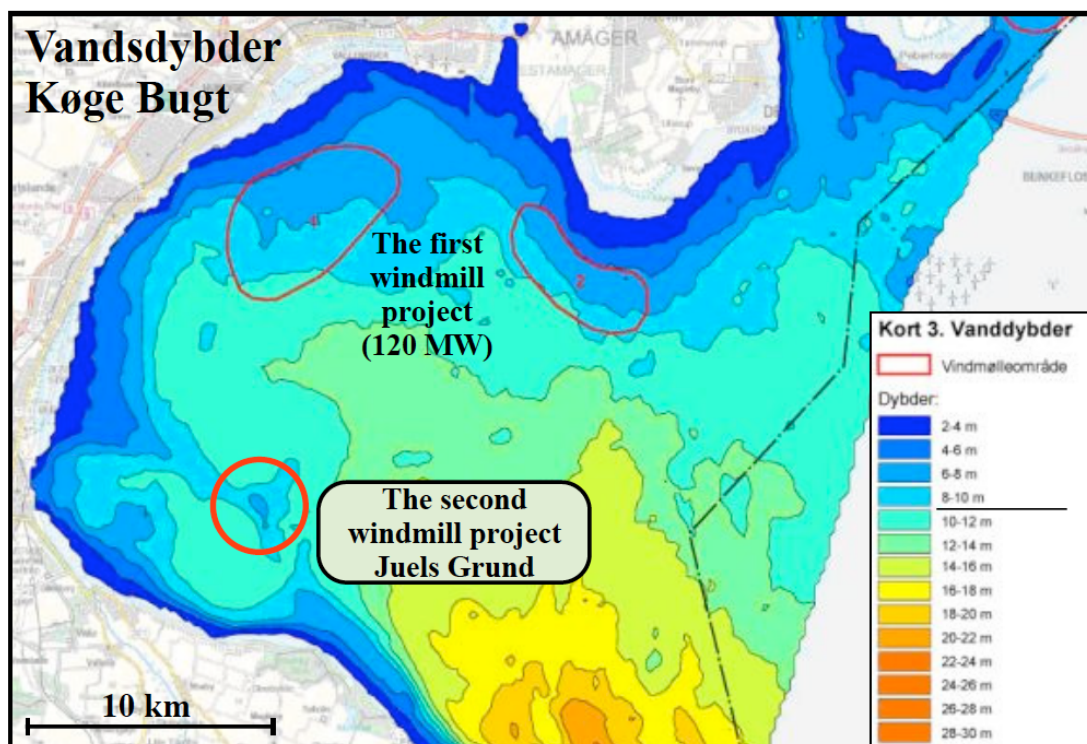
Figure 1. Water depth and location of proposal for coastal sea windmill project in Køge Bay.
