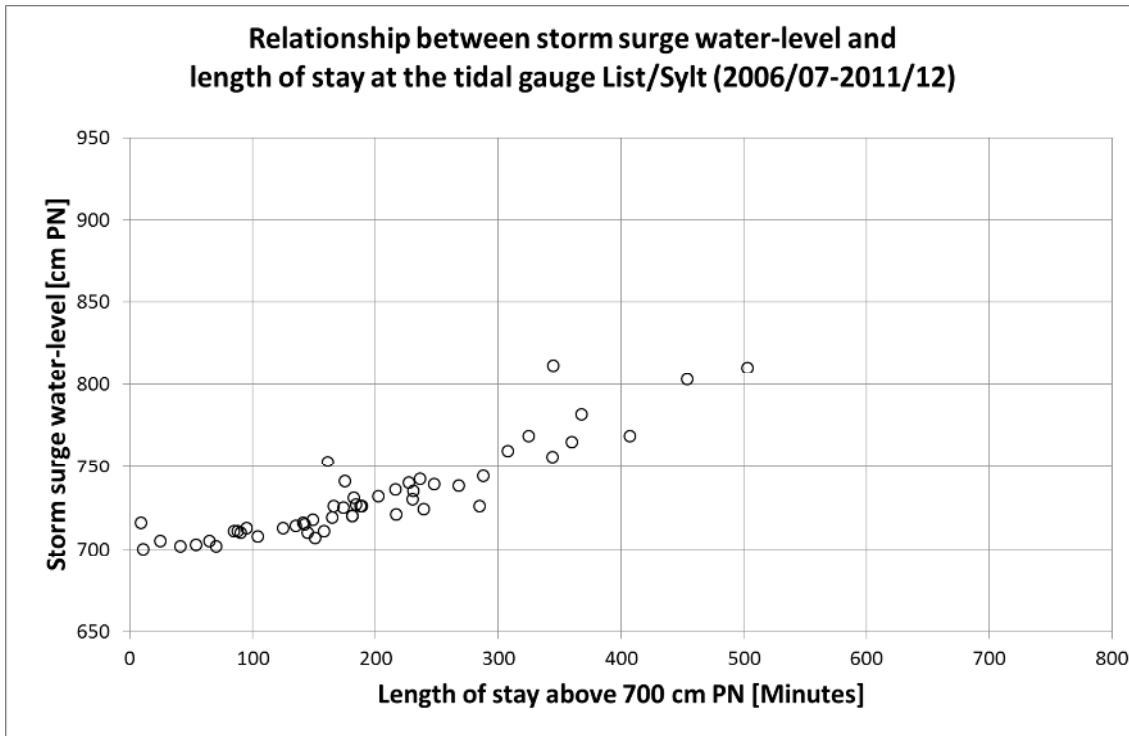
Figure 55: Relationship between storm surge water-level and length of stay at the tidal gauge harbour List/Sylt between 2006/2007 and 2011/12.
