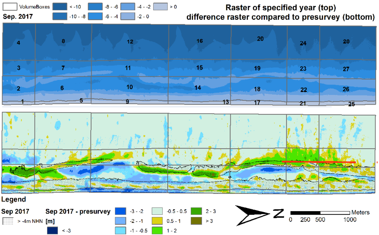
Figure 53: Comparison of terrain raster and difference raster for Sep. 2017 (red line is nourishment site).
