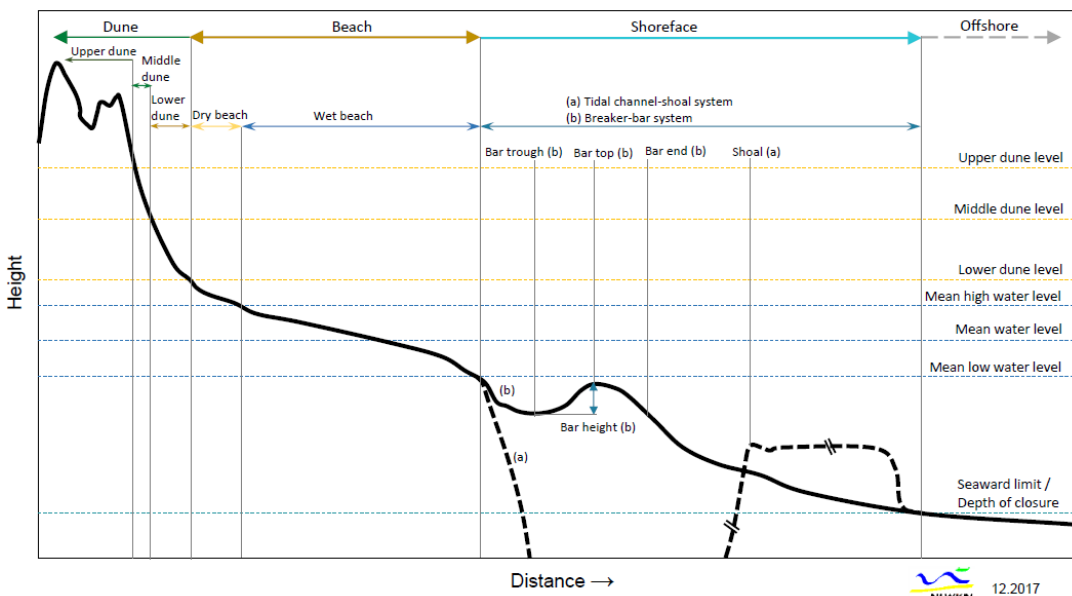
Figure 15: General terminology used to describe the coastal profile. On the vertical axis various levels in the profile are shown. The horizontal axis shows different Morphological zone in the profile.
