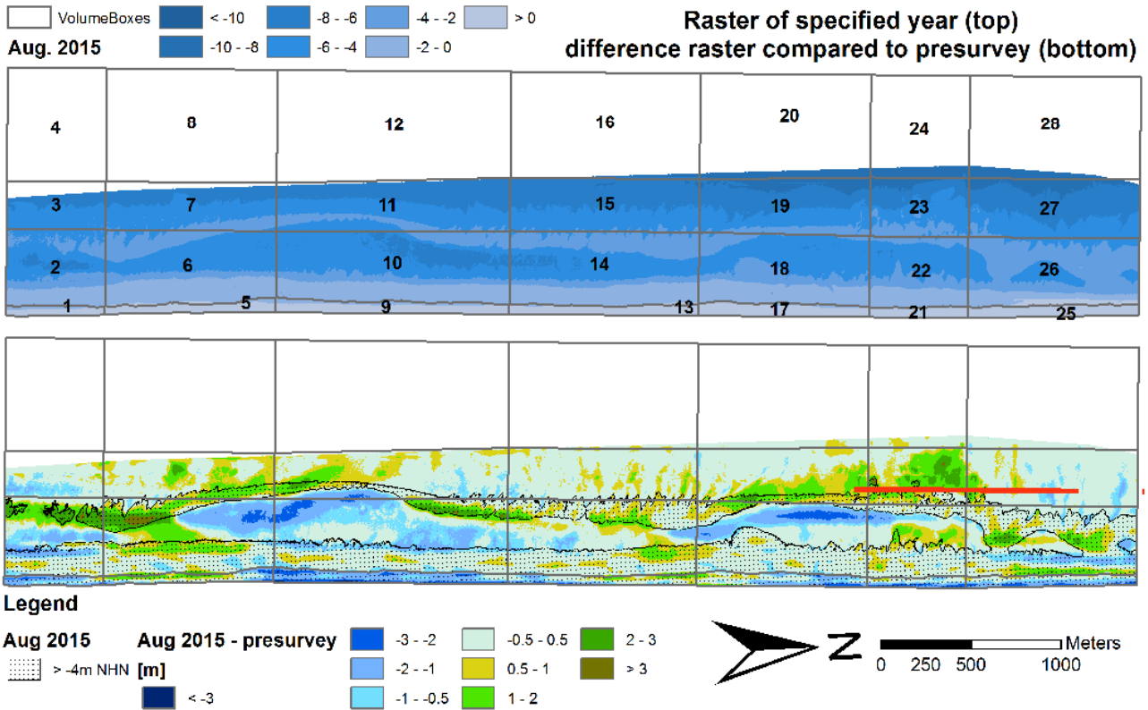
Figure 52: Comparison of terrain raster and difference raster for Aug. 2015 (red line is nourishment site).
