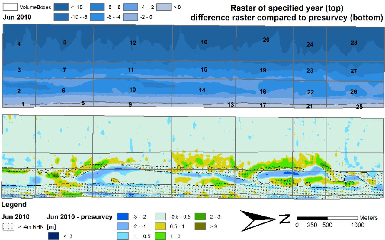
Figure 51: Comparison of terrain raster and difference raster for Jun. 2010.
