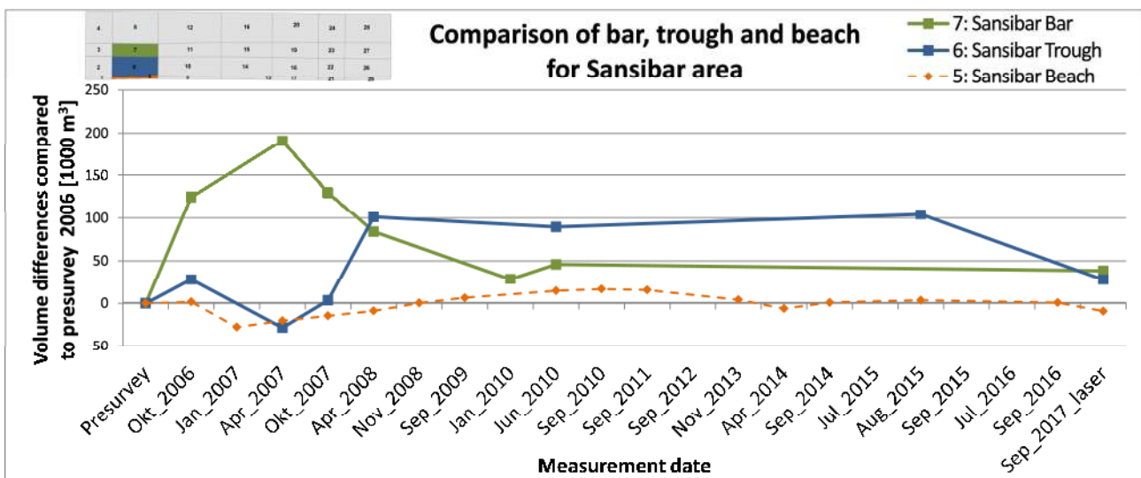
Figure 39: Trends of bar, trough and beach boxes for Sansibar.
