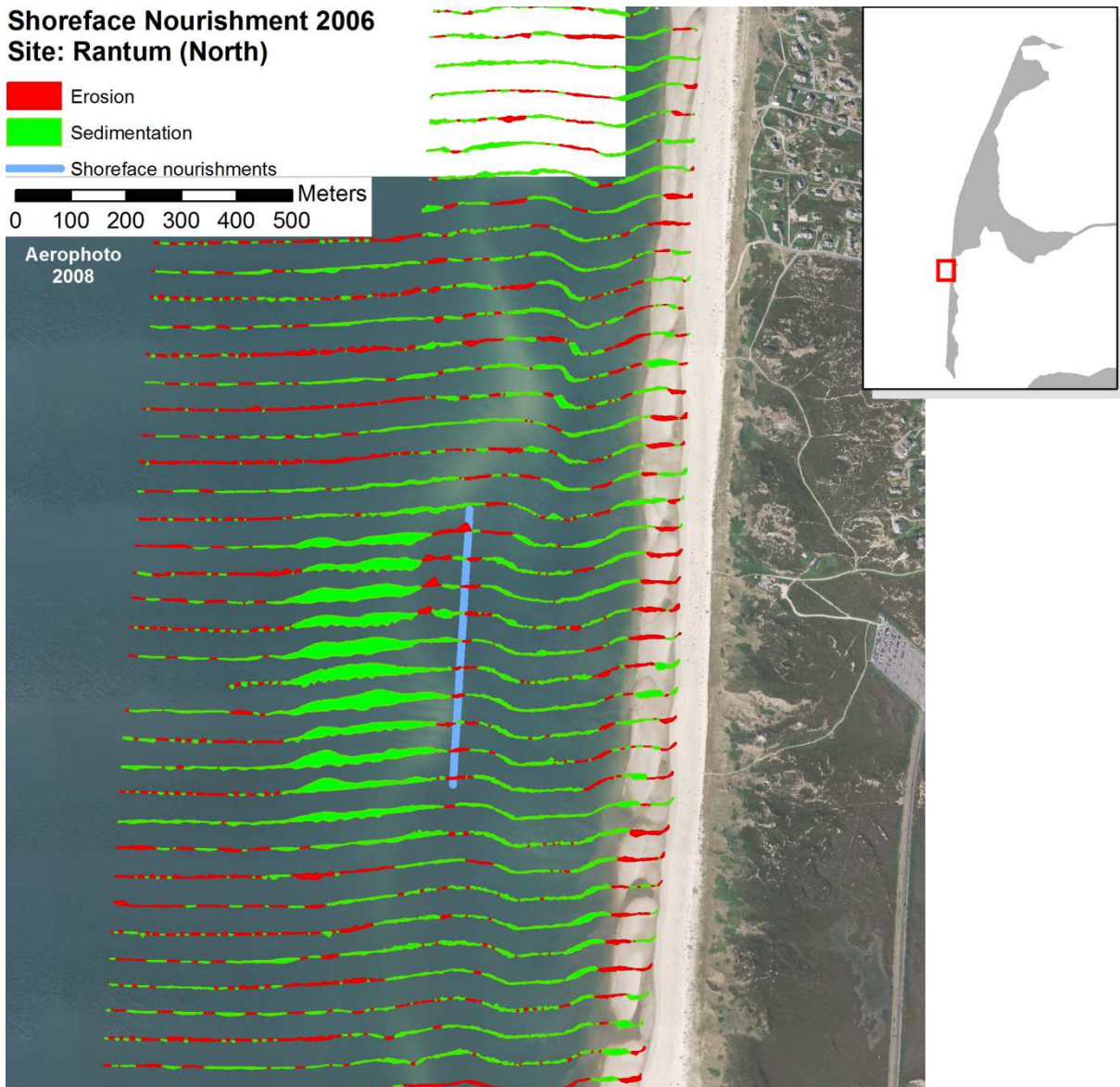
Figure 6: Cross section profile comparison, Rantum (shoreface), between 13.07.2006 and 13.09.2006.
