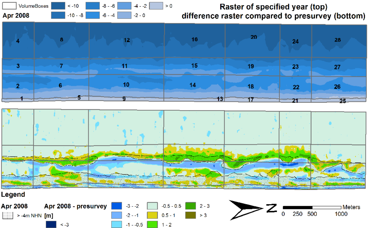
Figure 49: Comparison of terrain raster and difference raster for Apr. 2008.
