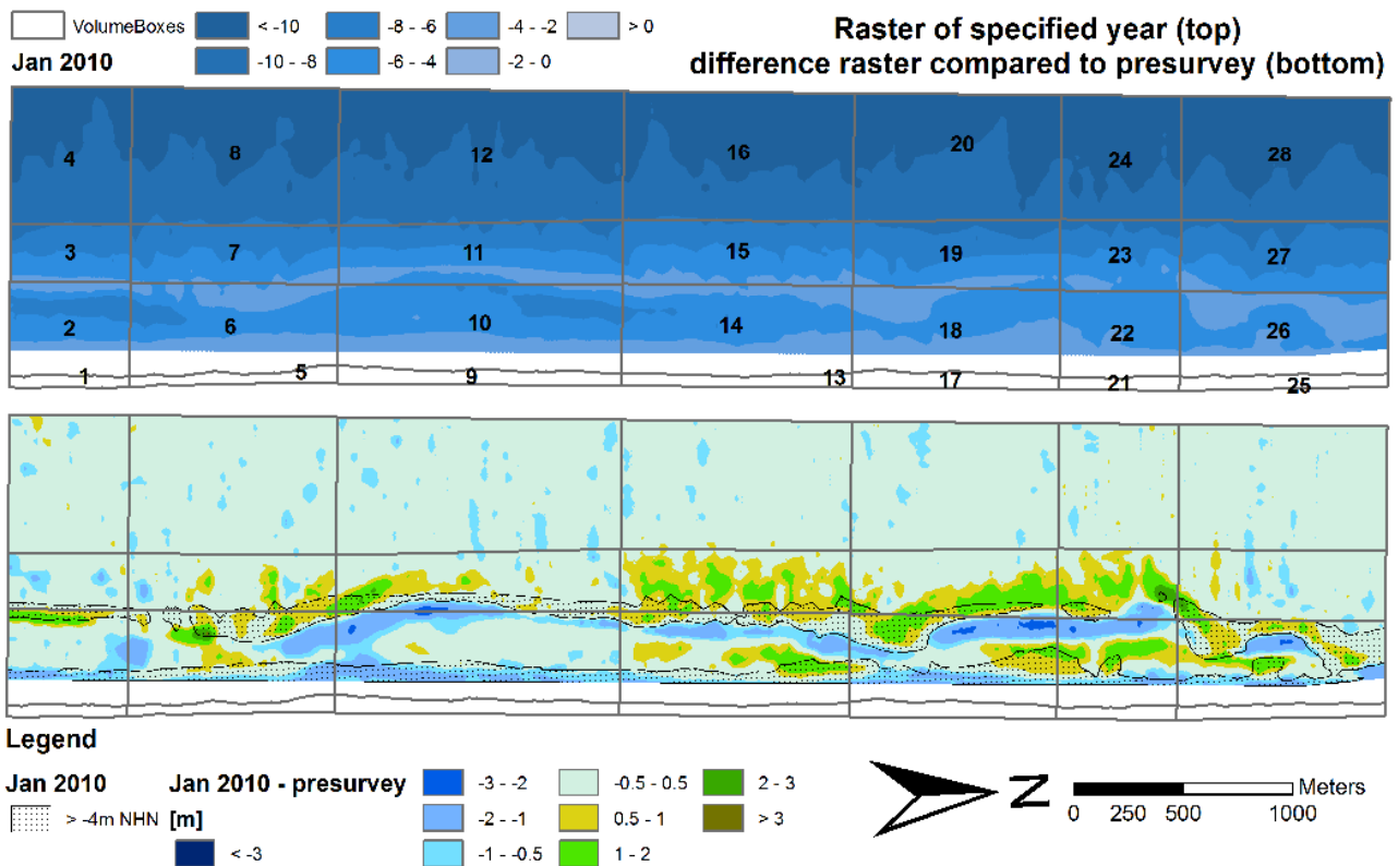
Figure 50: Comparison of terrain raster and difference raster for Jan. 2010.
