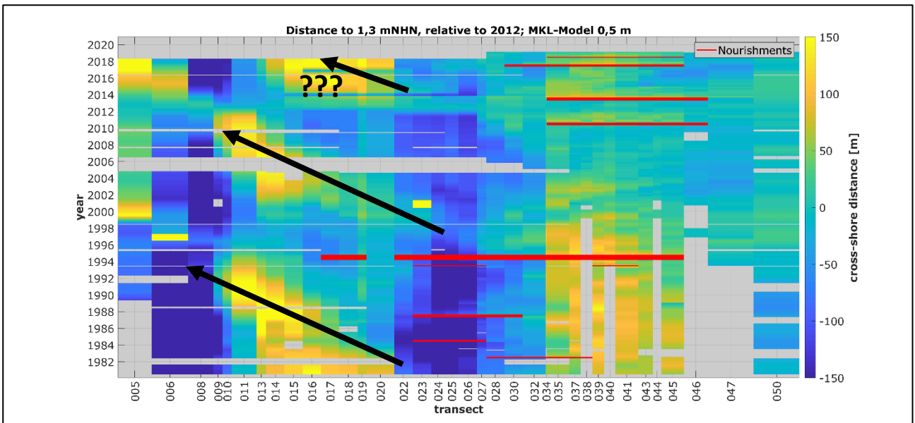
Figure 5 Time Distance Diagram of the main transects of Langeoog. Arrows indicate sand migration on the western head of the island from north to south.
