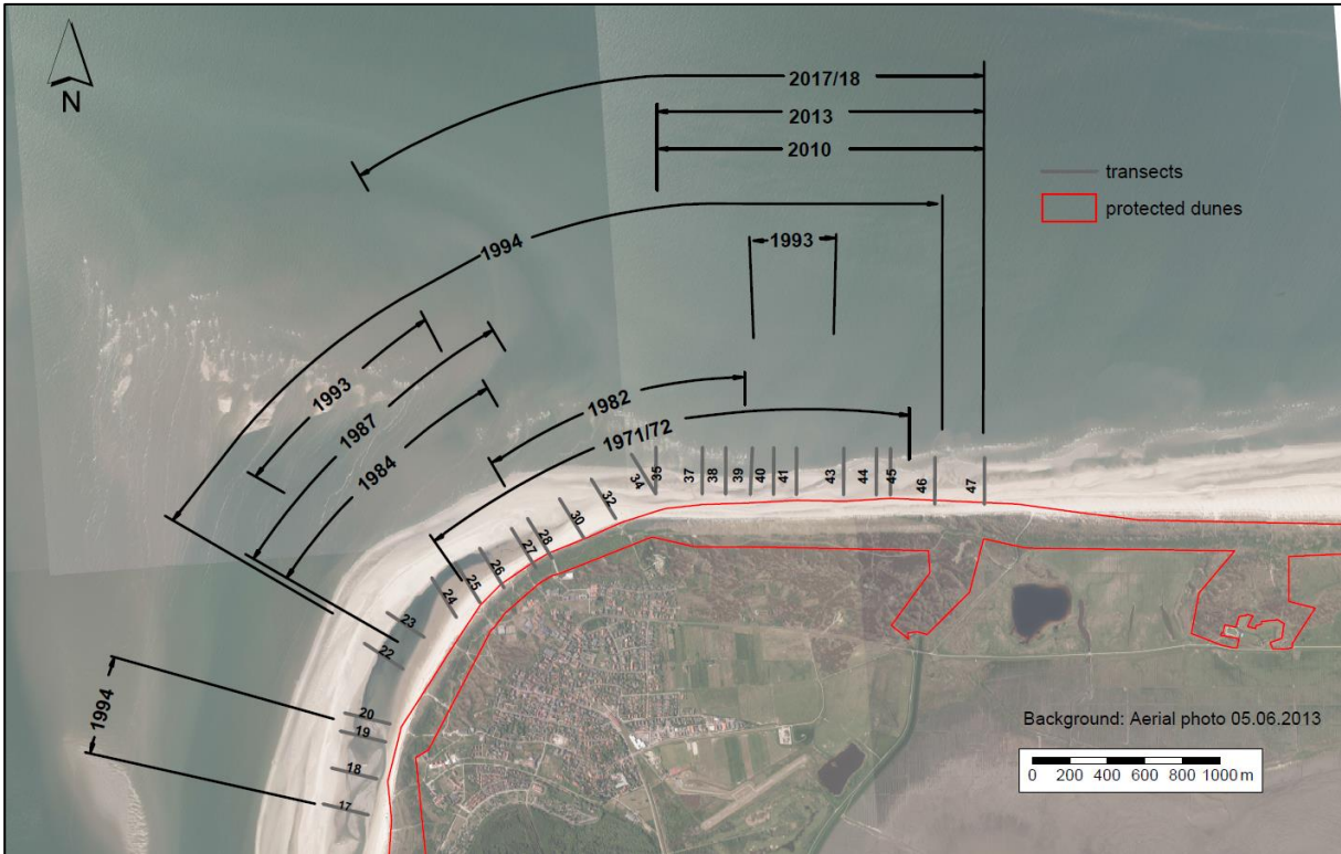
Figure 9 Historical beach nourishments at western part of Langeoog since 1971/72 up to 2018
