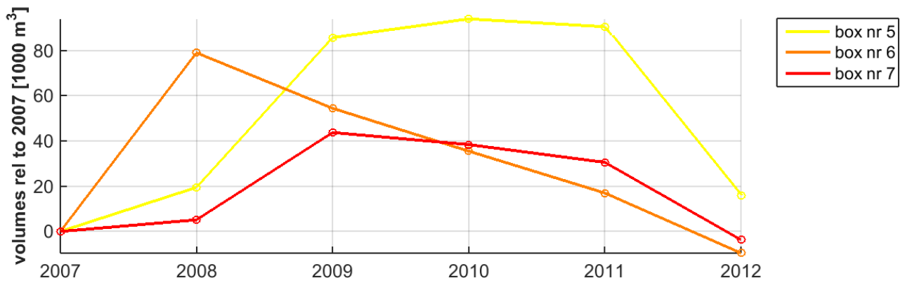
Figure 55 Volume development from one year before the nourishment until the last year before the next nourishment
