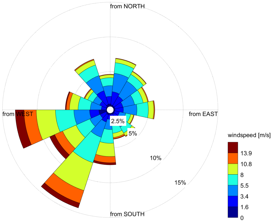
Figure 28: Wind conditions for the long term, pre nourishment period 1989-2008
