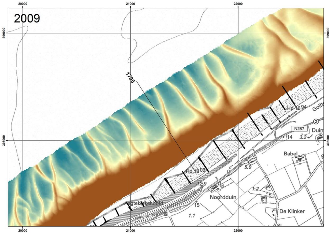
Figure 33: Multibeam bathymetry of shoreface close to Domburg (source: Mastbergen et al., 2017)
