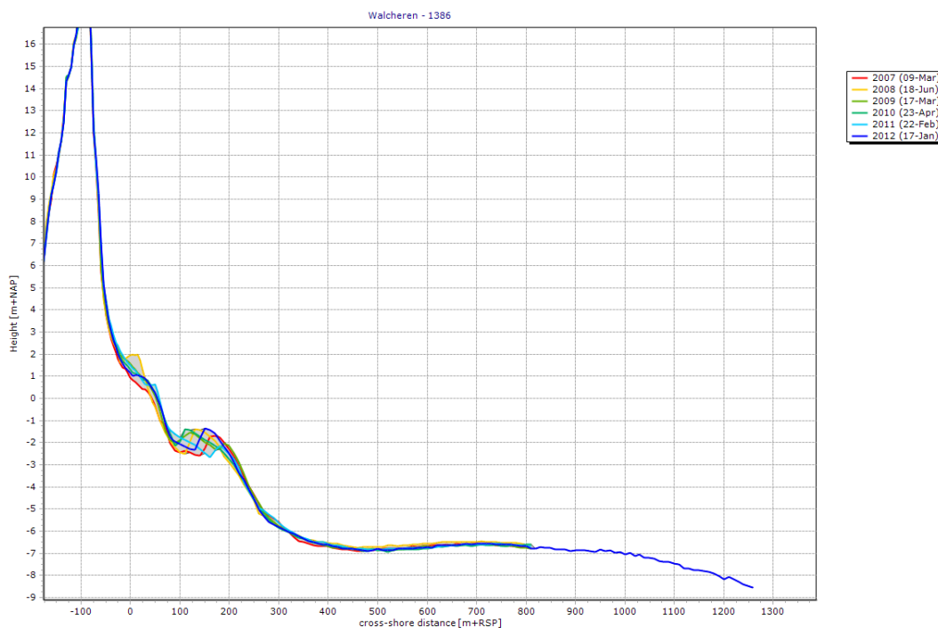
Figure 31: Development of shoreface in transect 1386 between 2007 and 2012
