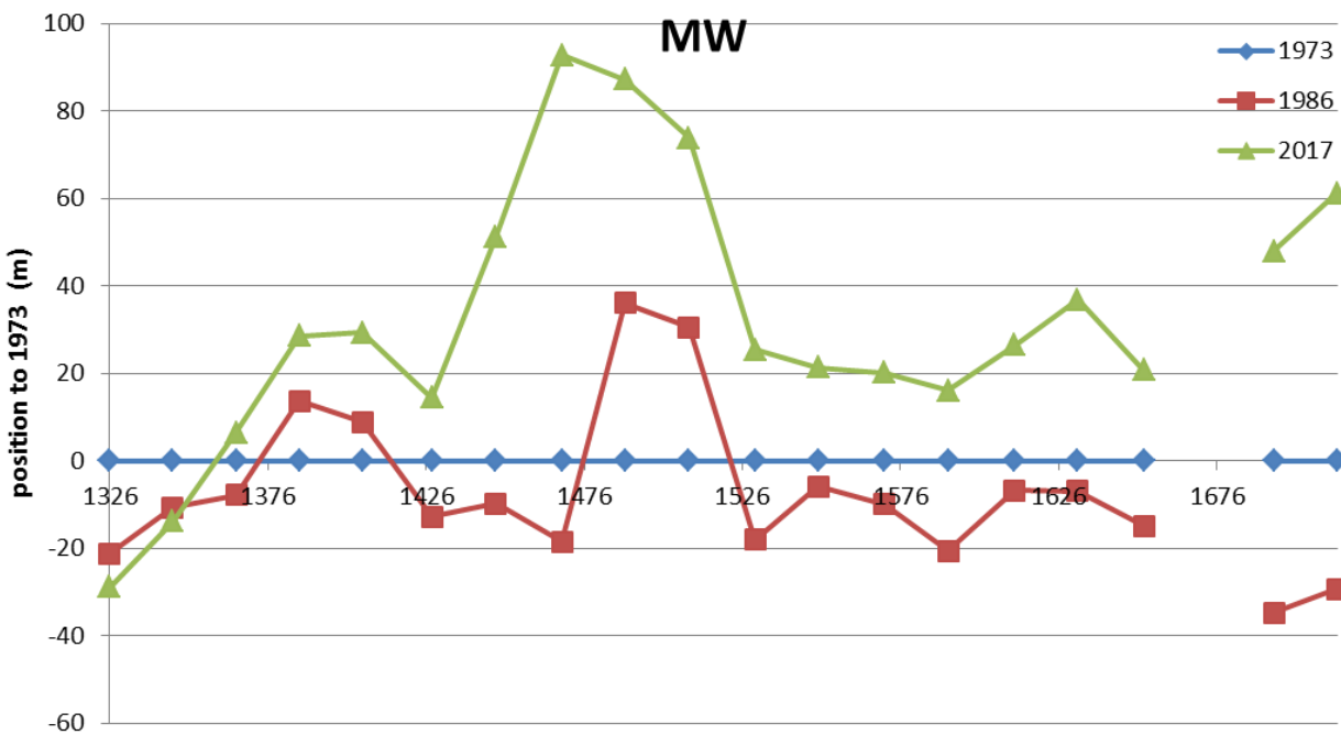
Figure 52: Position of the mean water level for studied transects in 1973, 1986 and 2017
