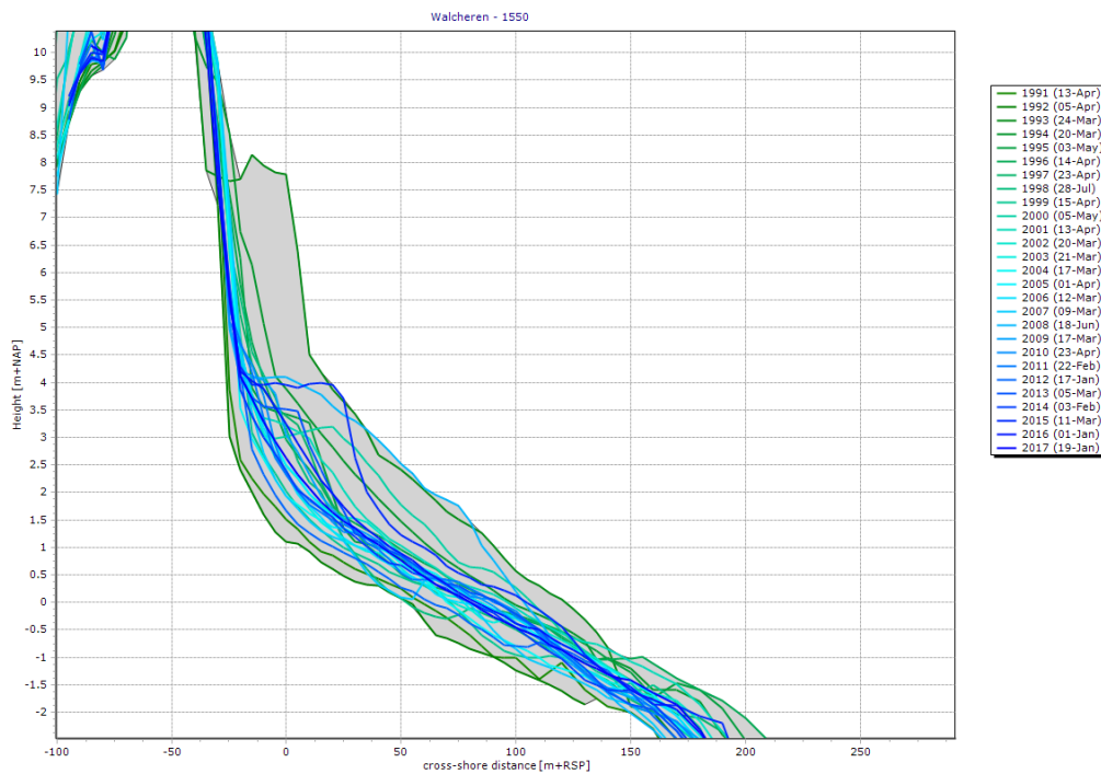
Figure 41: Development of beach and dune in transect 1550 between 1990 and 2017
