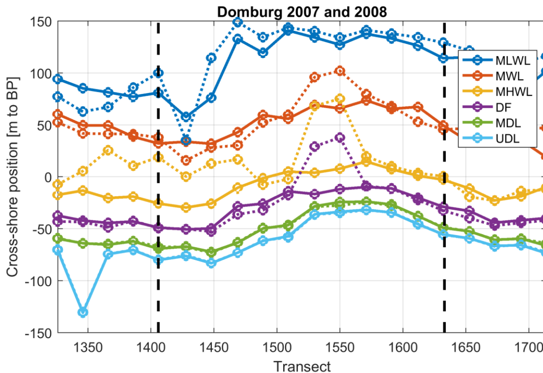
Figure 42: The physical marks of the transects at Domburg for the year 2007 (solid line) and the year 2008 (coloured dashed line). The colours indicate the defined level, see 4.2.1. The black dashed line indicates the prescribed boundary of the nourishment.
