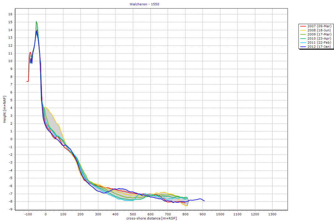
Figure 32: Development of shoreface in transect 1550 between 2007 and 2012
