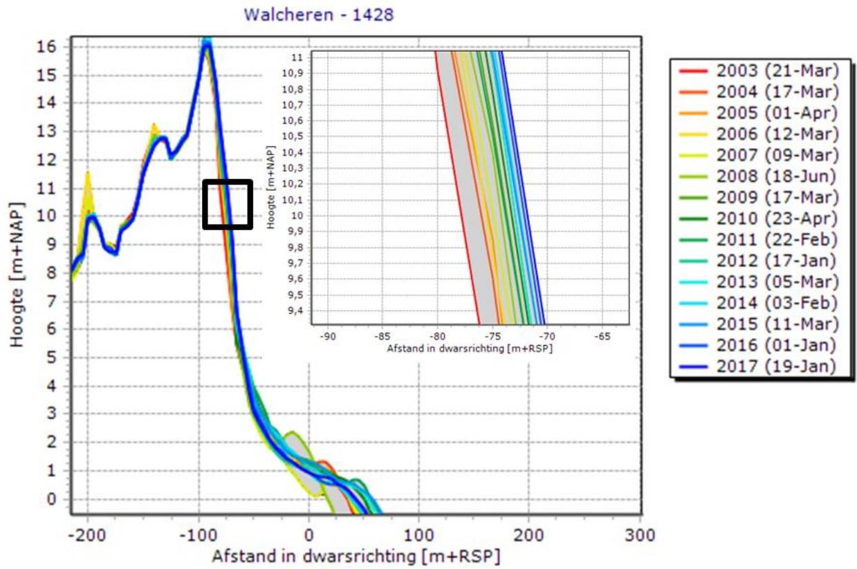
Figure 47: The dune profile for transect 1428 for the years 2003 till 2017. The colours represent various years. The figure also contains a zoom in of the profile. The black square indicates the location off the zoom in.
