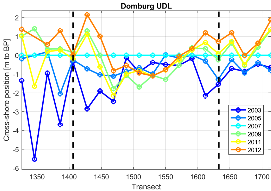
Figure 46: The difference in cross-shore position of MHWL with respect to 2007. When the value is positive the position lays more offshore than in 2007.
