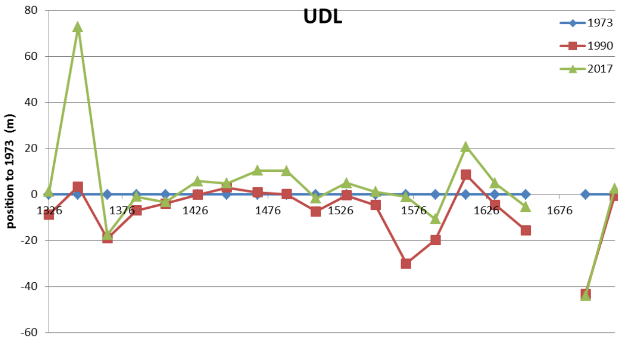
Figure 48: Position of the upper dune level for studied transects in 1973, 1990 and 2017
