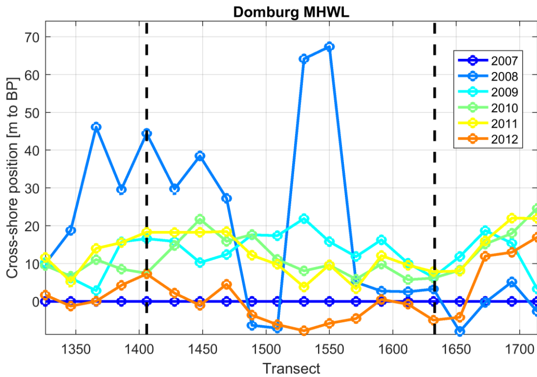
Figure 43: The difference in cross-shore position of MHWL with respect to 2007. When the value is positive the position lays more offshore than in 2007.
