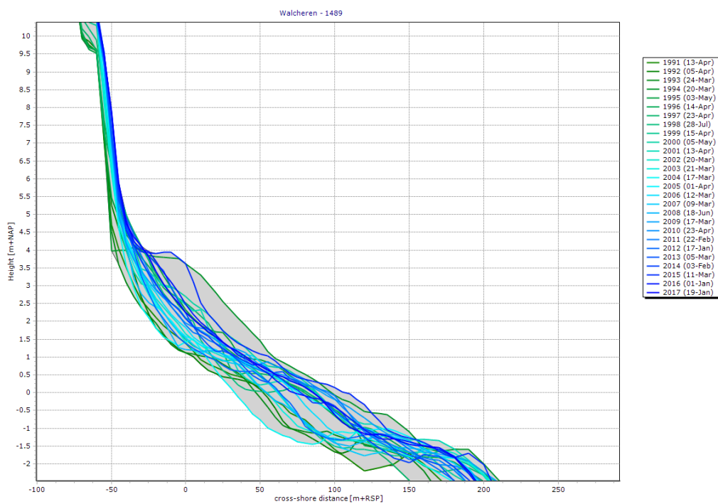
Figure 40: Development of beach and dune in transect 1489 between 1990 and 2017
