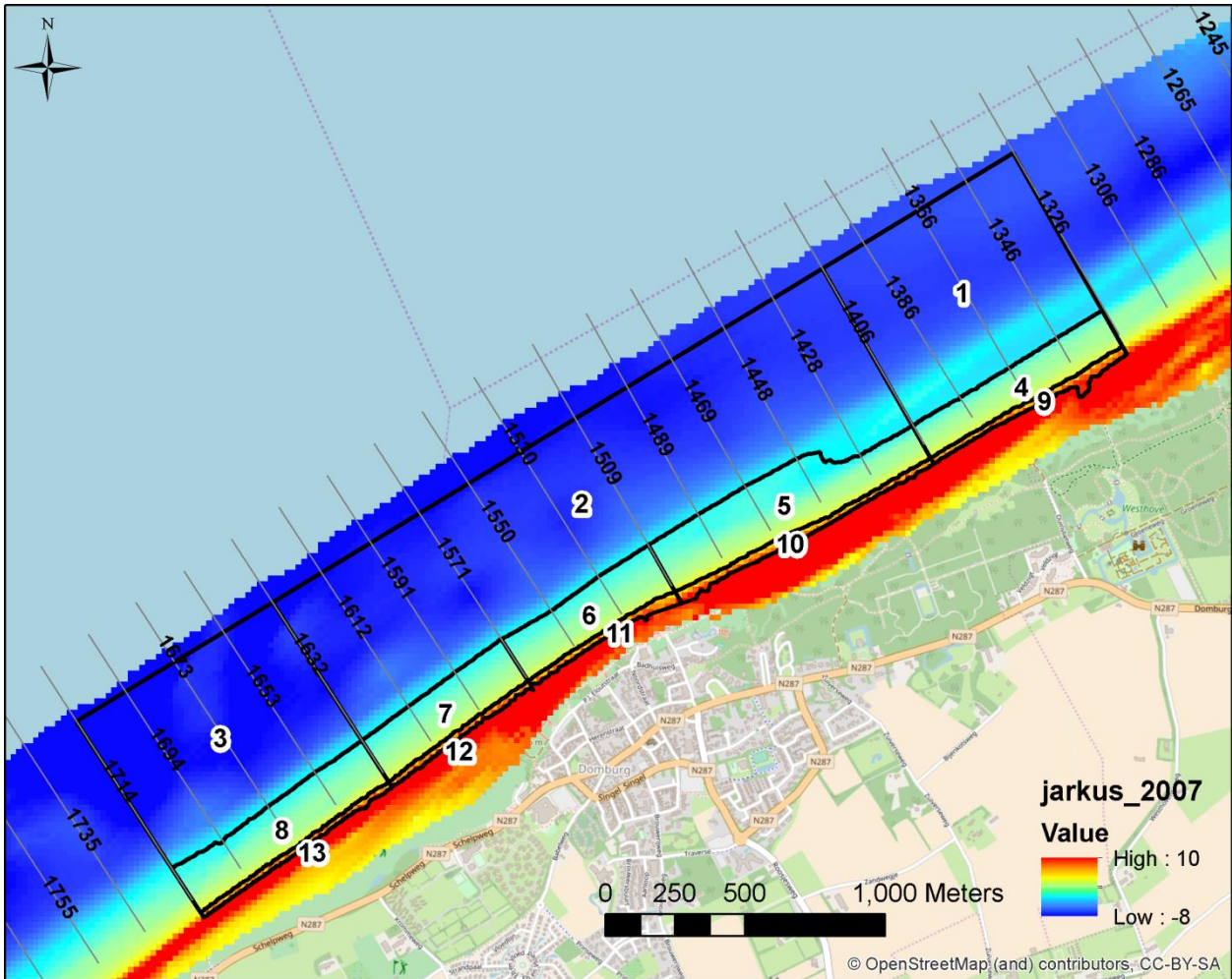
Figure 54 Areas used for calculation of volumes
