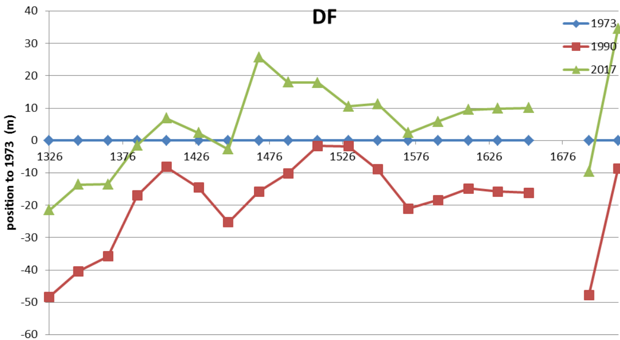
Figure 50: Position of the dune foot for studied transects in 1973, 1990 and 2017
