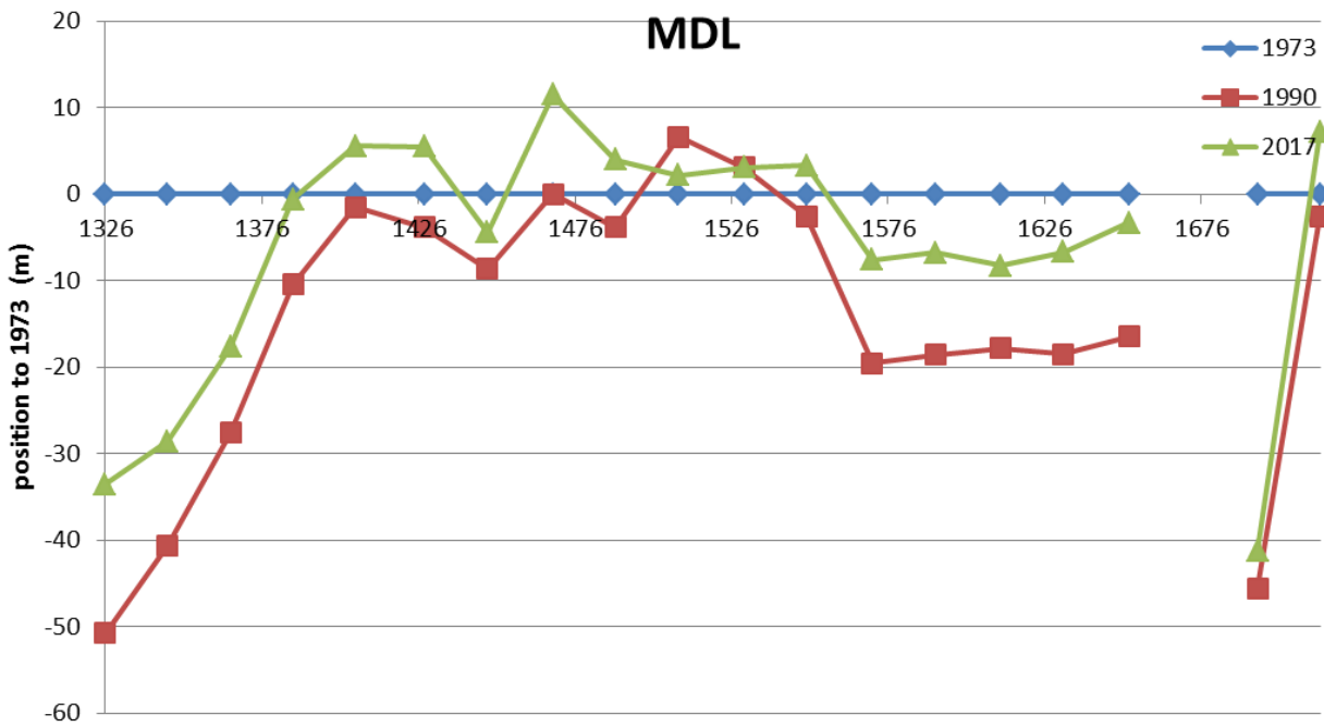
Figure 49: Position of the middle dune level for studied transects in 1973, 1990 and 2017
