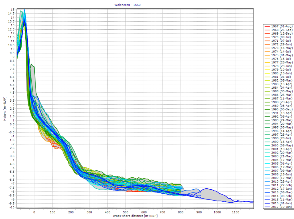
Figure 35: Development of shoreface in transect 1550 between 1967 and 2017
