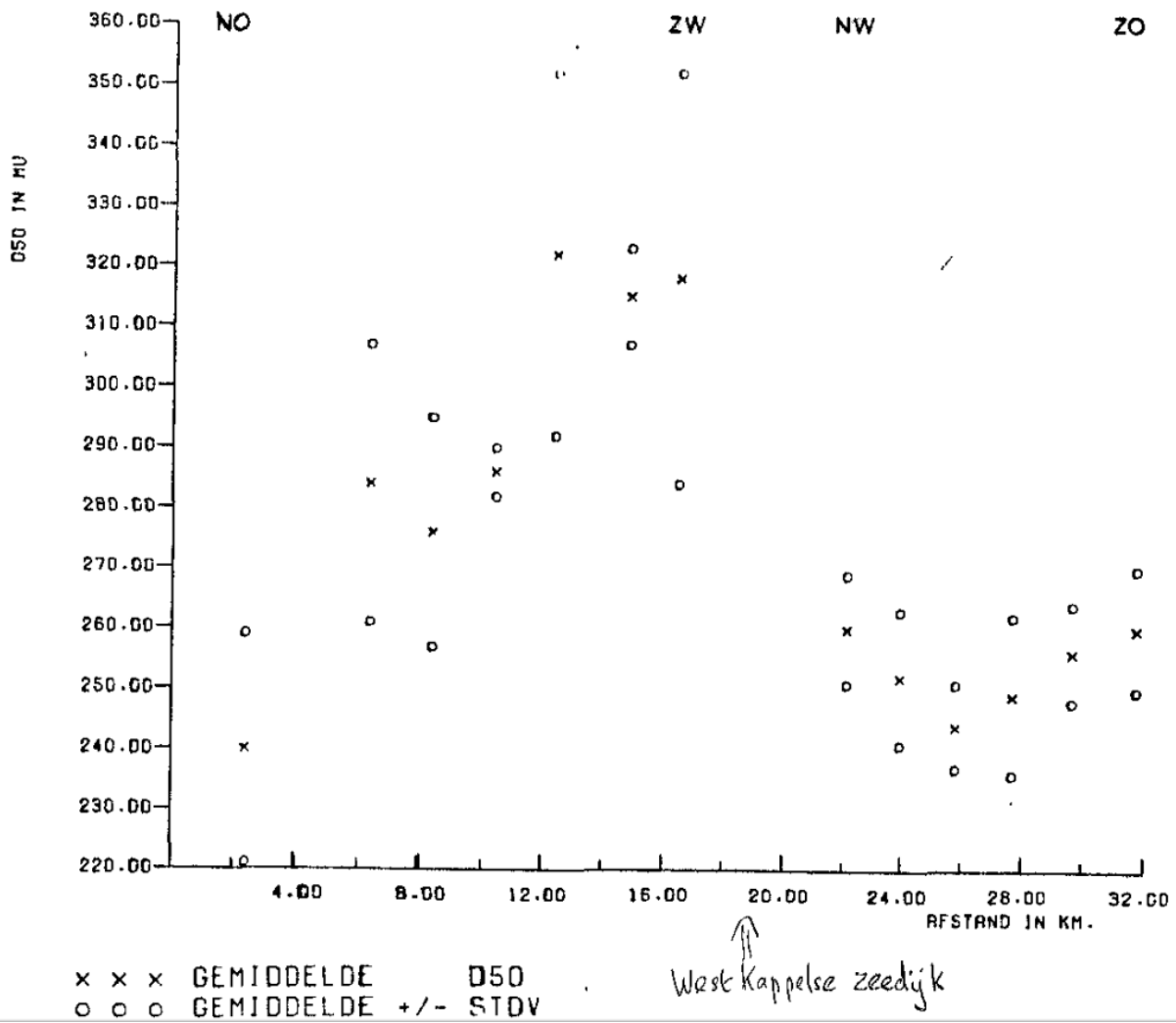
Figure 30: Average median grain size for the dunes of Walcheren, the studied nourishment is around 15.00 with a D50 around 300 micron. Source: Koksiek (1984)
