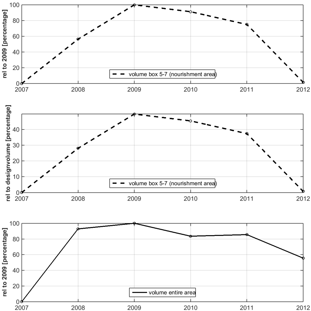
Figure 57 Volume development in percentages for nourishment area relative to maximum volume in 2009 (top), relative to design volume of 370.000 m 3 (middle) and for entire area (area 1-8) relative to maximum volume (bottom)
