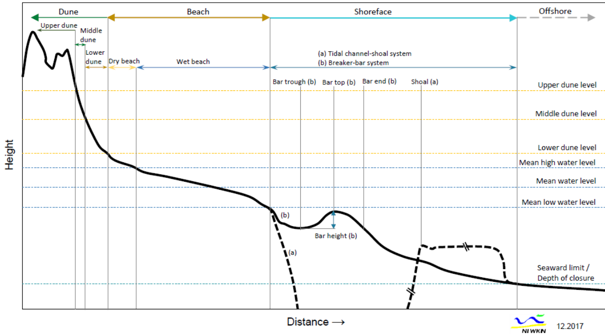
Figure 13: General definition/terminology coastal profile used. On the vertical axis various levels in the profile are shown. The horizontal axis shows different zones in the profile. Source: Simon Hillmann (NLWKN)
