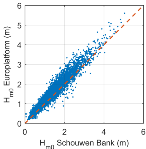
Figure 17: A scatterplot of the H_s measured at the Schouwen Bank and at the Europlatform from 2004 till 2008.
