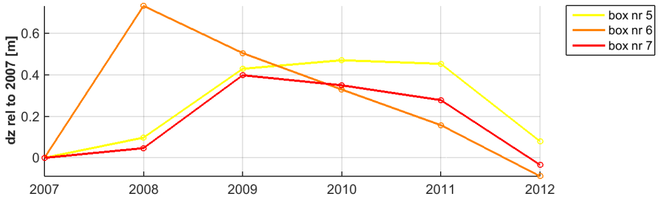
Figure 58 Change in average bed level for each polygon
