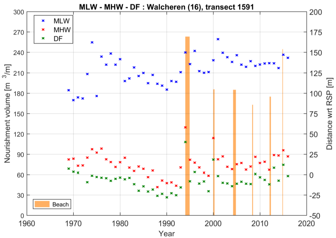
Figure 44: Long term location of the MLW (Mean Low Water), MHW (Mean High Water) and the Dune Foot (DF) as a function of time for transect 1591. The orange bars indicate the volume for a nourishment.
