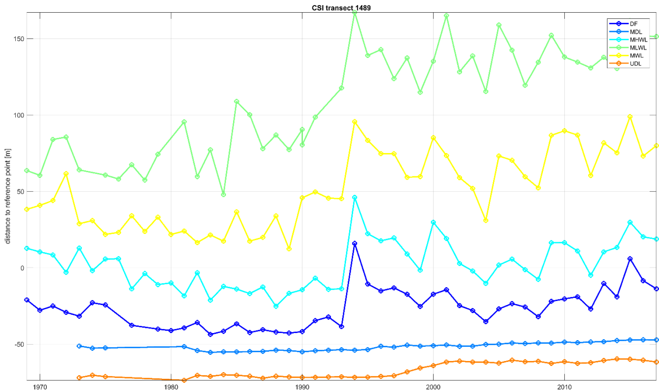
Figure 45: Timeseries of physical marks for transect 1489
