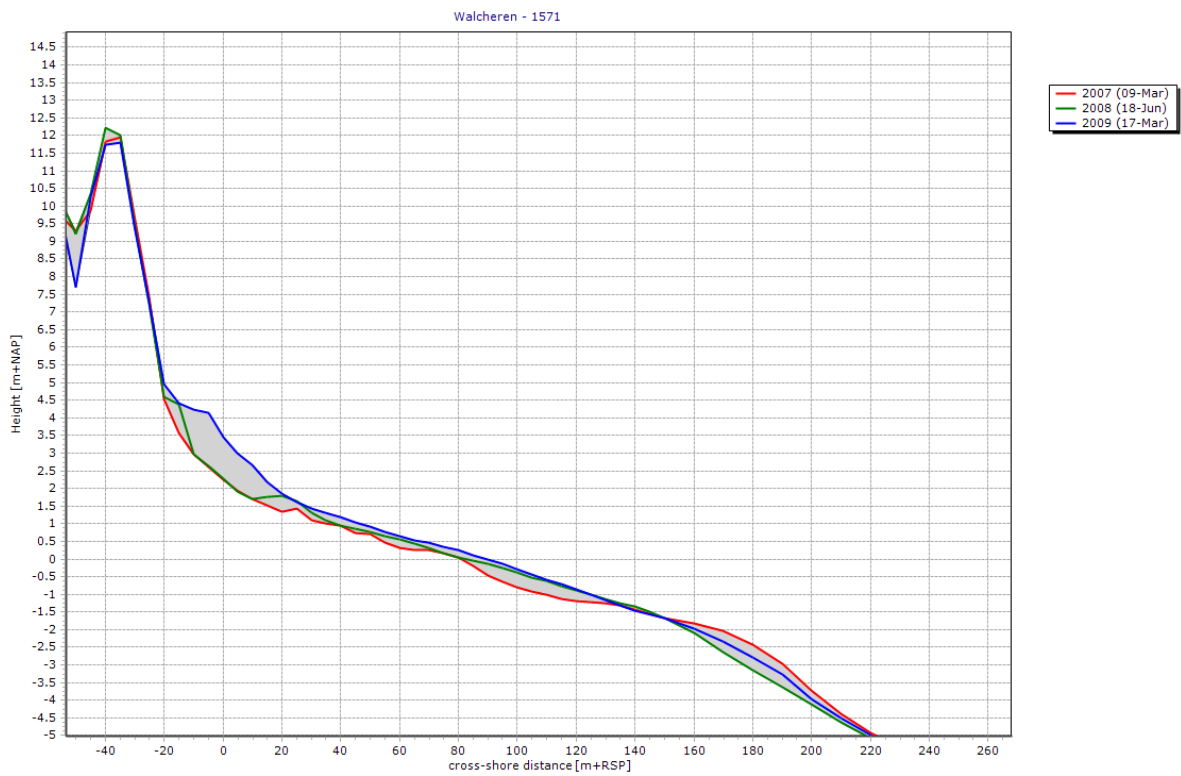
Figure 9: Placement of nourishment in transect 1571
