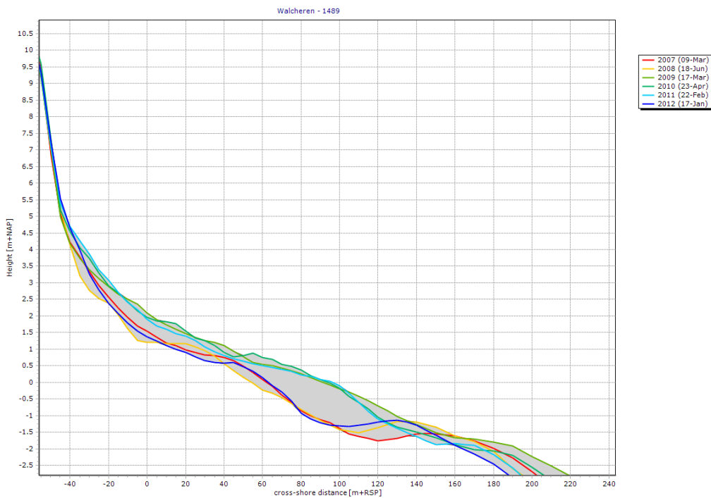
Figure 36: Development of beach and dune in transect 1489 between 2007 and 2012
