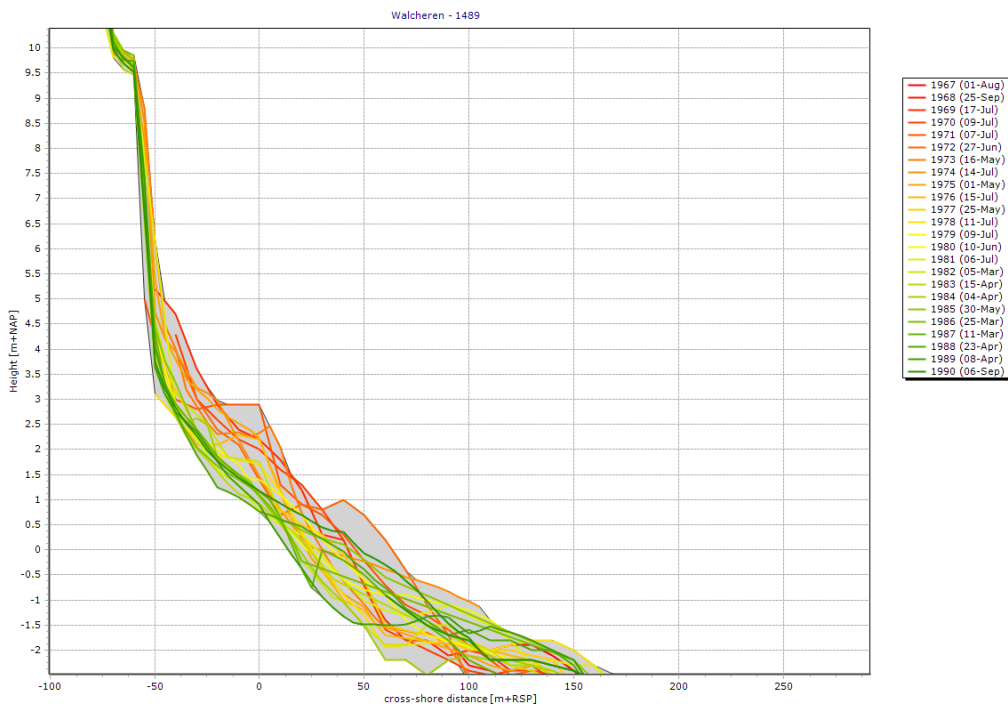
Figure 38: Development of beach and dune in transect 1489 between 1967 and 1990.
