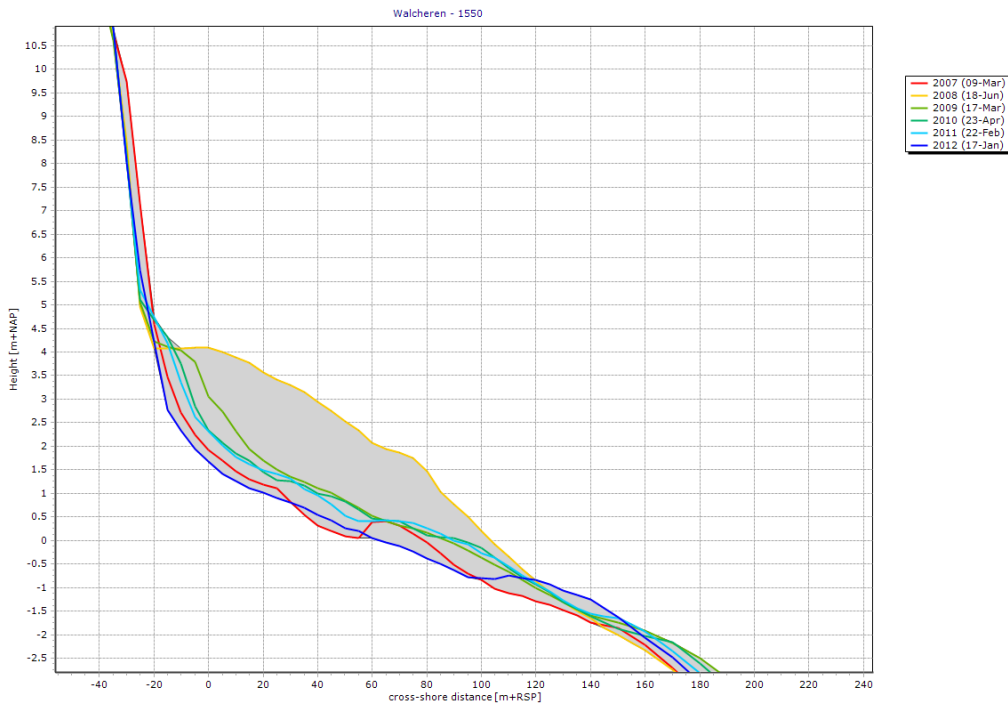
Figure 37: Development of beach and dune in transect 1550 between 2007 and 2012.
