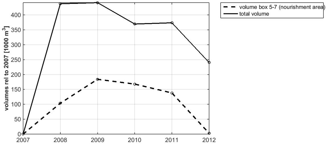
Figure 56 Volume development nourishment polygons (5-7) and polygons 1-8 (total volume)
