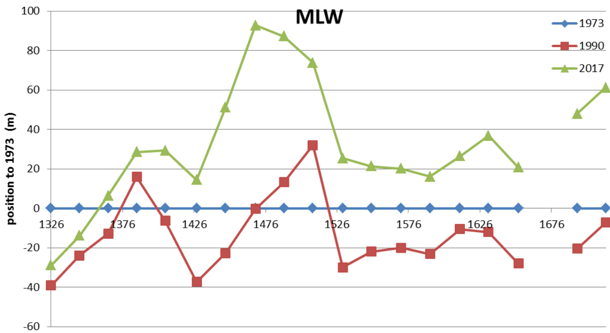
Figure 53: Position of the mean low water level for studied transects in 1973, 1990 and 2017
