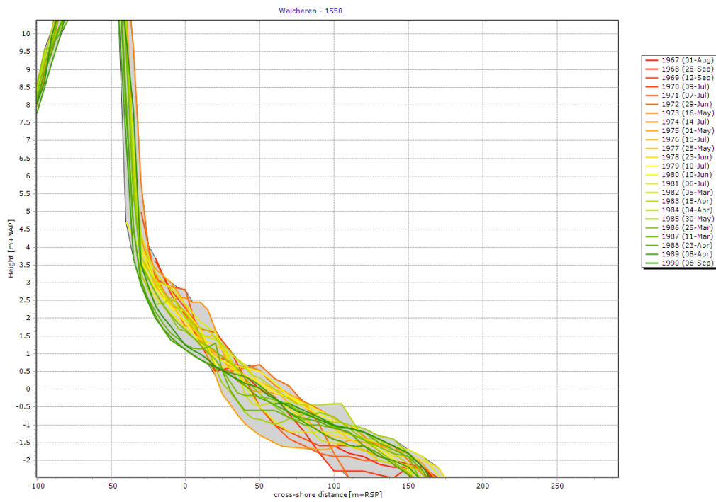
Figure 39: Development of beach and dune in transect 1550 between 1967 and 1990.
