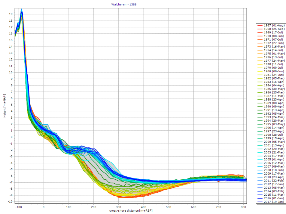
Figure 34: Development of shoreface in transect 1386 between 1967 and 2017
