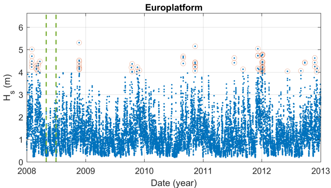
Figure 27: A time series of the wave height. The red circles indicate the events with H_s > 4m and the green lines the start and end time the nourishment.
