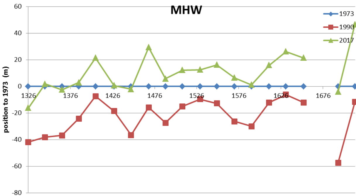
Figure 51: Position of the mean high water level for studied transects in 1973, 1990 and 2017
