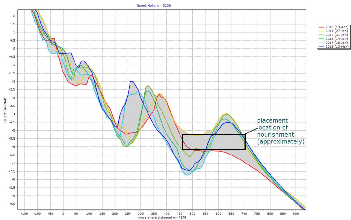
Figure 25: Profile 3200 showing the shoreface at the north side of the shoreface nourishment
