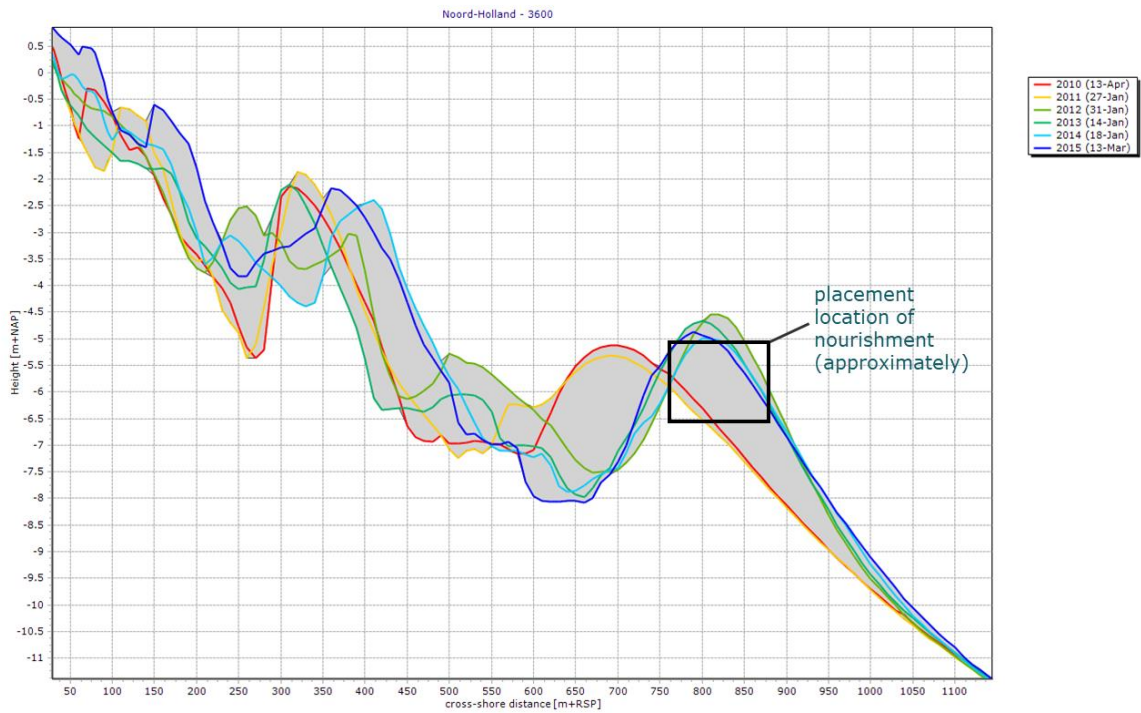
Figure 26: Profile 3600 showing the shoreface in the central part of the shoreface nourishment
