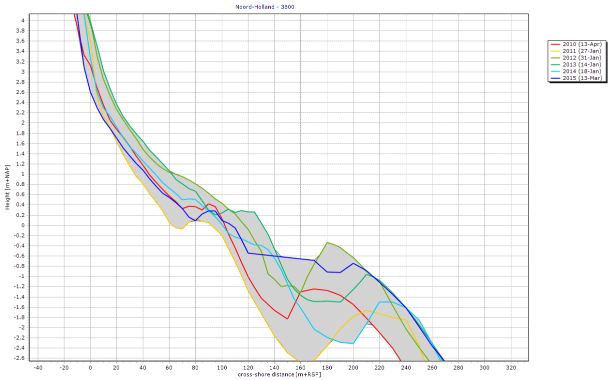
Figure 34: Profile 3800 showing the zone around the beach in at the centre of the southern beach nourishment
