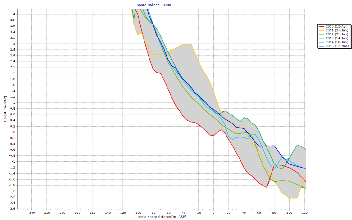
Figure 30: Profile 3300 showing the zone around the beach at the centre of the northern beach nourishment
