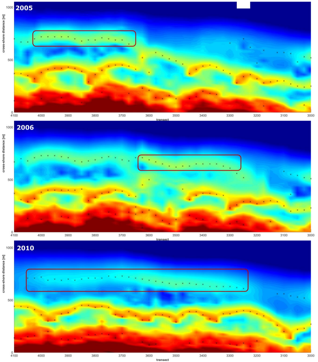
Figure 59: Bathymetry plot based on transect data (not gridded data) measured in 2005, 2006 and 2010 with the detected bar crest position indicated with crosses. The indicated areas show the shoreface nourishments of 2004 (top) and 2005 (middle), and their remaining sediment in 2010 (bottom)
