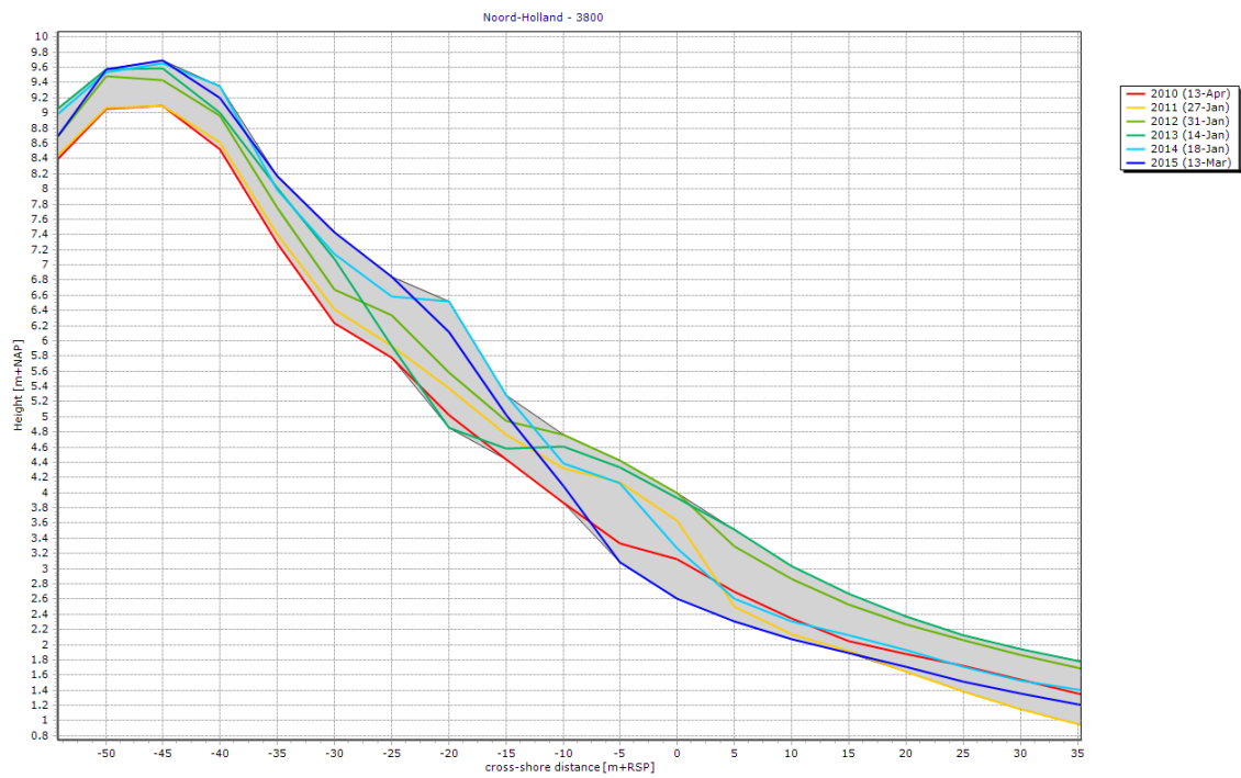
Figure 41: Profile 3800 showing the first dune at the southern beach nourishment
