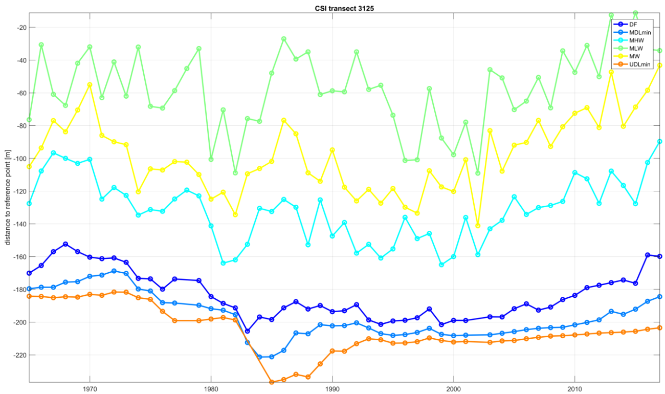
Figure 49: Development of all coastal state indicators in time for transect 3125
