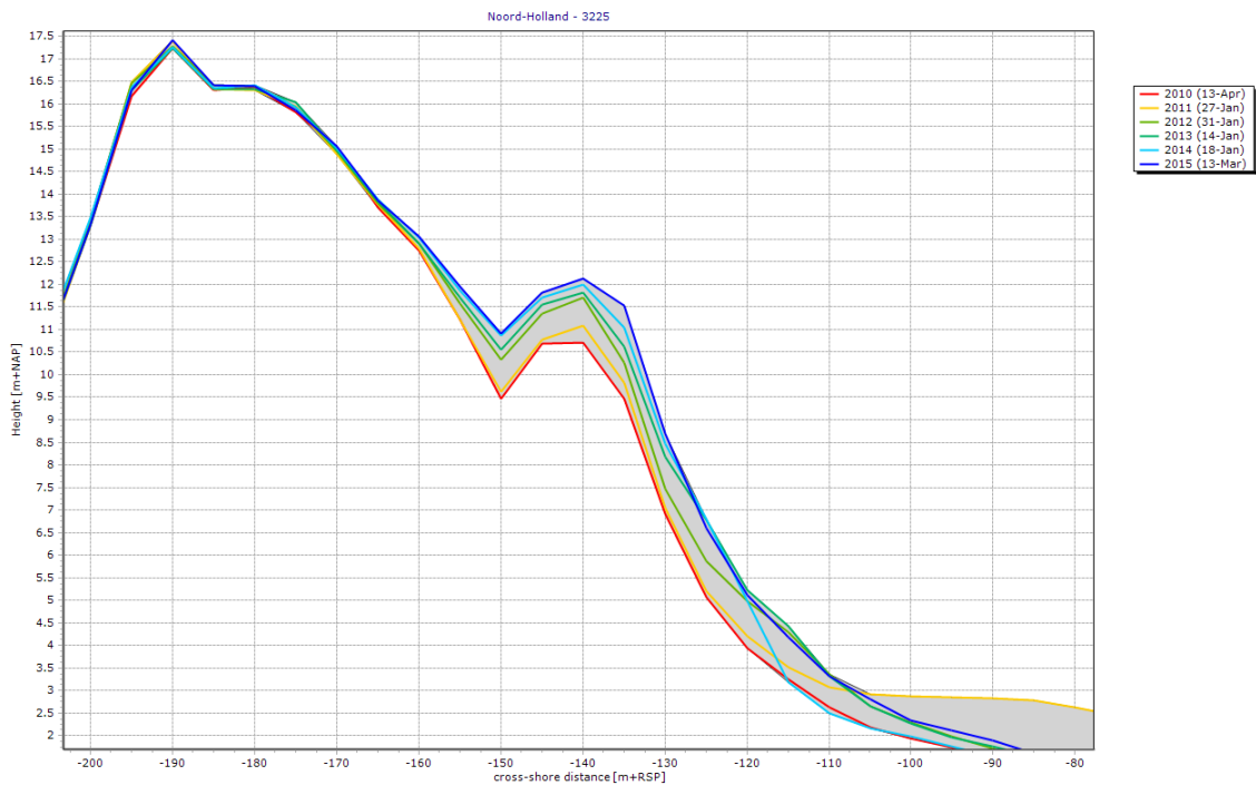
Figure 38: Profile 3225 showing the first dune at the centre of the northern beach nourishment
