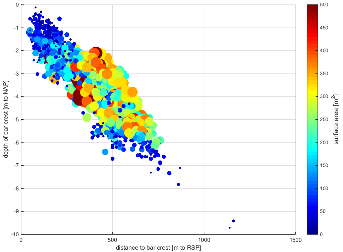
Figure 58: Relation between horizontal distance to bar crest and depth of the bar crest, for each bar in the years before the start of the shoreface nourishments (2000). Colours and circle-size correspond with surface area of the bar (m 2 )
