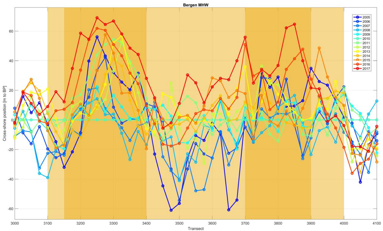
Figure 47: Position of the mean high water line relative to the position in 2010 for the transects in the study area (3000 is in the north, 4100 in the south) from 2005 to 2017. Squares indicate nourishment positions: shoreface nourishment (yellow) and two parts of the beach nourishment (orange).
