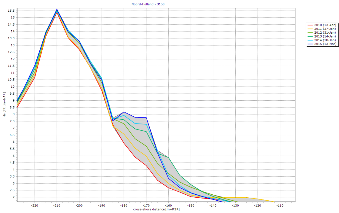
Figure 37: Profile 3150 showing the first dune at the north end of the northern beach nourishment
