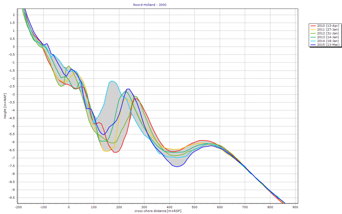
Figure 24: Profile 3000 showing the shoreface just north of the shoreface nourishment
