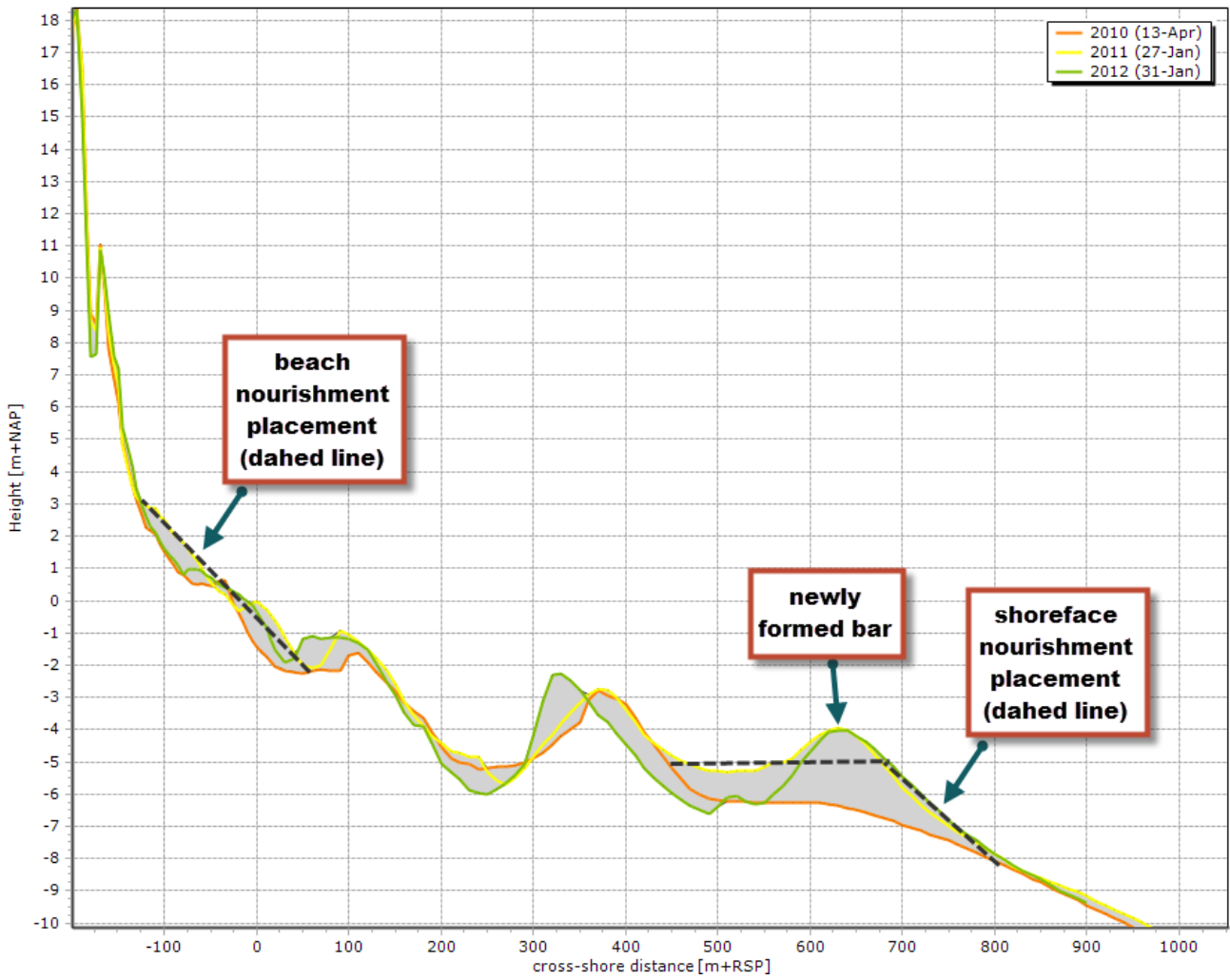
Figure 5: Transect 3200 showing the placement of the beach and shoreface nourishments. The actual placement of the beach nourishment is likely ending around NAP -1 m, not NAP -2 m as seen in this profile due to changes after construction.
