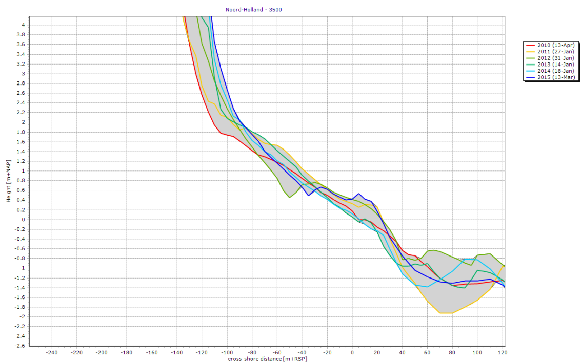
Figure 31: Profile 3500 showing the zone around the beach in between the northern and southern beach nourishments
