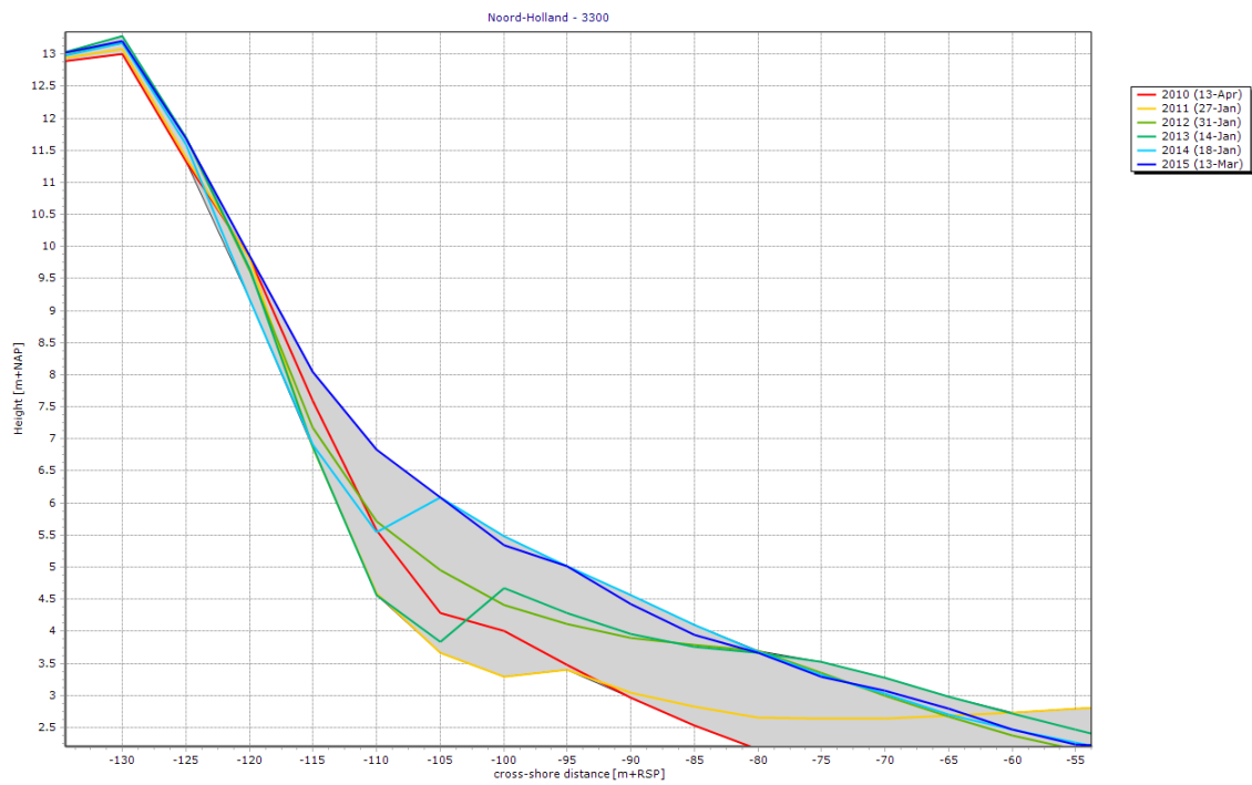
Figure 39: Profile 3300 showing the first dune at the northern beach nourishment
