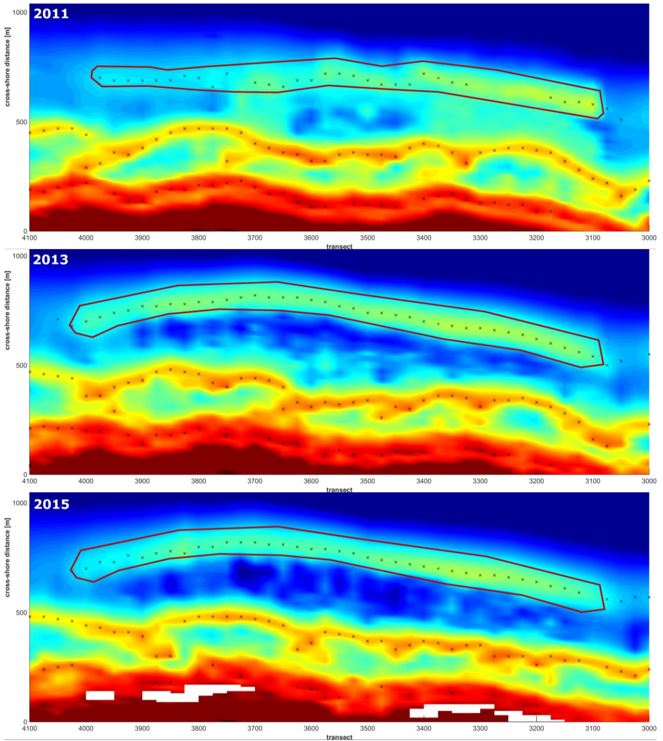
Figure 60: Bathymetry plot based on transect data (not gridded data) measured in 2011, 2013 and 2015 with the detected bar crest position indicated with crosses. The indicated areas show the shoreface nourishments considered in this study of 2010 (top) and 2011 (middle), and their remaining sediment in 2015 (bottom)
