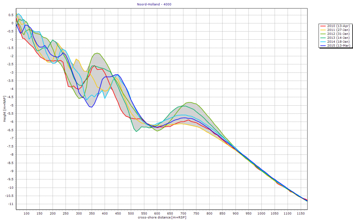
Figure 27: Profile 4000 showing the shoreface just south of the shoreface nourishment
