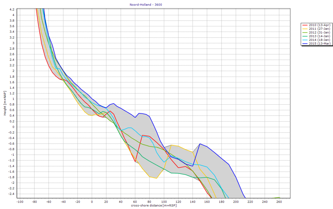
Figure 32: Profile 3600 showing the zone around the beach in between the northern and southern beach nourishments
