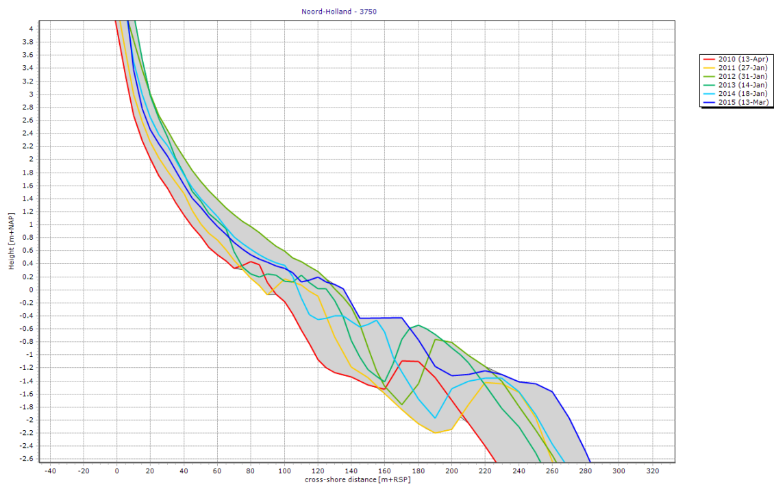
Figure 33: Profile 3750 showing the zone around the beach in at the north end of the southern beach nourishment
