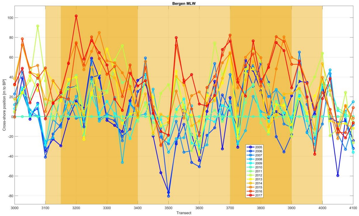
Figure 46: Position of the mean low water line relative to the position in 2010 for the transects in the study area (3000 is in the north, 4100 in the south) from 2005 to 2017. Squares indicate nourishment positions: shoreface nourishment (yellow) and two parts of the beach nourishment (orange).
