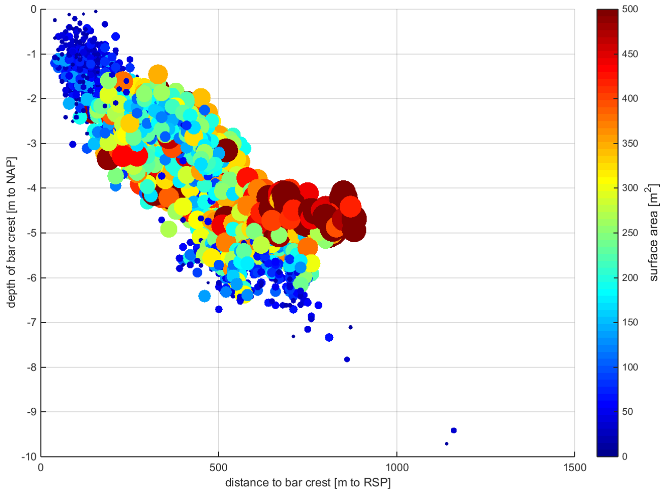
Figure 57: Relation between horizontal distance to bar crest and depth of the bar crest, for each bar in all measured years. Colours and circle-size correspond with surface area of the bar (m 2 )
