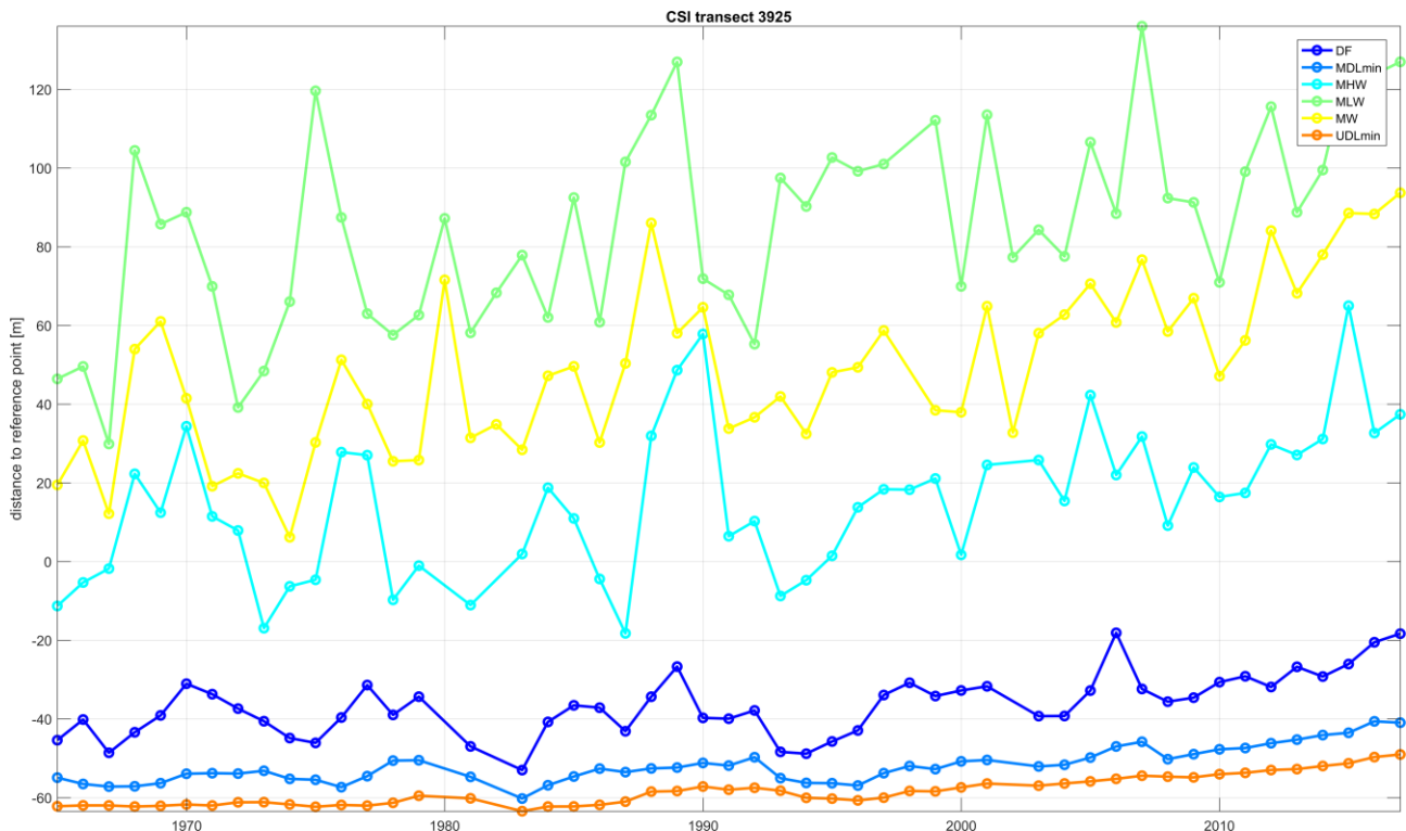
Figure 51: Development of all coastal state indicators in time for transect 3925
