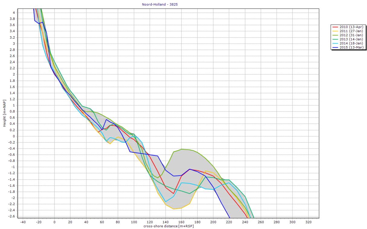
Figure 35: Profile 3825 showing the zone around the beach at the north end of the southern beach nourishment
