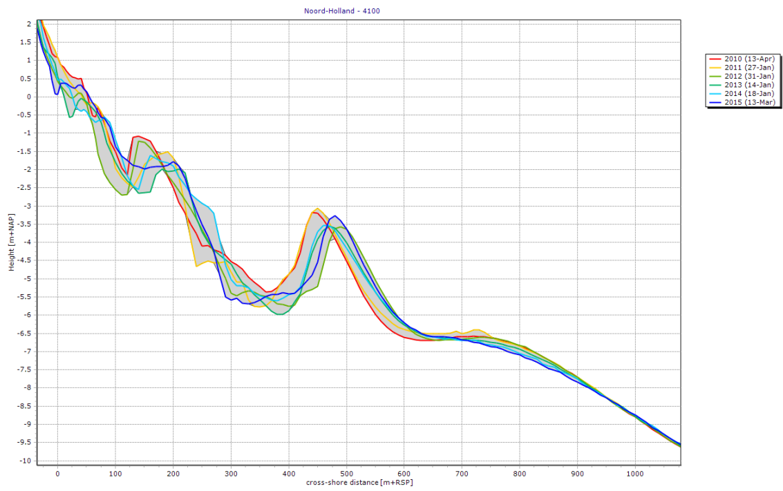
Figure 28: Profile 4100 showing the shoreface 1 km south of the shoreface nourishment
