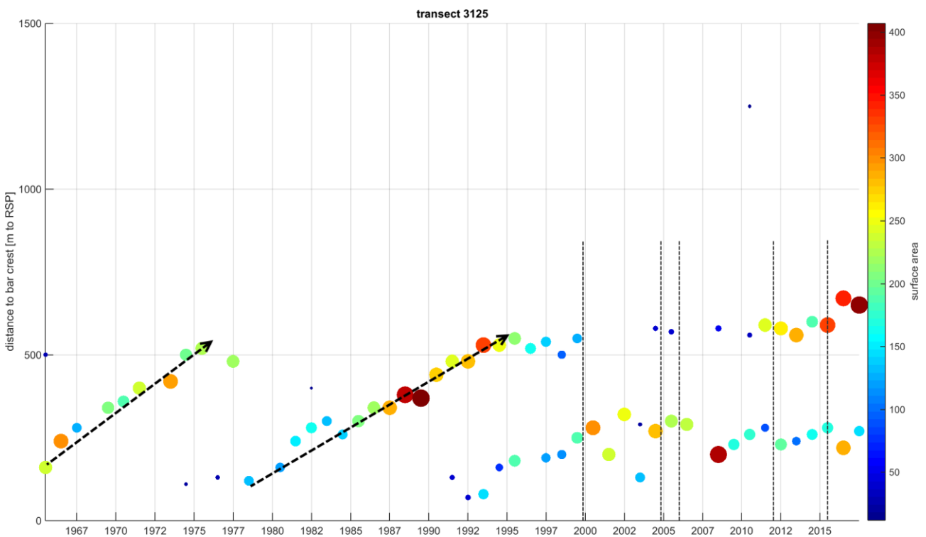
Figure 52: Development of bar crests position over time for transect 3125, colours and circle-size correspond with surface area of the bar (m 2 ), dashed arrows indicate movement of single bar in time, dashed vertical lines indicate shoreface nourishments.
