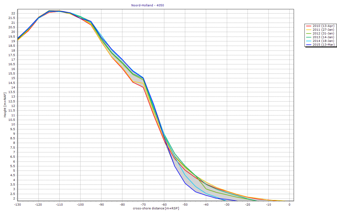
Figure 42: Profile 4050 showing the first dune just south of the southern beach nourishment
