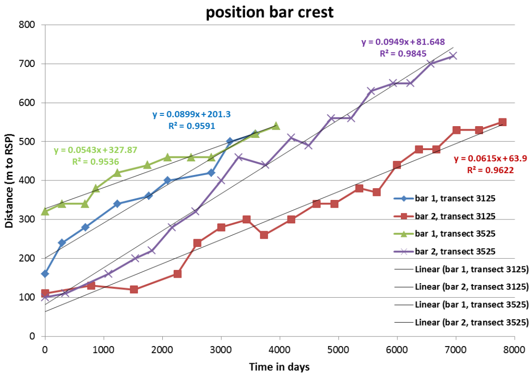
Figure 53: Linear regression analyses on change of bar crest position in time for four randomly chosen bars
