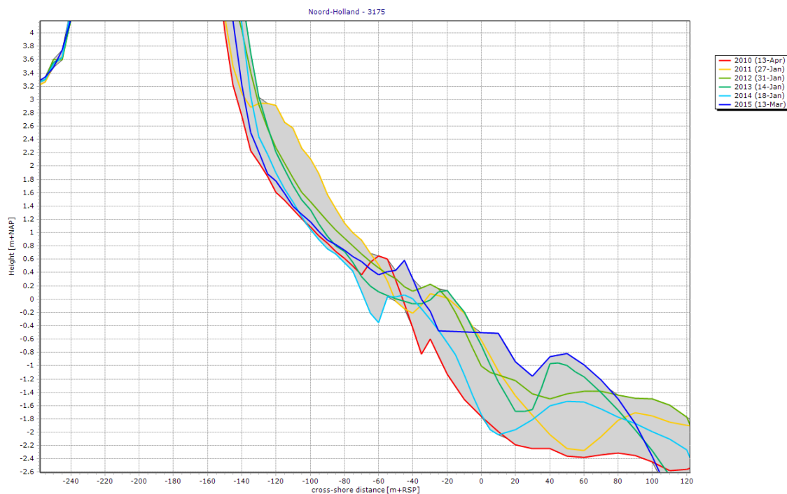
Figure 29: Profile 3175 showing the zone around the beach at the north end of the northern beach nourishment
