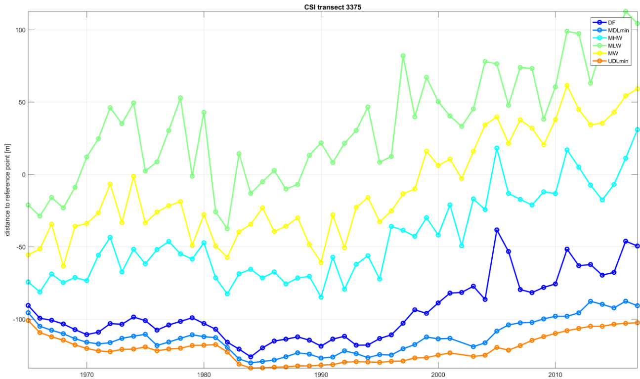
Figure 50: Development of all coastal state indicators in time for transect 3375
