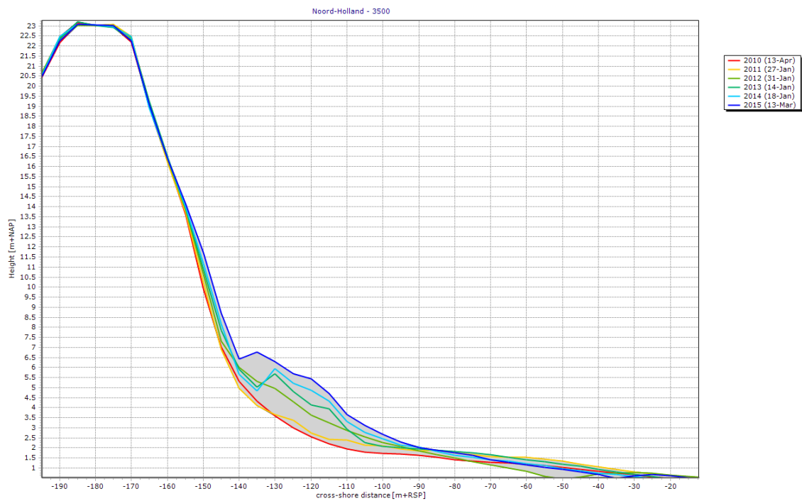
Figure 40: Profile 3500 showing the first dune just in between the northern and southern beach nourishment
