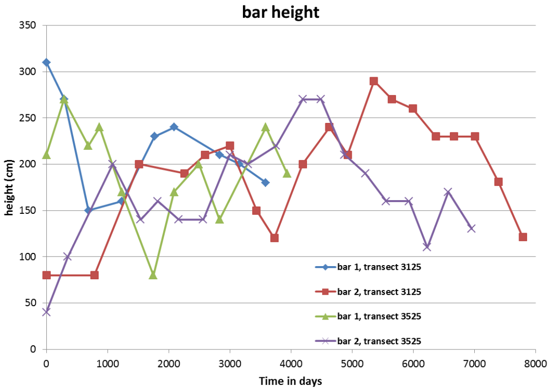
Figure 54: Change of bar height in time for randomly chosen bars
