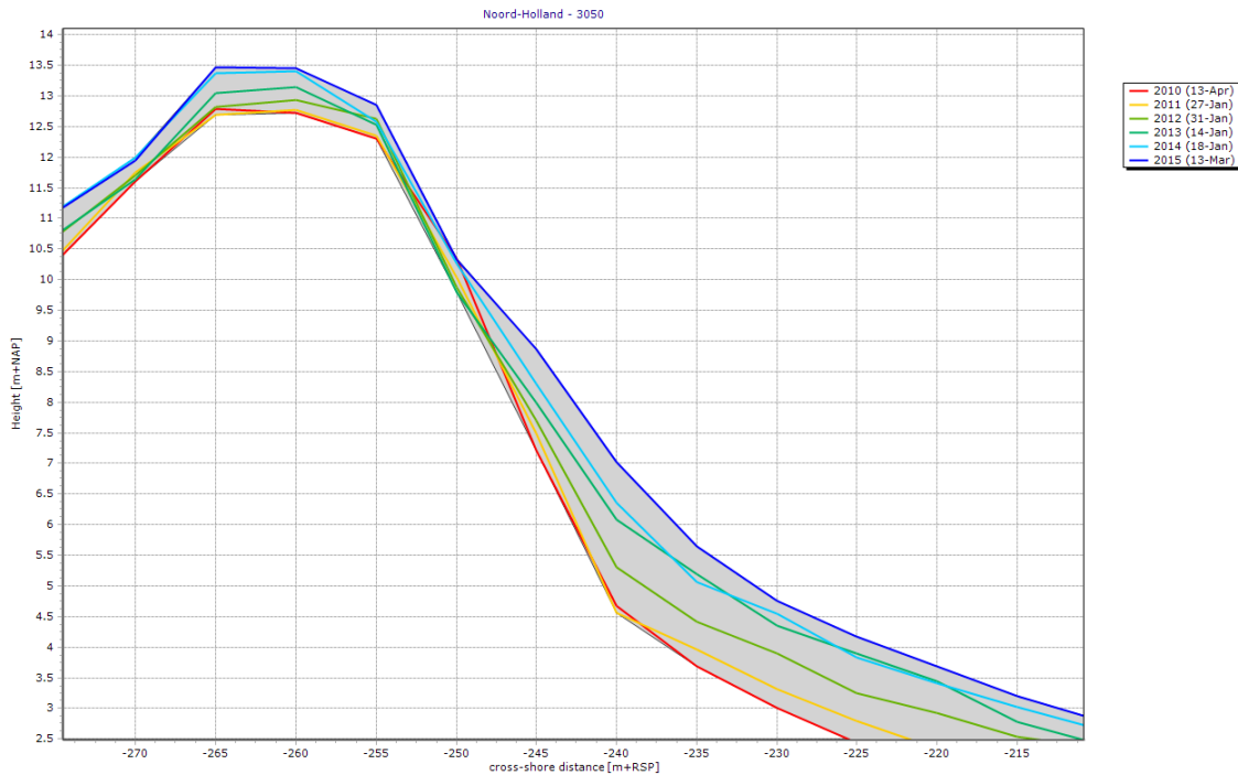
Figure 36: Profile 3050 showing the first dune 1 km north of the northern beach nourishment
