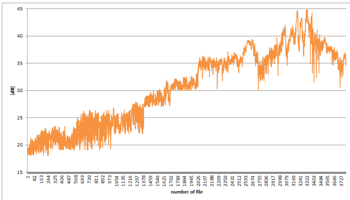
Figure 6-33: Measurements of the 'highest peak/ side peaks' ratio on the Karlskrona-Gdynia route
