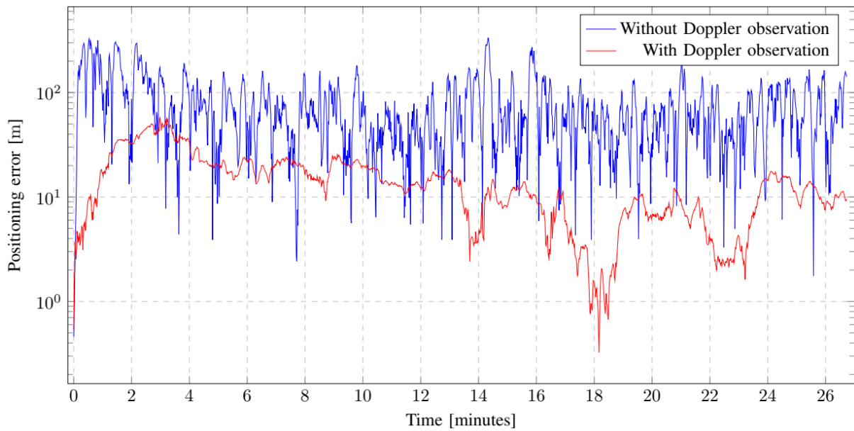
Figure 5-12: Positioning error after Kalman filtering.
