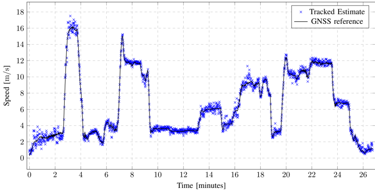
Figure 5-11: Estimated speed and reference speed obtained by GNSS.
