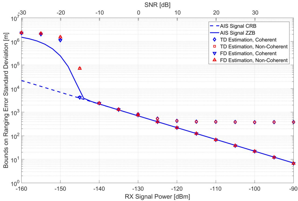
Figure 3-1: R-Mode ranging performance bounds and simulation results using a 1-slot ranging signal in 1 AIS Channel. The ranging signal is a GMSK modulated random 256-bit sequence.
