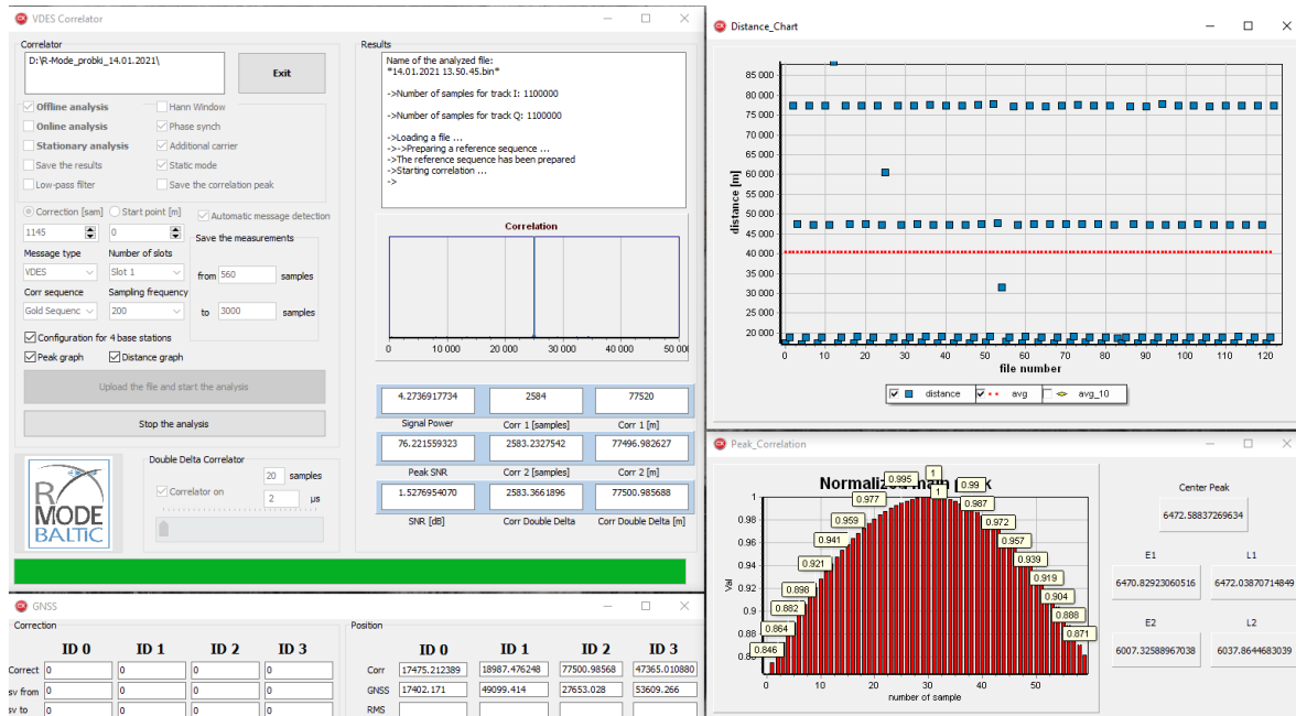
Figure 6-60: Signal correlation application - scenario for four stations
