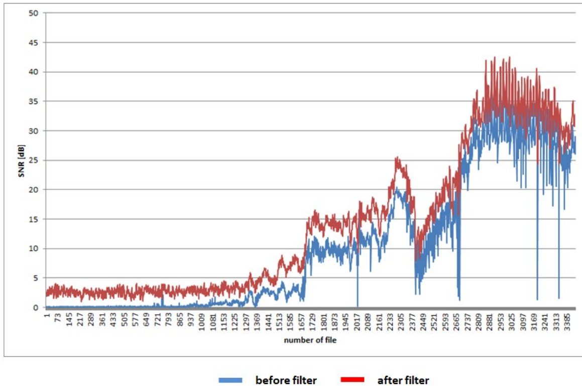
Figure 6-32: Measured SNR on the Karlskrona-Gdynia route
