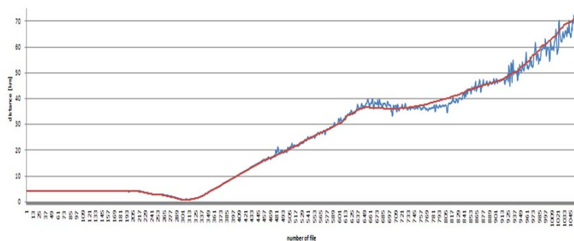
Figure 6-17: Superimposed results from the correlator and GNSS + EGNOS receiver for the AIS measurement campaign on the Gdynia-Karlskrona route
