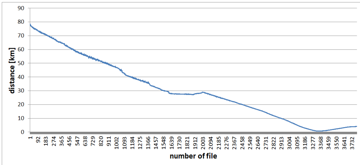
Figure 6-28: Distance measurements from the application for the correlation of signals on the Karlskrona-Gdynia route
