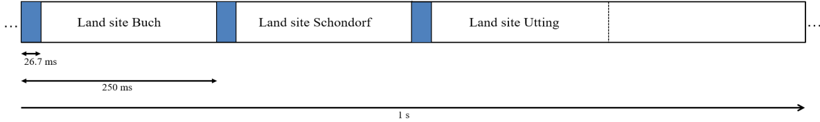
Figure 5-7: Time scheduling of the different land transmitters. The blue colored area represents the ranging sequence of length T_{\text{seq}} = 26.67\text{ms} or one VDES time slot.
