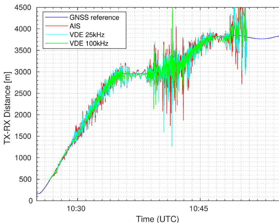
Figure 5-4: Ranging performance plotted over time.
