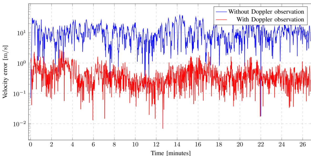
Figure 5-14: Absolute error of the estimated velocity after Kalman tracking.
