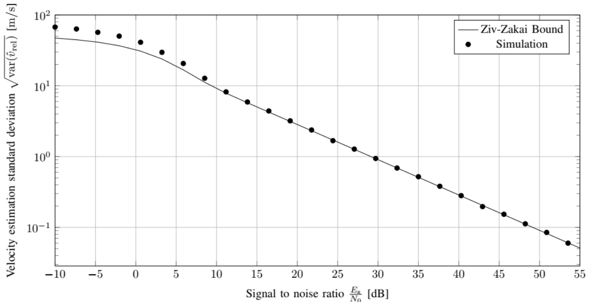
Figure 2-2: Ziv-Zakai Bound for Doppler based velocity estimation.
