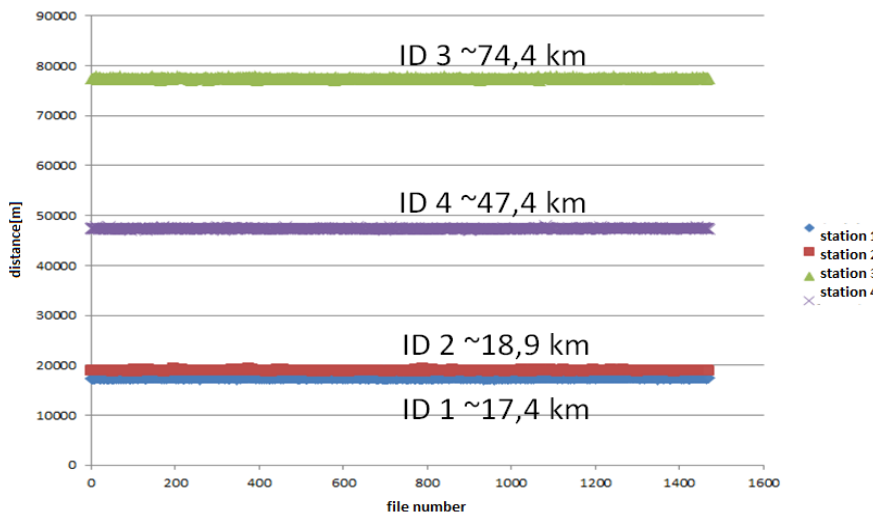
Figure 6-61: Designated distances for four base stations
