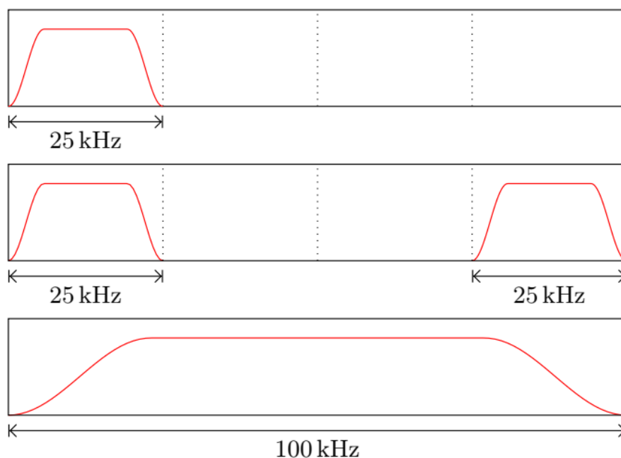
Figure 3-10: Different options for utilizing the available bandwidth. Schematically showing the power spectral density of average VDES link signals.
