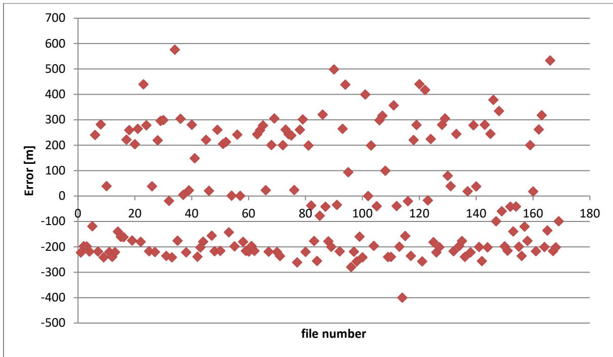
Figure 6-51: Measurement results for 1 MHz sampling frequency
