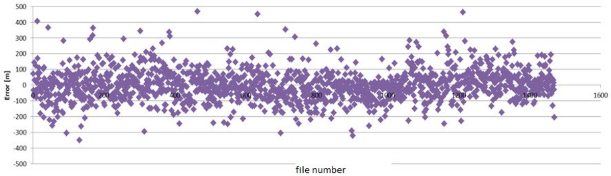
Figure 6-67: Calculated accuracy for the fourth station
