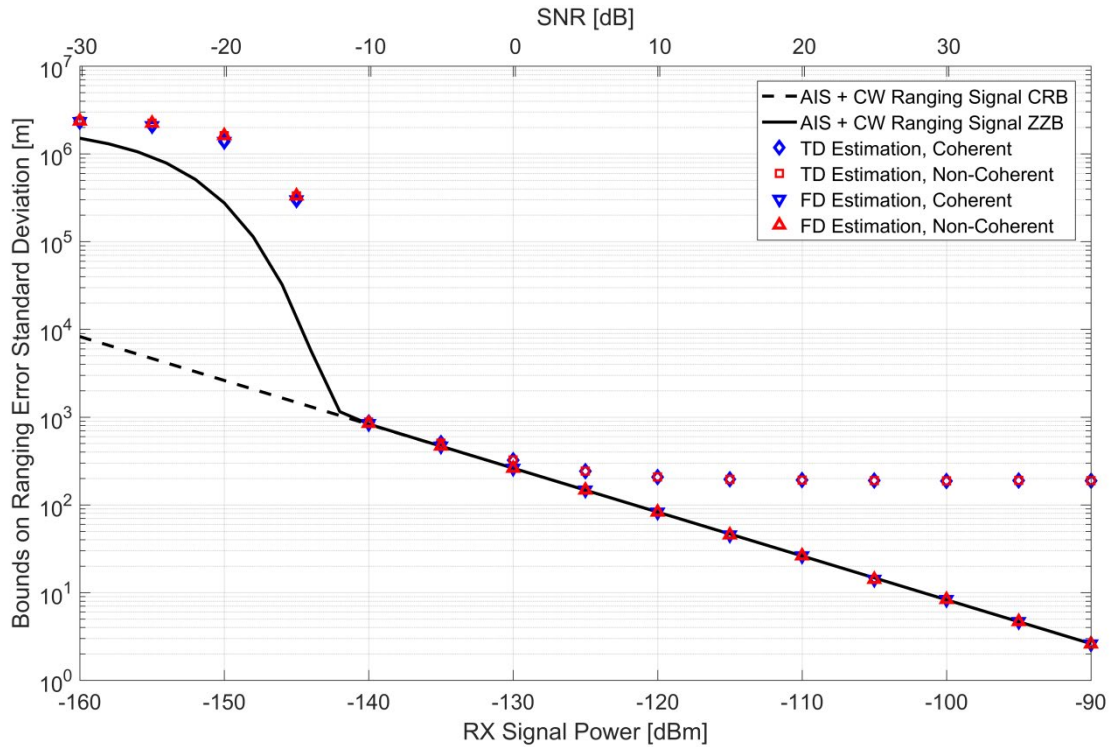
Figure 3-7: R-Mode ranging performance bounds and simulation results using a 1-slot ranging signal in 1 AIS Channel. The ranging signal consists of a GMSK modulated random bit sequence and a Tukey windowed CW signal, transmitted with equal power.
