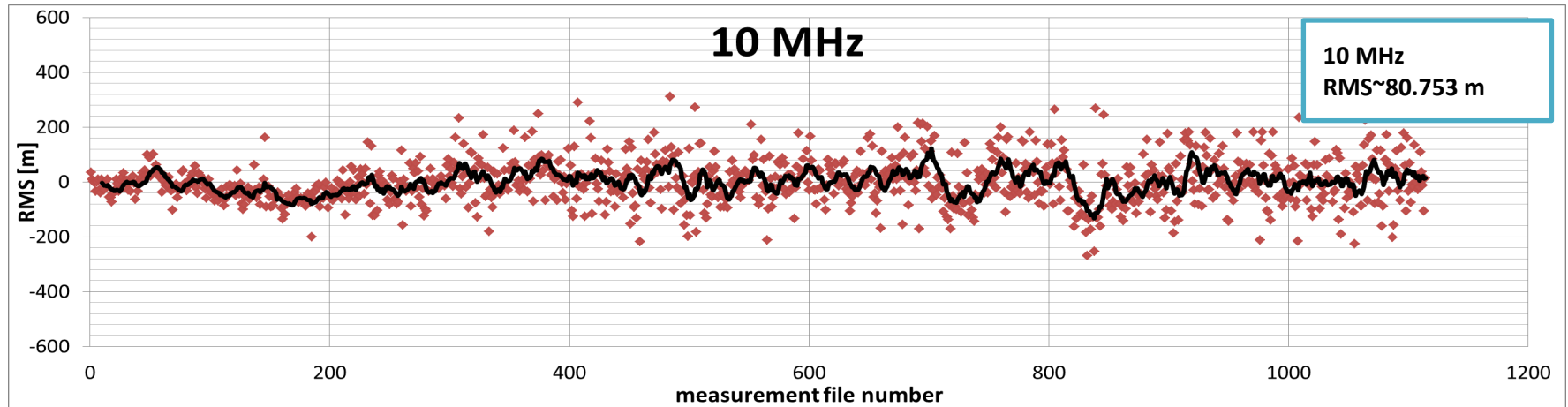
Figure 6-53: Results for a sampling frequency of 10 MHz
