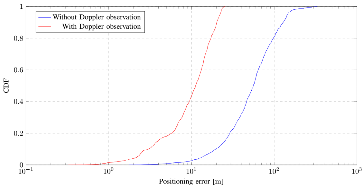
Figure 5-13: Positioning error CDF under line of sight conditions.
