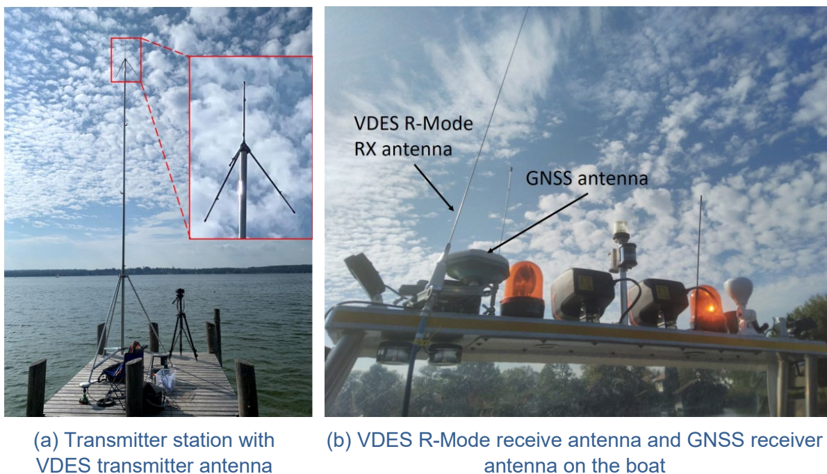
Figure 5-6: Transmitter and receiver setup at Lake Ammer.
