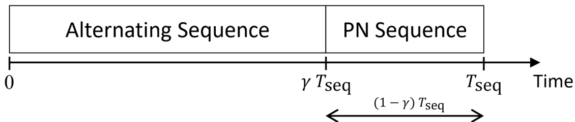
Figure 4-5: The ranging sequence is split into two parts consisting of an alternating sequence part and a Gold code (pseudo-noise (PN)) sequence part. The ratio of both sequence parts in a VDES time slot of T_{seq} = 26.67 ms is determined by the ranging sequence ratio \gamma \in [0; 1] .
