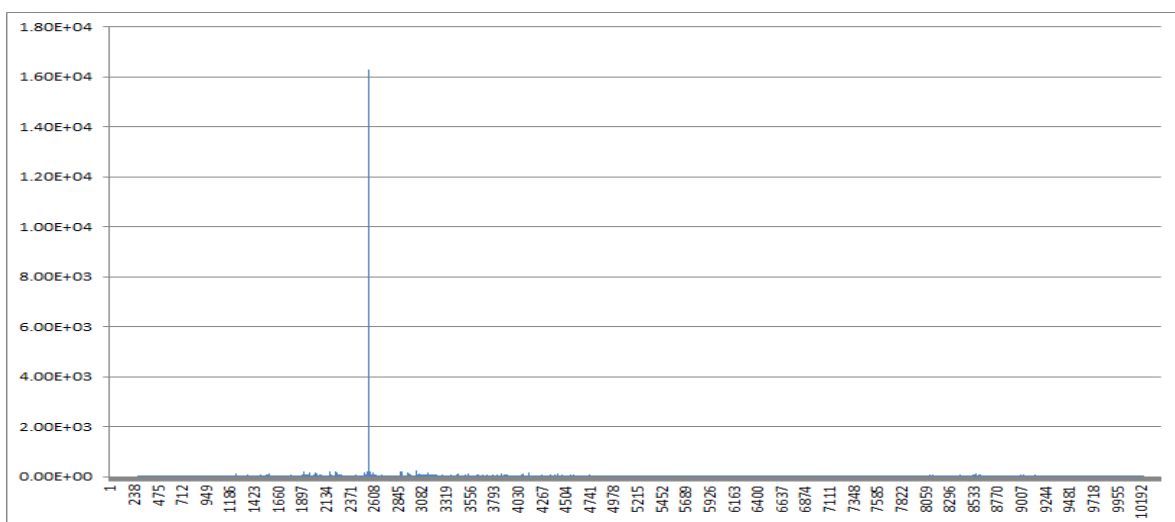
Figure 6-69: Correlation of parts of the Gold sequence
