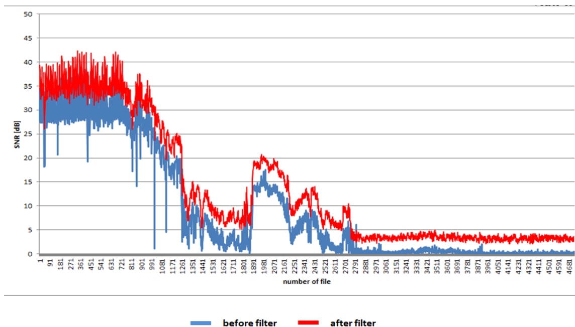
Figure 6-18: Measured SNR on the Gdynia-Karlskrona route
