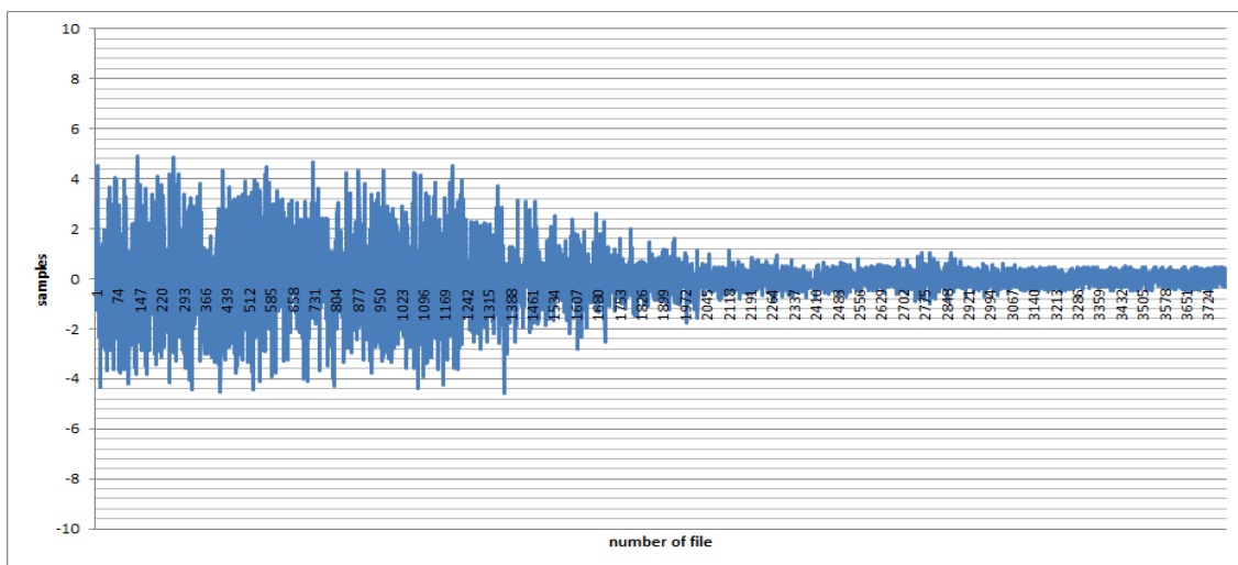
Figure 6-35: Effectiveness of using multicorrelation - Double-delta d1=d2=10
