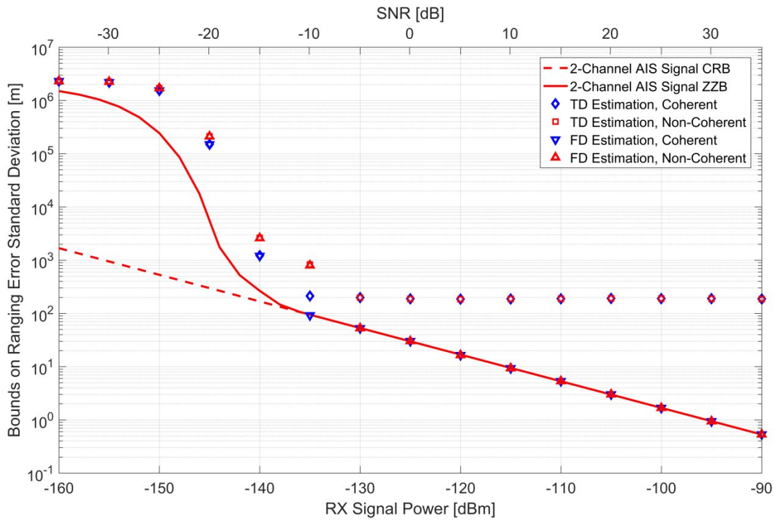
Figure 3-9: R-Mode ranging performance bounds and simulation results using a 1-slot GMSK ranging signal covering 2 AIS Channels coherently.
