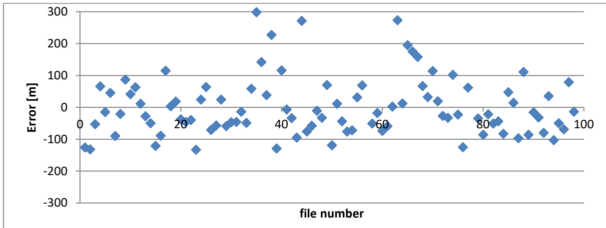
Figure 6-45: Measurement results for 200 MHz sampling frequency
