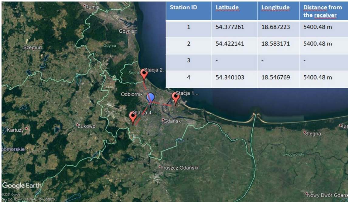
Figure 7-12: The fifth measurement scenario for testing the R-Mode positioning system demonstrator in real time
