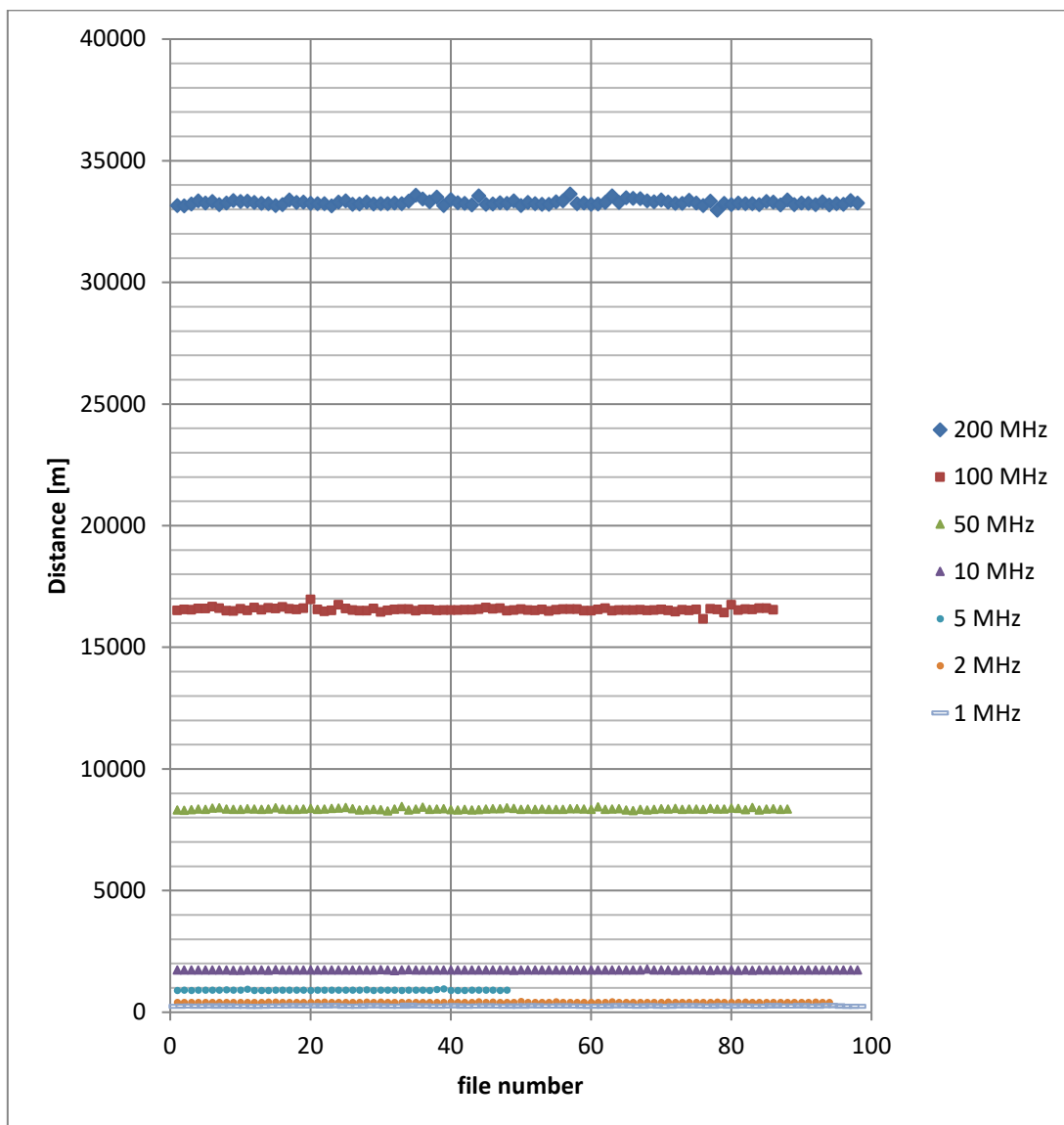
Figure 6-44: Analysis of the calculated distance accuracy depending on the sampling frequency
