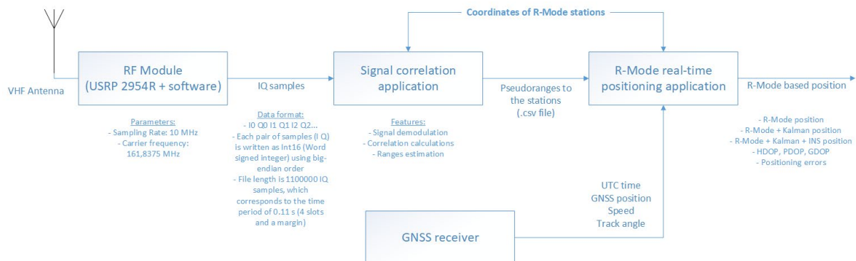
Figure 7-1: A diagram of the R-Mode system implementation
