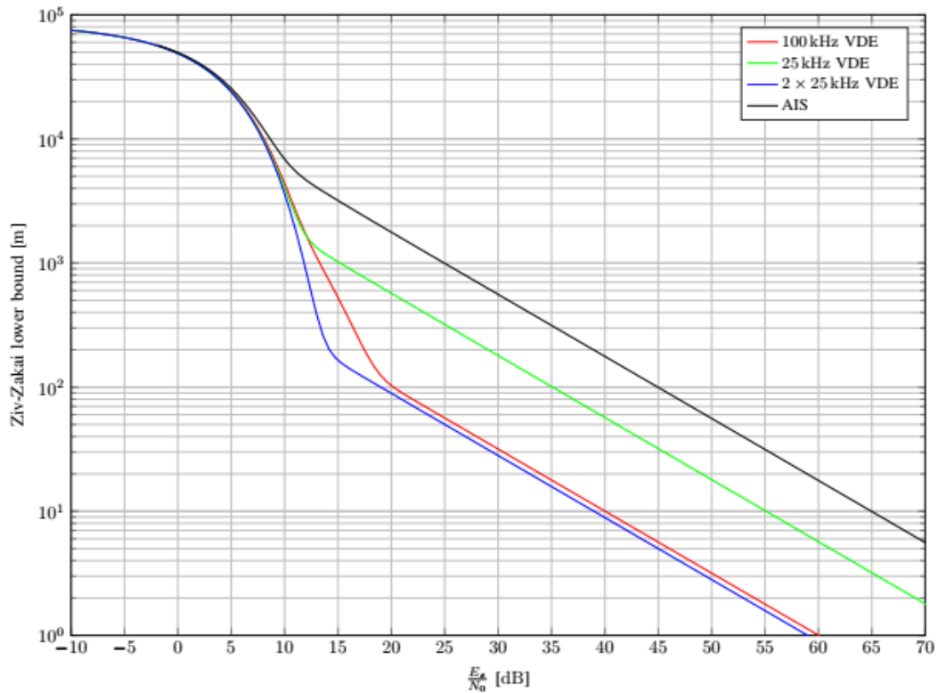
Figure 3-11: Lower bounds on the time of arrival estimation error.
