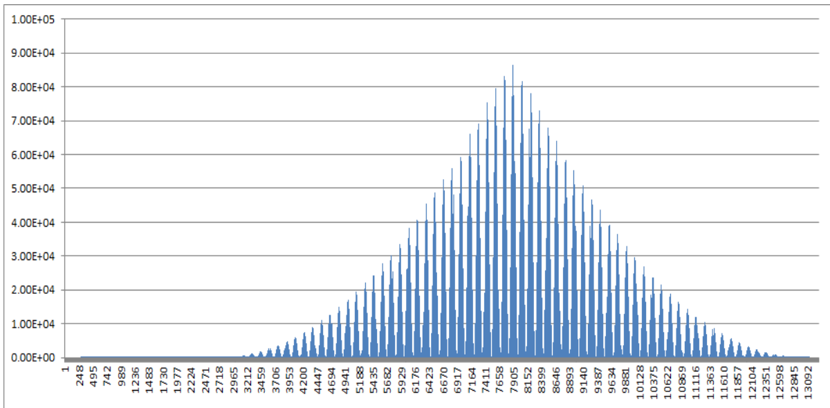
Figure 6-70: Correlation part of the string alternative sequence
