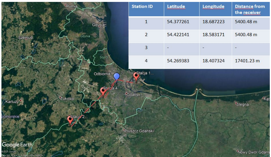
Figure 7-13: The sixth measurement scenario for testing the R-Mode positioning system demonstrator in real time
