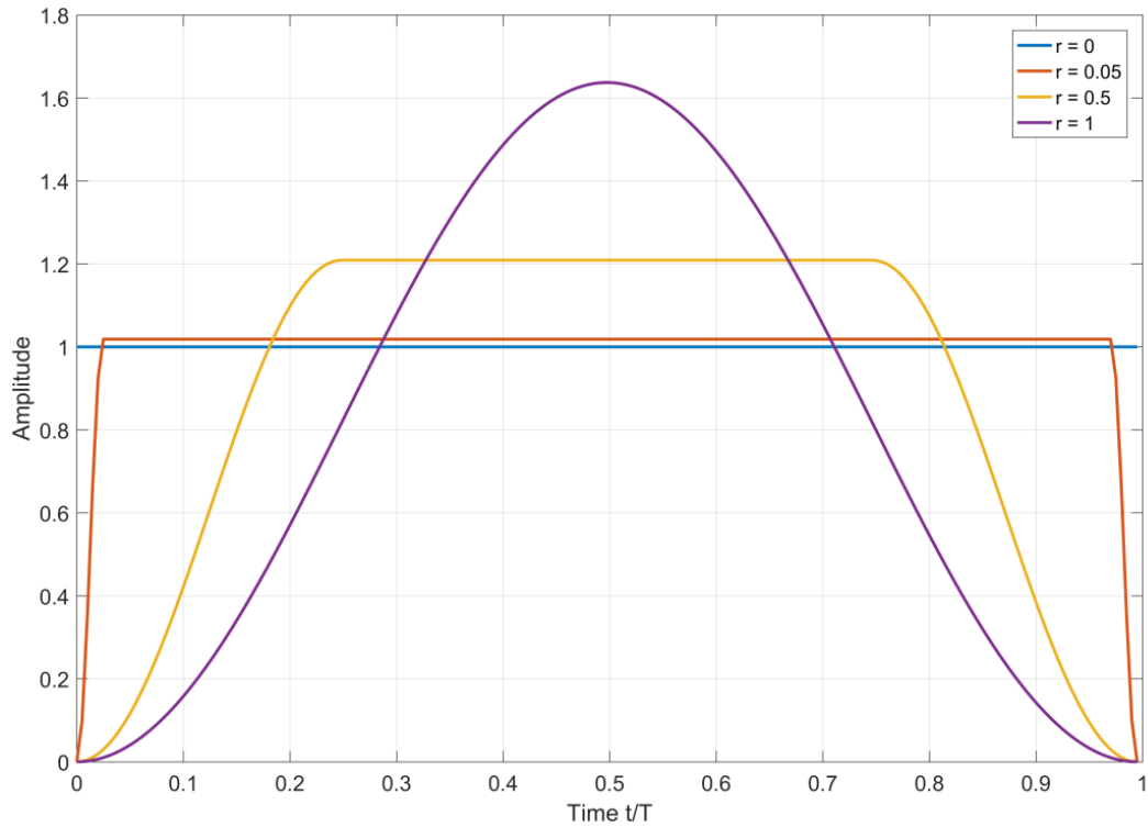
Figure 3-3: Tukey window for different roll-off values r .
