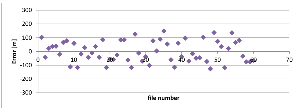
Figure 6-50: Measurement results for 2 MHz sampling frequency
