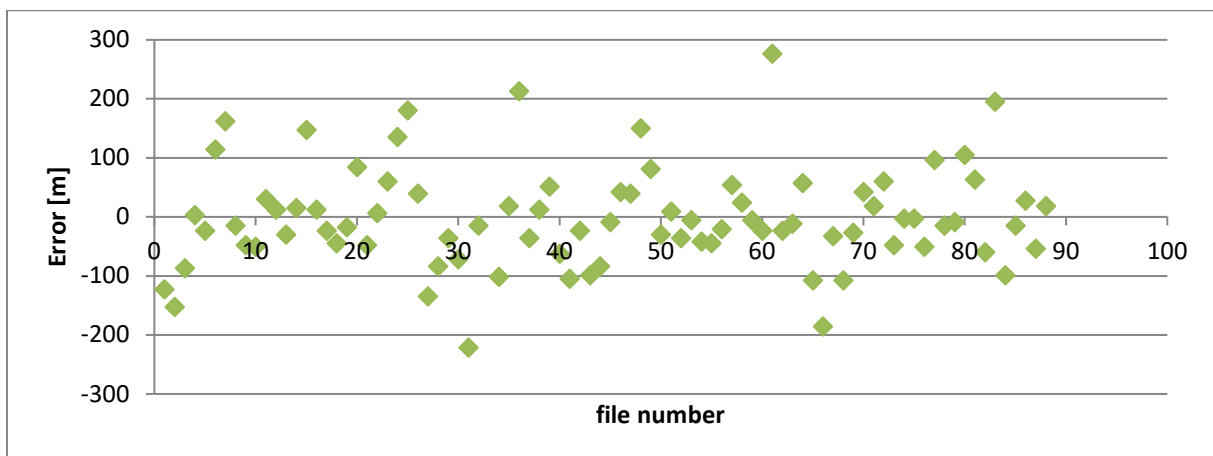
Figure 6-47: Measurement results for 50 MHz sampling frequency
