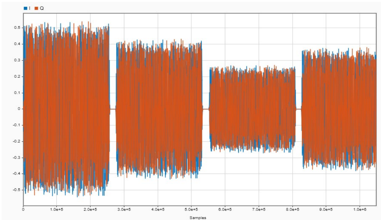
Figure 6-57: A four-slot message
