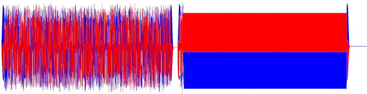
Figure 6-55: VDES signal transmitted in two time slots. In the first slot, the Gold sequence is transmitted, in the second slot the alternating sequence is transmitted.
