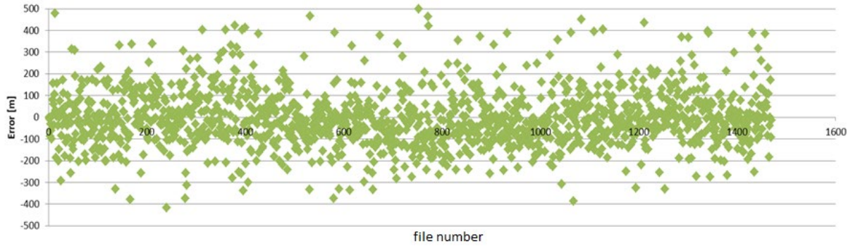
Figure 6-66: Calculated accuracy for the third station
