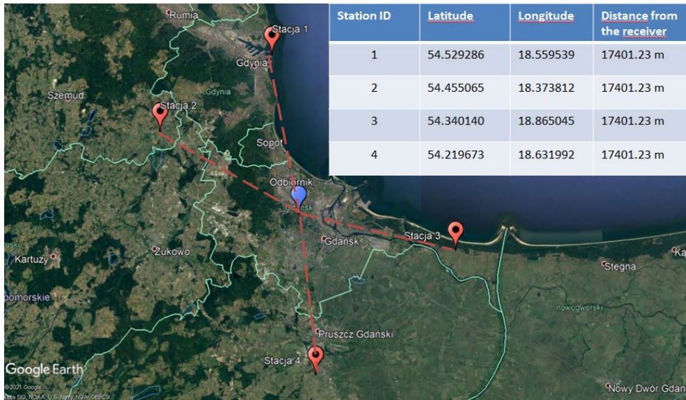
Figure 7-8: The first measurement scenario for testing the positioning R-Mode demonstrator in real time
