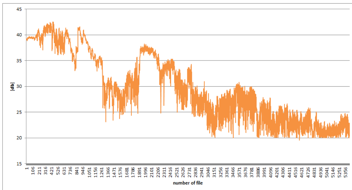
Figure 6-19: Measurements of the 'highest peak/ side peaks' ratio at the Gdynia – Karlskrona route
