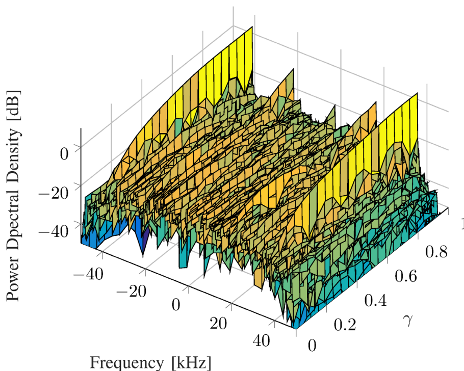
Figure 4-6: Power spectral density of the signal for different values of \gamma .
