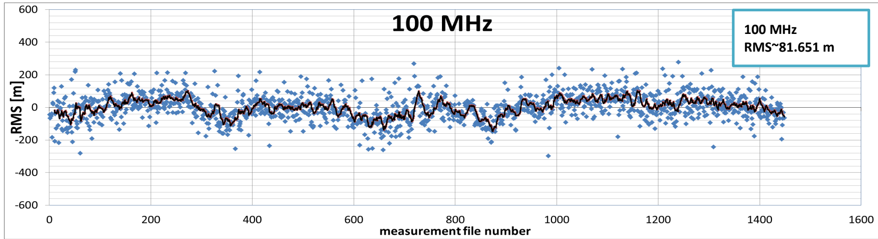
Figure 6-52: Results for a sampling frequency of 100 MHz
