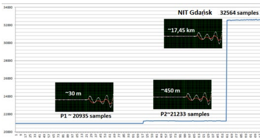
Figure 6-1: Processed calibration files
