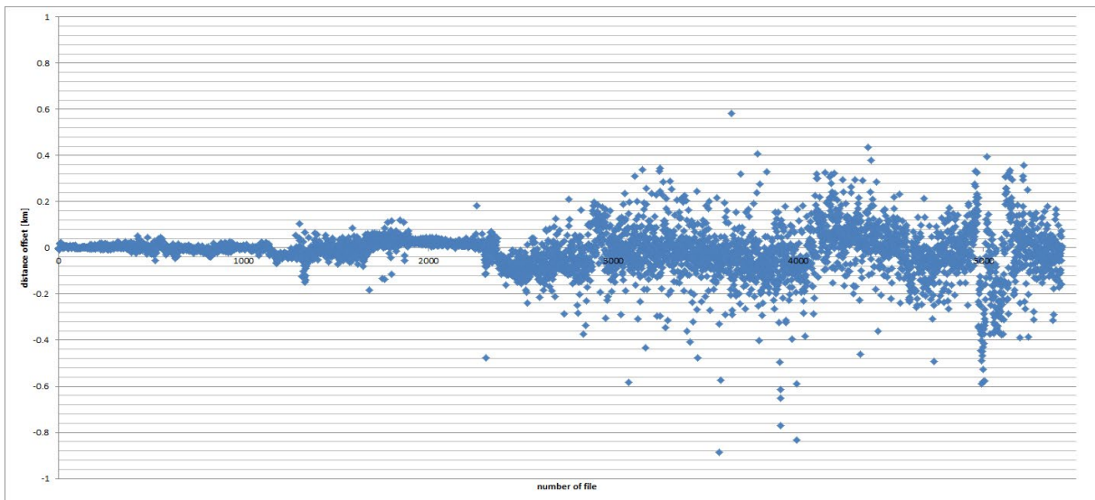
Figure 6-26: Distance error accuracy at the Gdynia – Karlskrona route
