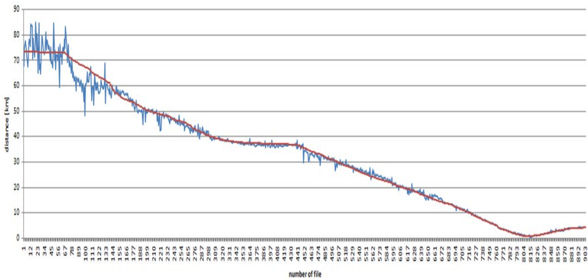
Figure 6-31: Distance measurements from the GNSS + EGNOS receiver on the AIS measurement campaign on the Gdynia-Karlskrona route
