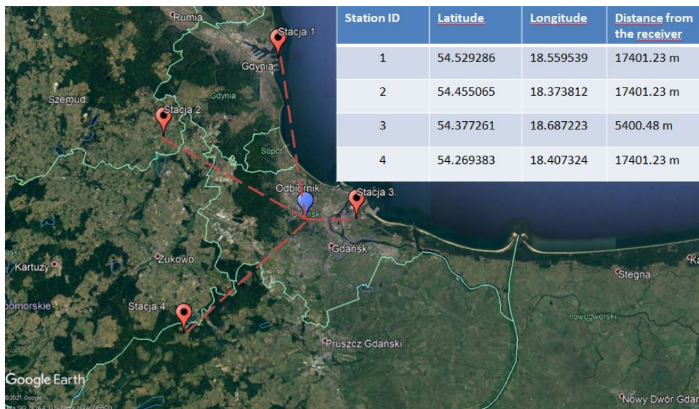
Figure 7-9: The second measurement scenario for testing the positioning R-Mode demonstrator in real time
