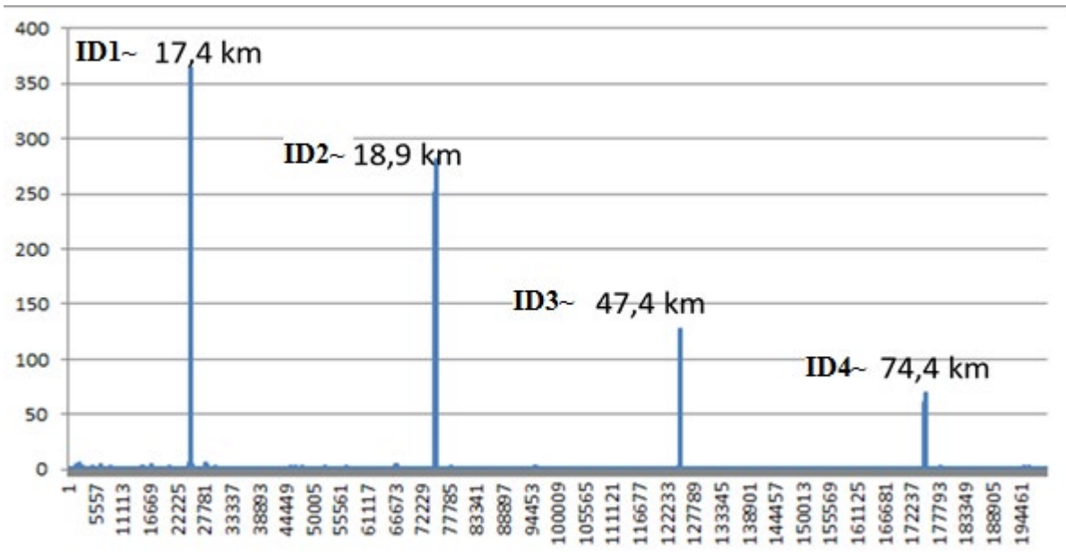
Figure 6-62: Correlation peaks for each of the slots
