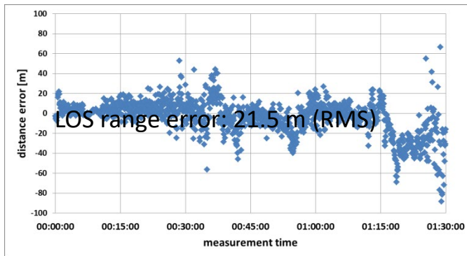
Figure 6-39: Obtained measurement results – ranging accuracy
