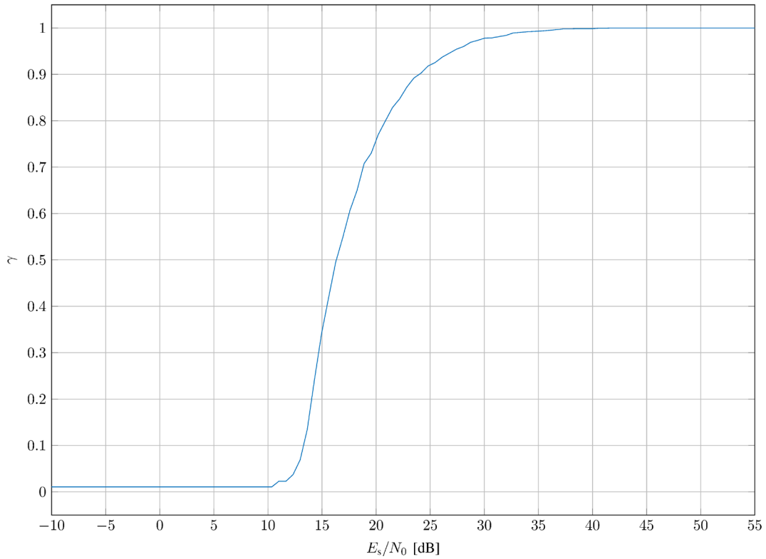
Figure 4-9: Optimal values of ranging sequence ratio \gamma for a given E_s/N_0
