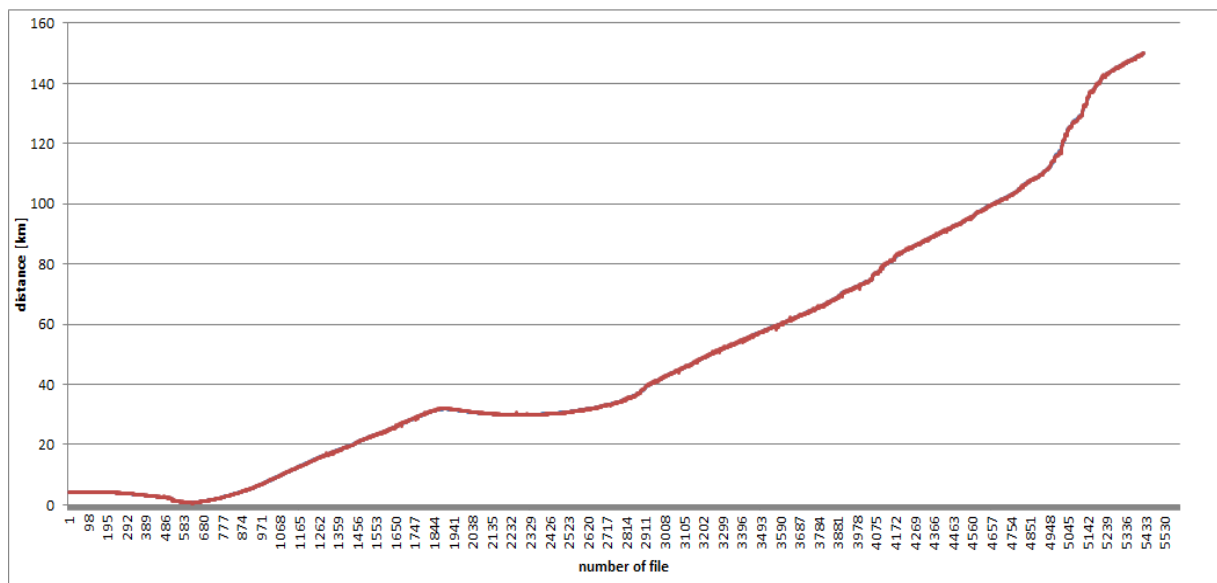
Figure 6-16: Superimposed results from the correlator and GNSS + EGNOS receiver for the VDES measurement campaign on the Gdynia-Karlskrona route
