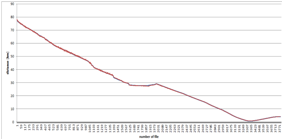
Figure 6-30: Superimposed results from the correlator and GNSS + EGNOS receiver for the VDES measurement campaign on the Karlskrona-Gdynia route
