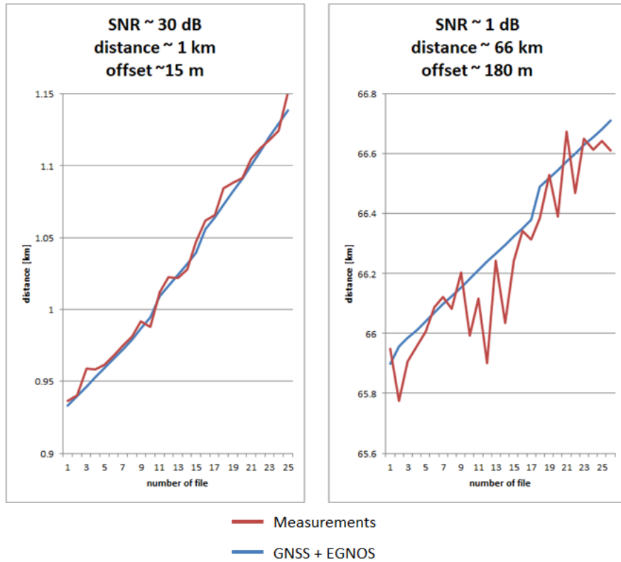
Figure 6-25: Accuracy obtained on measurements at the Gdynia – Karlskrona route
