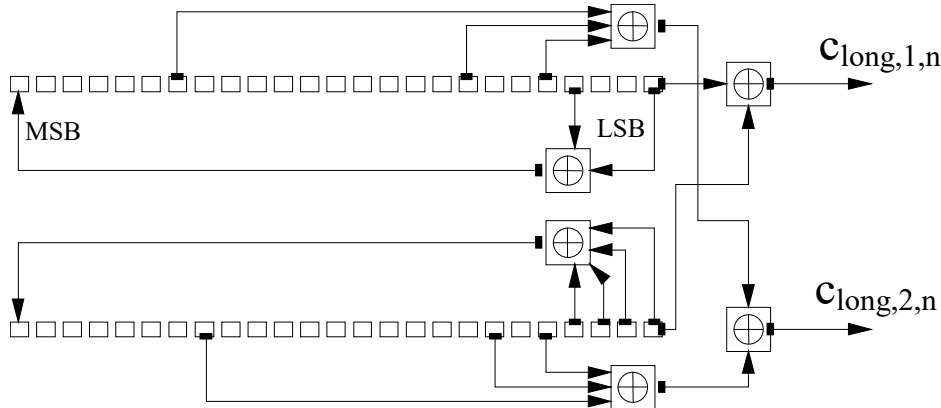
Figure 4-2: Configuration of the UMTS uplink scrambling sequence generator [UMTS]
