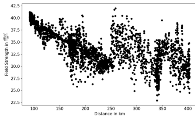
Figure 9. Field strength over distance for the Swedish transmitter station Holmsjö.
