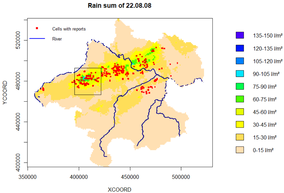
Figure 6: Spatial distribution of precipitation (daily rain sum) at the 22.08.08
