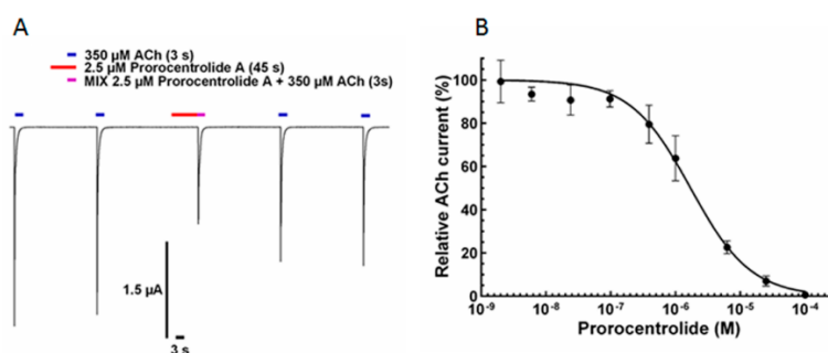
Figure 2. Effect of prorocentrolide-A on the human \alpha 7 nAChR expressed in Xenopus oocytes. (A) Typical inward nicotinic currents evoked by ACh (350 \mu M) applied for 3 s and recorded at -60 mV holding membrane potential. The blue tracings above the current traces denote the perfusion of ACh. The red tracing (above the current trace) denotes the perfusion of 2.5 \mu M prorocentrolide-A. Note that no current was evoked by the perfusion of the prorocentrolide alone, which indicates that it has no direct agonist action on the \alpha 7 -receptor, while when applied together with ACh (red and blue tracing, MIX, 3rd current trace from left) a block of the peak inward current was observed. The washout of the prorocentrolide from the medium by the fast perfusion system allowed a partial recovery of the ACh evoked current (4th and 5th current tracings) as compared to the control currents (first two tracings). (B) Concentration-dependent inhibition of ACh-elicited nicotinic currents by prorocentrolide-A in oocytes expressing the human \alpha 7 nAChR. Peak amplitudes of ACh-evoked currents (mean \pm SEM), recorded at -60 mV in the presence of the prorocentrolide were normalized to control currents, and fitted to the Hill equation ( nH = 0.93 ). The concentration of ACh used was the EC_{50} determined.
