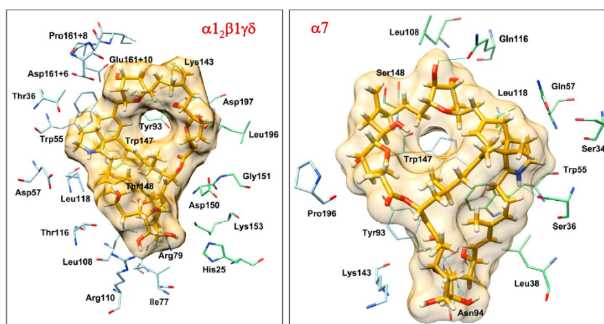
Figure 4. Docking conformations of prorocentrolide-A at the subunit interface of muscle-type (left) and neuronal \alpha_7 nAChR (right). Residues within 4 Å from the ligand are shown. Loop C is hidden for more clarity.
