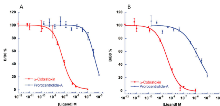
Figure 3. Prorocentrolide-A and \alpha -cobratoxin displaced, in a concentration-dependent manner, the specific [ 125 I] \alpha -BTX binding to HEK-293 cells, expressing the chimeric chick neuronal \alpha 7 -5HT 3 nAChR (A) and to Torpedo membranes expressing the muscle-type \alpha 1_2\beta 1\gamma\delta nAChR; and (B) each point in the curves represents the mean \pm SEM of three different experiments performed in duplicate.
