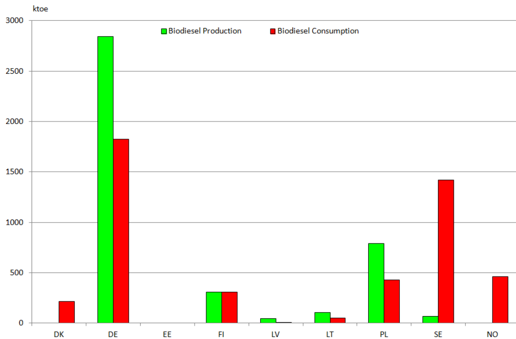
Fig. 45. Primary biodiesel production and final energy consumption in the transport sector in the BSR countries in 2017
