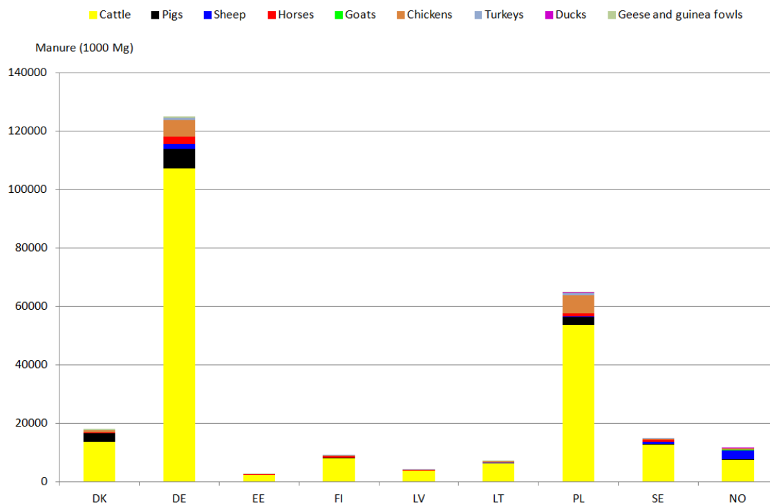
Fig. 16. Theoretical manure potential in the BSR countries in 2017 (1000 Mg/year)
