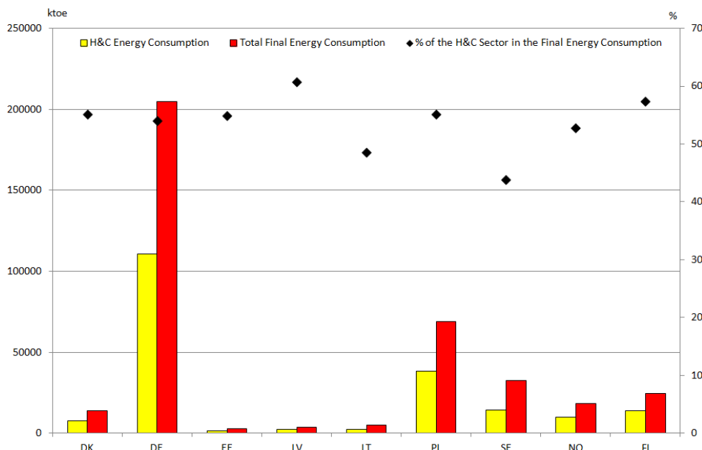
Fig. 35. Heating and cooling consumption compared with total final energy consumption in the BSR countries in 2017
