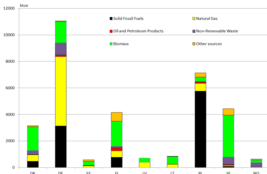
Fig. 36. Gross production of derived heat by type of fuels in the BSR countries in 2017 Source: Bioenergy Europe, 2019d.
