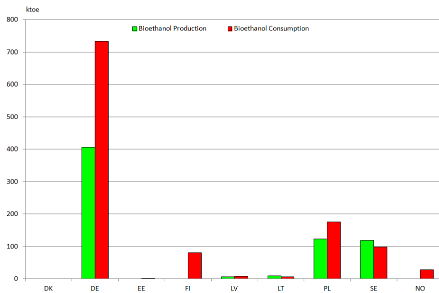
Fig. 44. Primary bioethanol production and final energy consumption in the transport sector in the BSR countries in 2017
