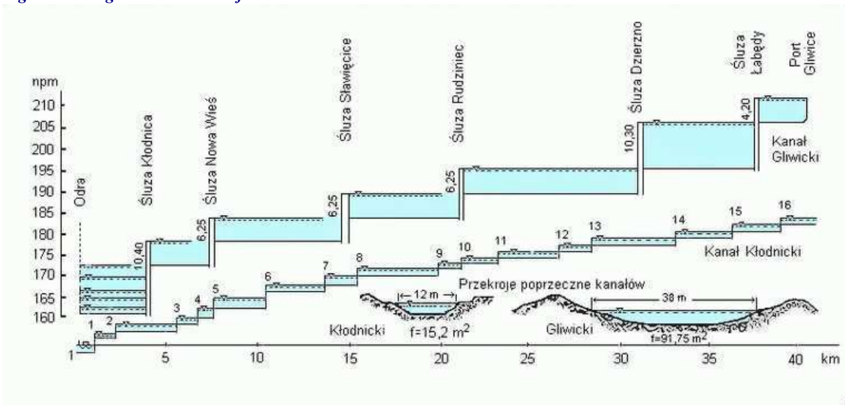
Figure 6 _Longitudinal section of Channel Gliwicki locks
