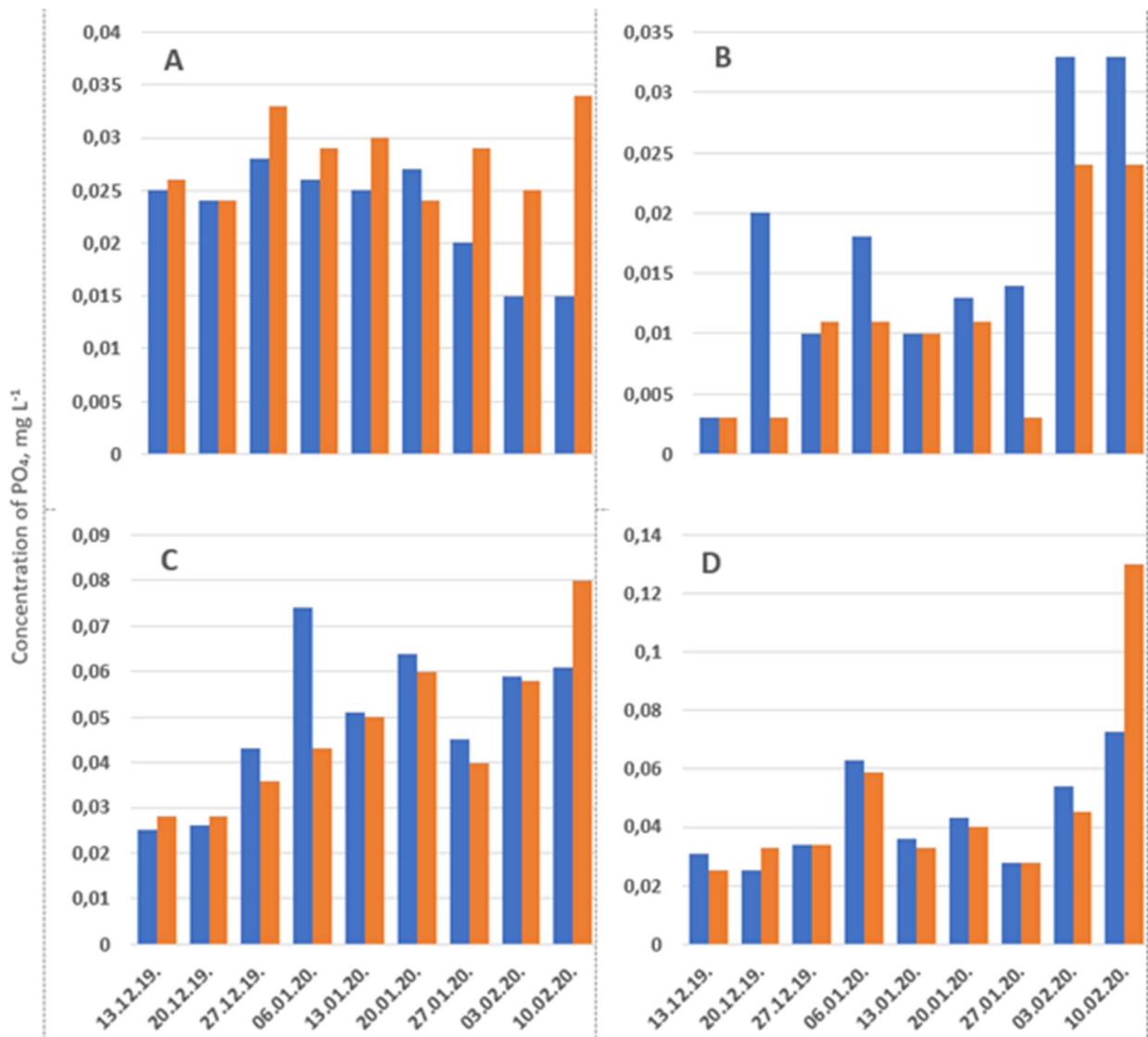
Figure 17. Changes in PO_4 concentration. Blue - PO_4 concentration in water before entering the filter construction, orange - PO_4 in water after discharge of the filter structure. A - Filter # 1, B - Filter # 2, C - Filter # 3, D - Filter # 4.
