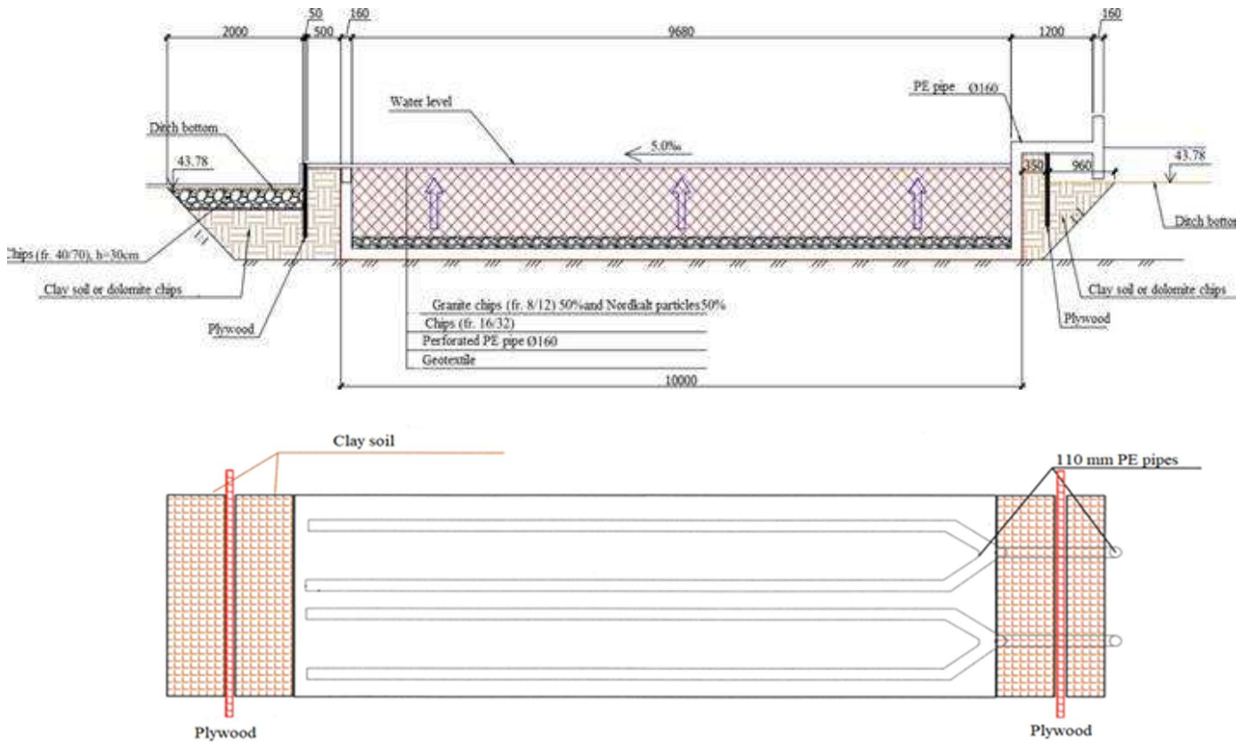
Figure 15. Schematic representation of phosphorus filter. Top - side view, bottom - top view.
