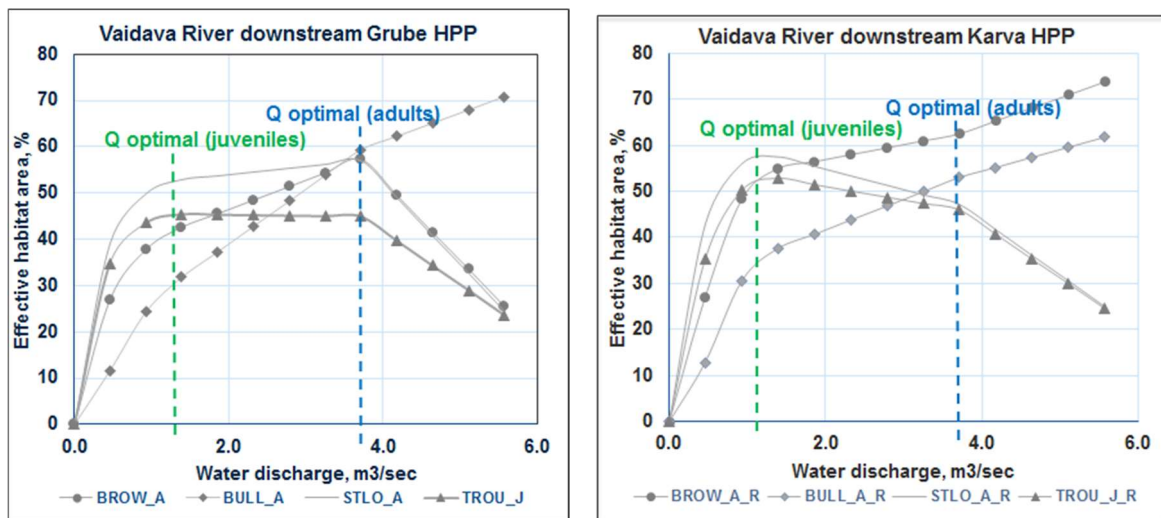
Figure 13. Habitat-Flow rating curves of Vaidava River downstream HPPs (green arrow shows the optimal water discharge for juveniles and blue arrow – for adults).
