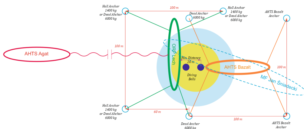
Fig. 7. A variant of common anchorage for the AHTS 'Bazalt' and ORP 'Lech' [own work]
