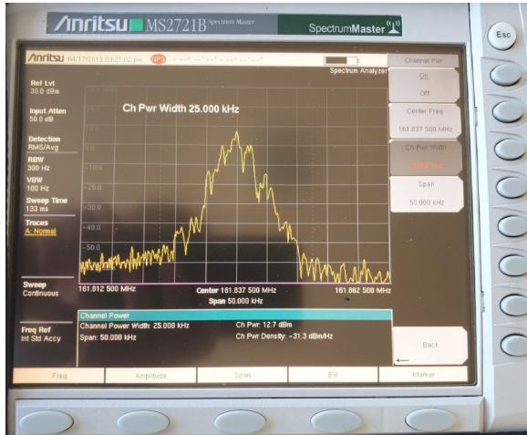
Figure 2-15: Channel power measurements
