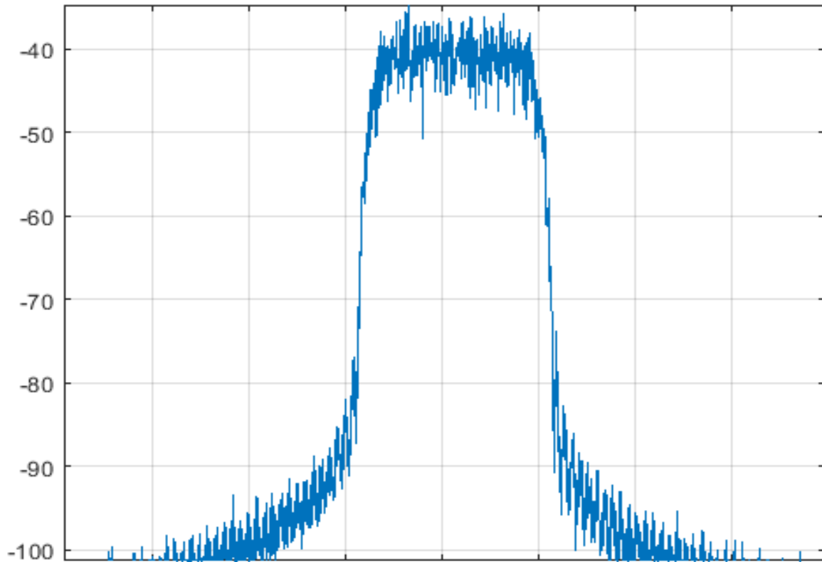
Figure 2-12: Spectrum of the VDES signal
