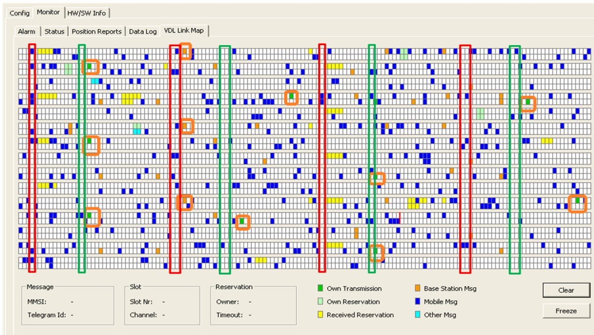
Figure 3-5: The occupancy of AIS slots registered in the Bay of Gdańsk area
