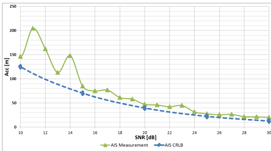
Figure 4-14: RMS curves for water path
