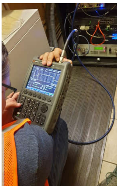
Figure 5-4: Photo from calibration c)
