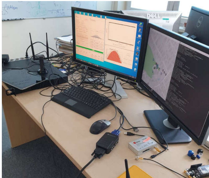
Figure 7-15: R-Mode demonstration stand c)
