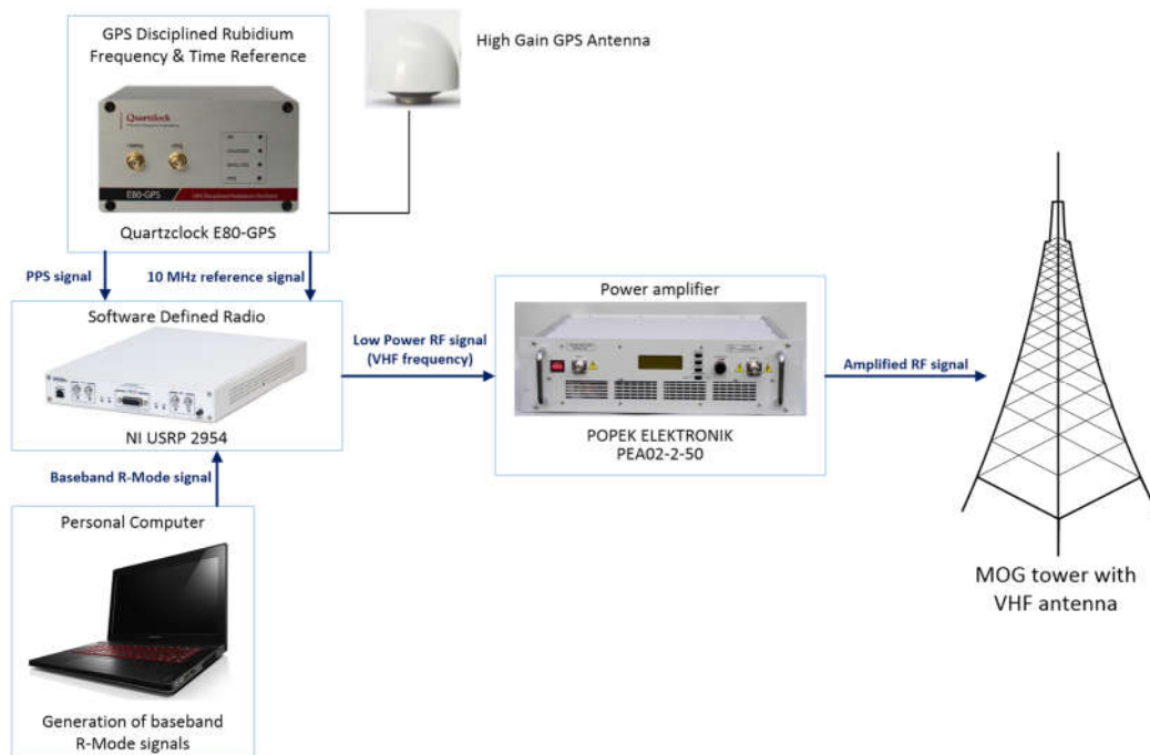
Figure 4-2: Test-bed transmitter diagram for the VDES transmission
