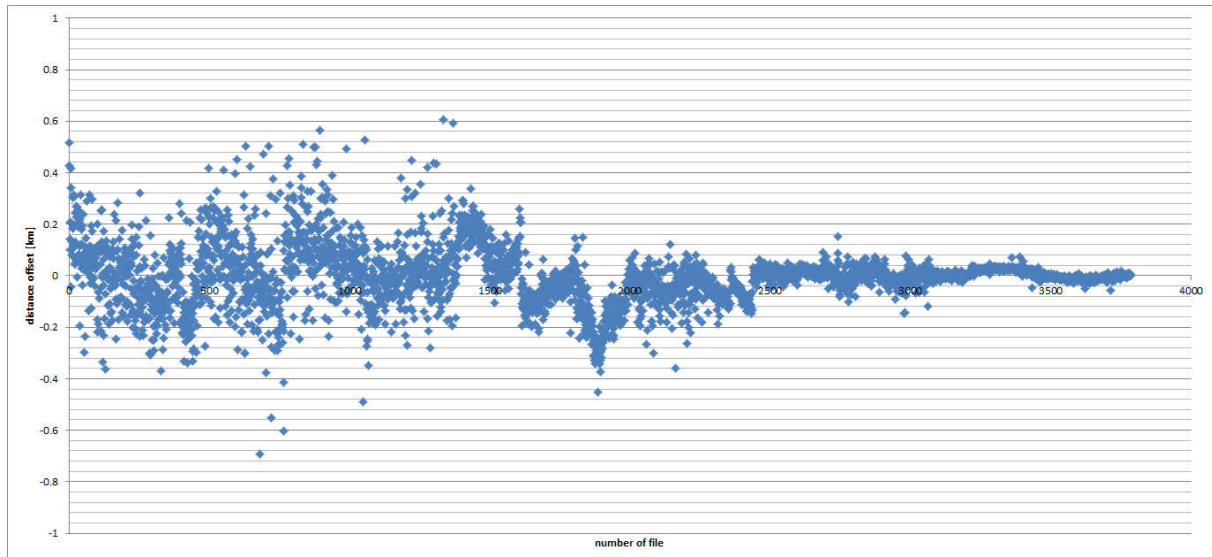
Figure 5-38: Distance error accuracy on the Gdynia – Karlskrona route
