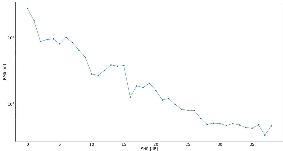
Figure 4-16: Dependence of the RMS value of the position estimation error on the value of the measured SNR of the R-Mode station.
