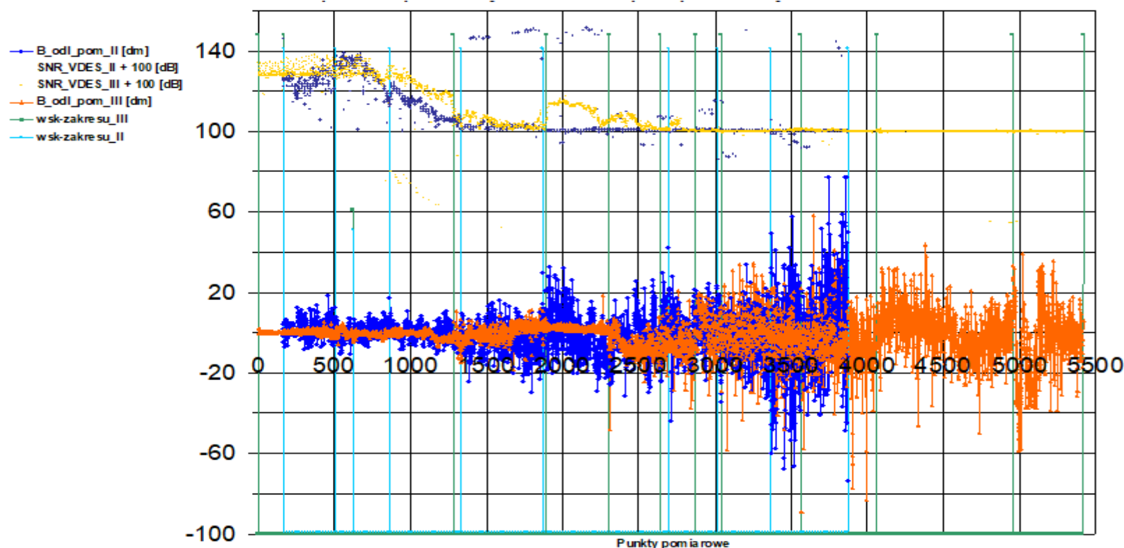
Figure 11: Measurement data (distance measurement error and SNR_VDES value) and range limits as a function of measurement points in the 2nd and 3rd measurement campaigns
