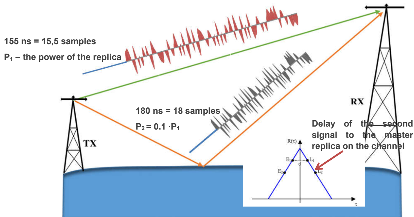
Figure 3-5: The second scenario: the signal replica is delayed with respect to the signal by such a time that the distorted peak of the correlation function is between the first and second pair of double delta correlator samples
