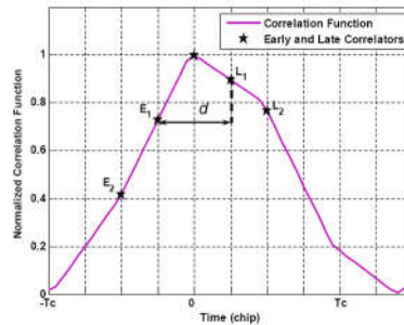
Figure 2-2: The correlation function under multipath conditions
