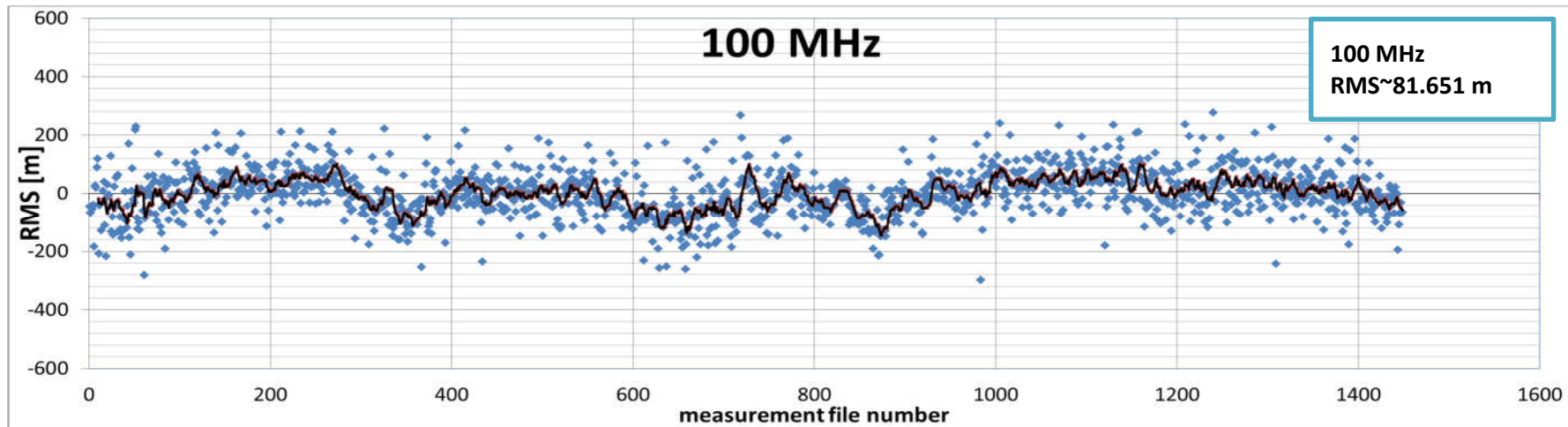
Figure 6-9: Results for a sampling frequency of 100 MHz
