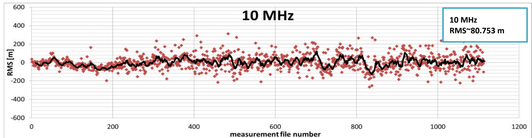
Figure 6-10: Results for a sampling frequency of 10 MHz
