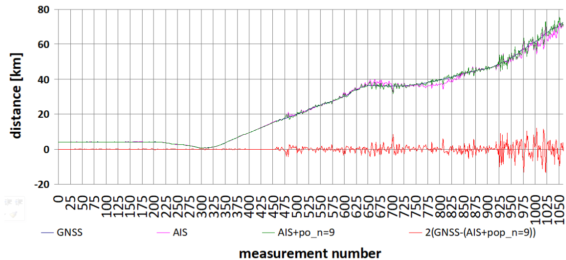
Figure 5: The results after adjusting for the moving average n = 9
