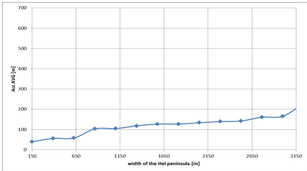
Figure 5-42: Hel peninsula influence for VDES
