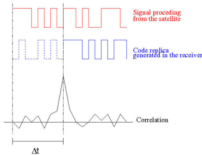
Figure 2-8: Correlation process
