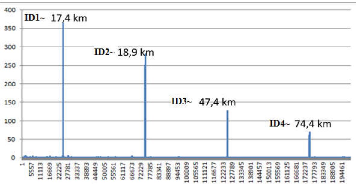
Figure 6-19: Correlation peaks for each of the slots
