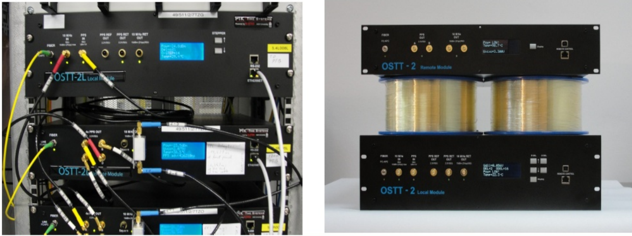
Fig. 5.5 ELSTAB technology – equipment to be installed for fiber optic T/F dissemination [4].
