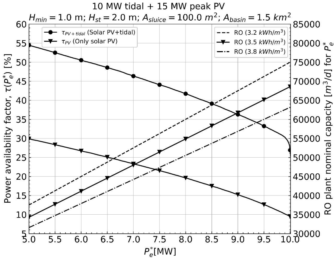
Figure 12. Power availability factors for a hybrid system 10 MW tidal range and 15 MW p PV at Broome, Australia. A_{sluice} = 100 \text{ m}^2 , A_{basin} = 1.5 \text{ km}^2 , H_{min} = 1 \text{ m} and H_{st} = 2 \text{ m} . Values for the only solar 15 MW p PV are given. Nominal SWRO plant capacity as a function of nominal power consumption is also shown for three different values of the SEC.
