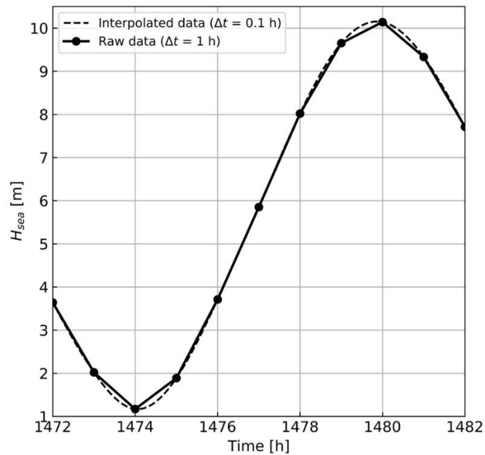
Figure 4. Comparison of raw and interpolated data of sea level ( H_{sea} ) at Broome (hour of the year in the x-axis).
