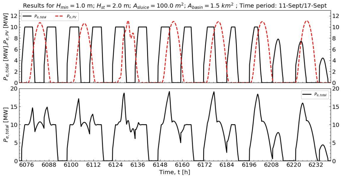
Figure 10. Power production of both 10 MW - tidal range and 15 MW peak PV plants and total power production in September at Broome.
