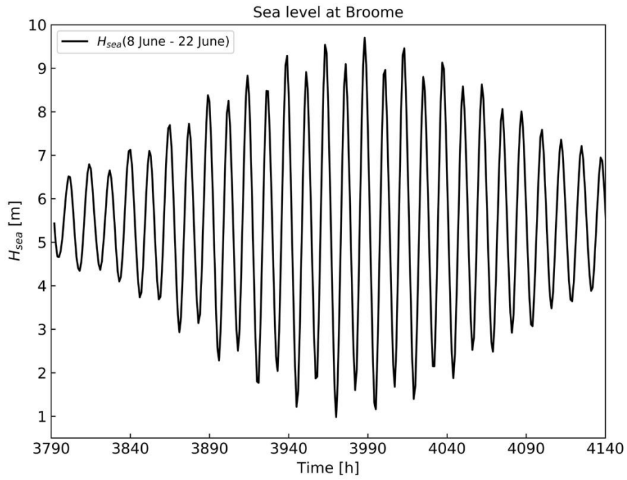
Figure 3. Exemplary behaviour of sea level ( H_{sea} ) where neap and spring tides are observed at Broome, Australia (hour of the year in the x-axis).
