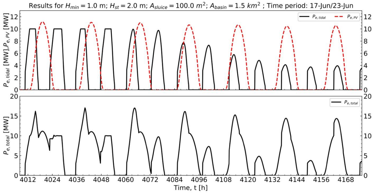
Figure 9. Power production of both 10 MW - tidal range and 15 MW peak PV plants and total power production in June at Broome.
