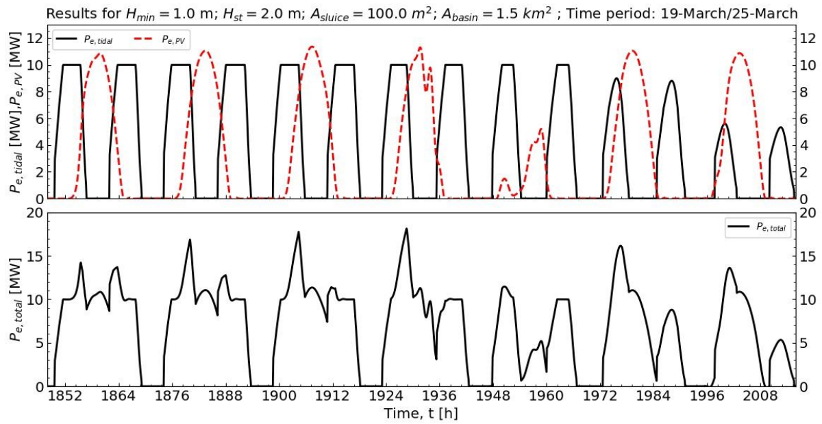
Figure 8. Power production of both 10 MW - tidal range and 15 MW peak PV plants and total power production in March at Broome.
