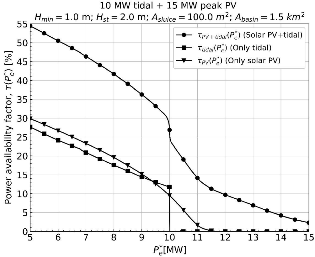
Figure 11. Power availability factors for a hybrid system 10 MW tidal range and 15 MW p PV at Broome, Australia. A_{sluice} = 100 \text{ m}^2 , A_{basin} = 1.5 \text{ km}^2 , H_{min} = 1 \text{ m} and H_{st} = 2 \text{ m} . Values for the only solar 15 MW p PV and only tidal 10 MW plants separately are given.
