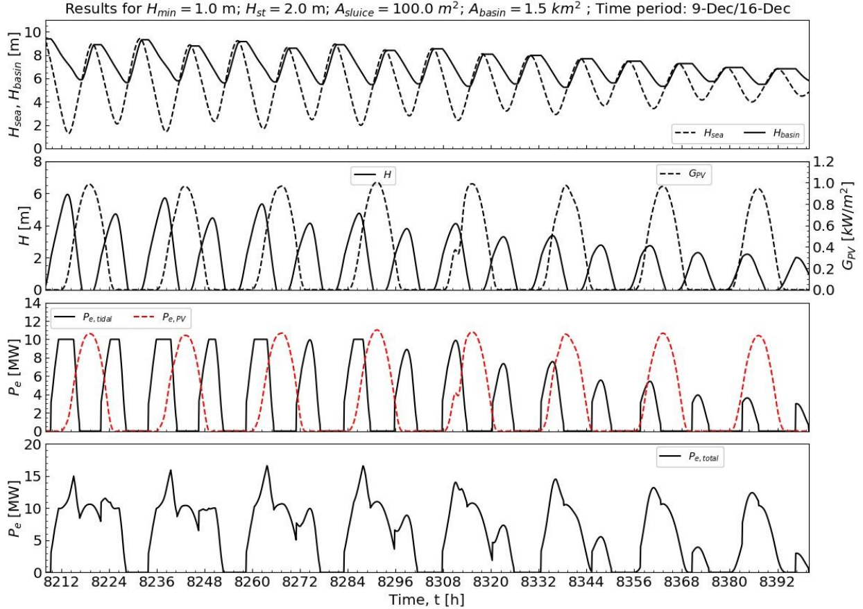
Figure 7. Full description of hybrid tidal range/solar PV system: Level of the sea and of the basin; tidal and solar resources represented by available head and solar irradiance on a North-oriented titled surface (18°); Power production of both 10 MW - tidal range and 15 MW peak - PV plants, and total power production in December at Broome.
