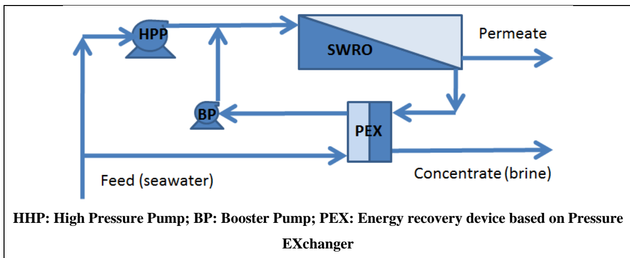
Figure 1. Conceptual diagram of the core of a SeaWater Reverse Osmosis (SWRO) desalination plant.
