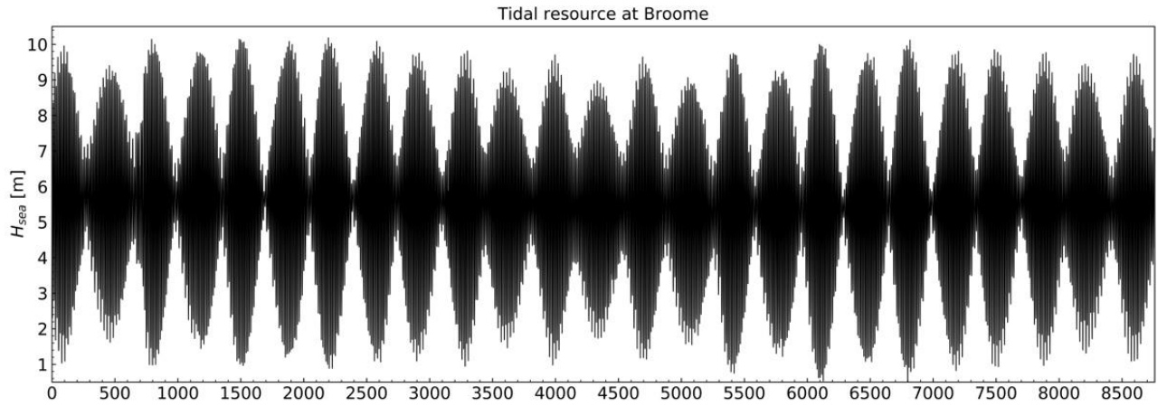
Figure 5. Sea level ( H_{sea} ) at Broome throughout the year 2018.
