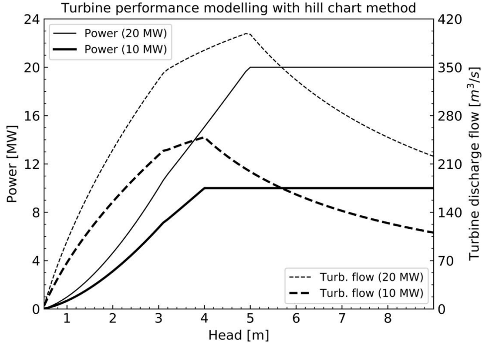
Figure 6. Model of selected turbine of 10 MW in comparison to that selected for the Swansea Bay Lagoon project (20 MW).
