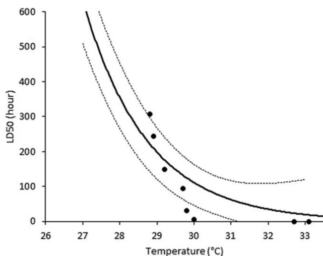
Fig. 2. The relationship between water temperature and LD50 (temperature inducing 50% survivorship) for larval Arctic Lamprey. LD50 = 3.855 \times 10^9 e^{-0.5787 \times \text{temperature}} . The ultimate incipient lethal temperature was estimated to be 29.3 °C. Reproduced from Arakawa and Yanai (2021) with permission.
