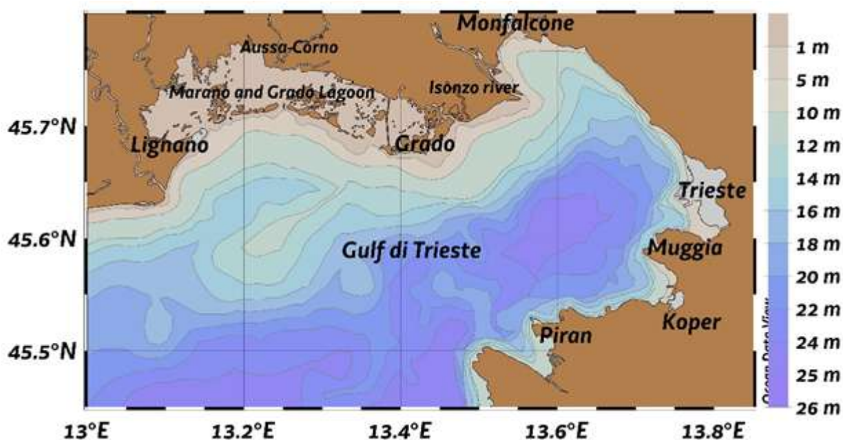
Figure 2.3.3. Bathymetry representation in the Gulf of Trieste
