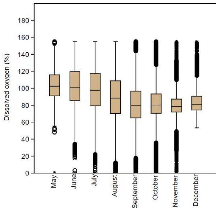
Figure 38. Dissolved oxygen values and their variability over the various months.
