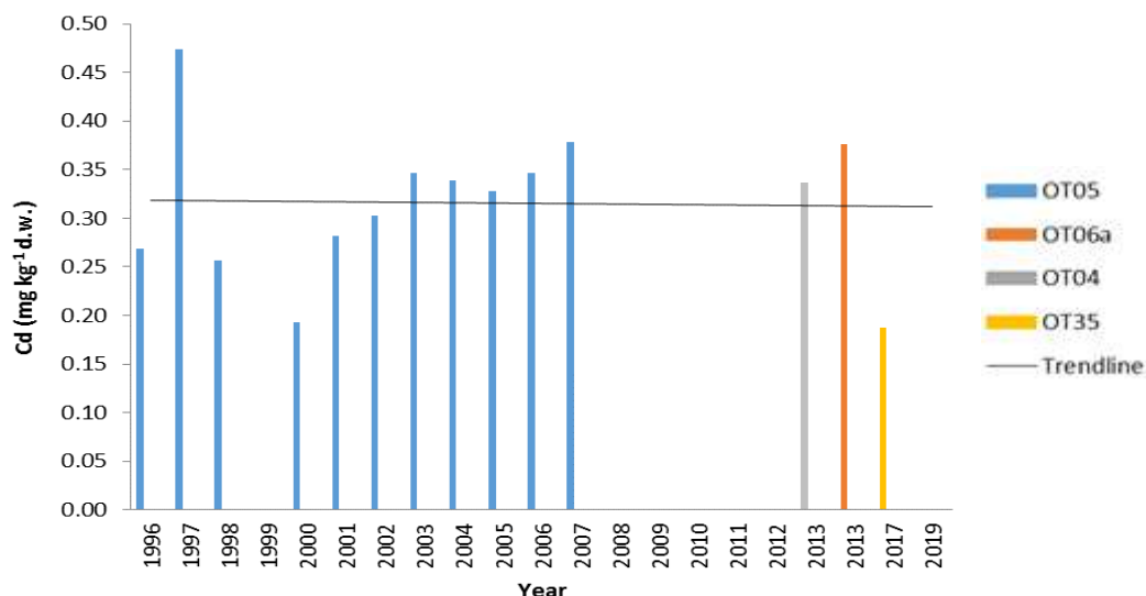
Figure 68. The concentrations of cadmium in sediment samples at OT05, OT06a, OT04 and OT35 stations in period 1996-2019.
