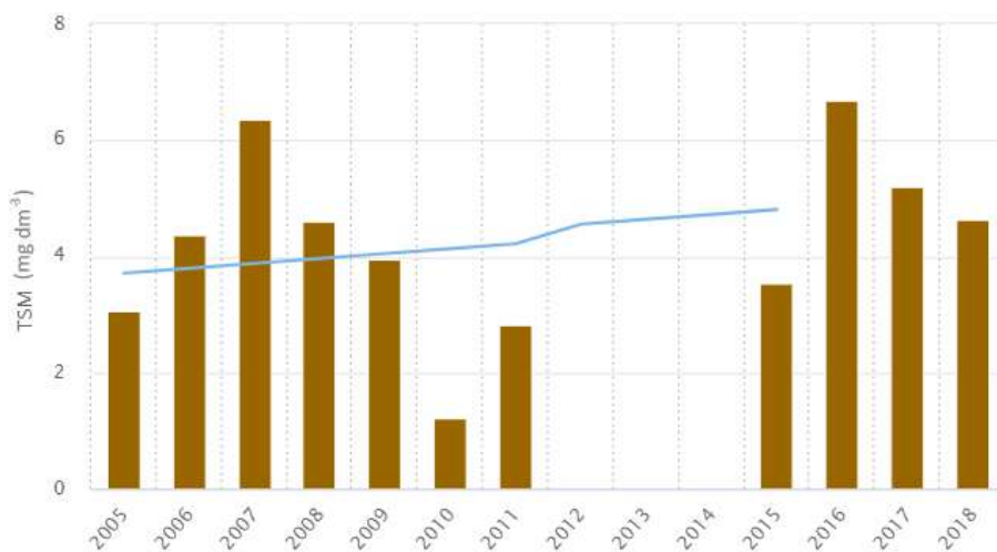
Figure 88. Total suspended matter at OCO3 station in period 2005-2018.
