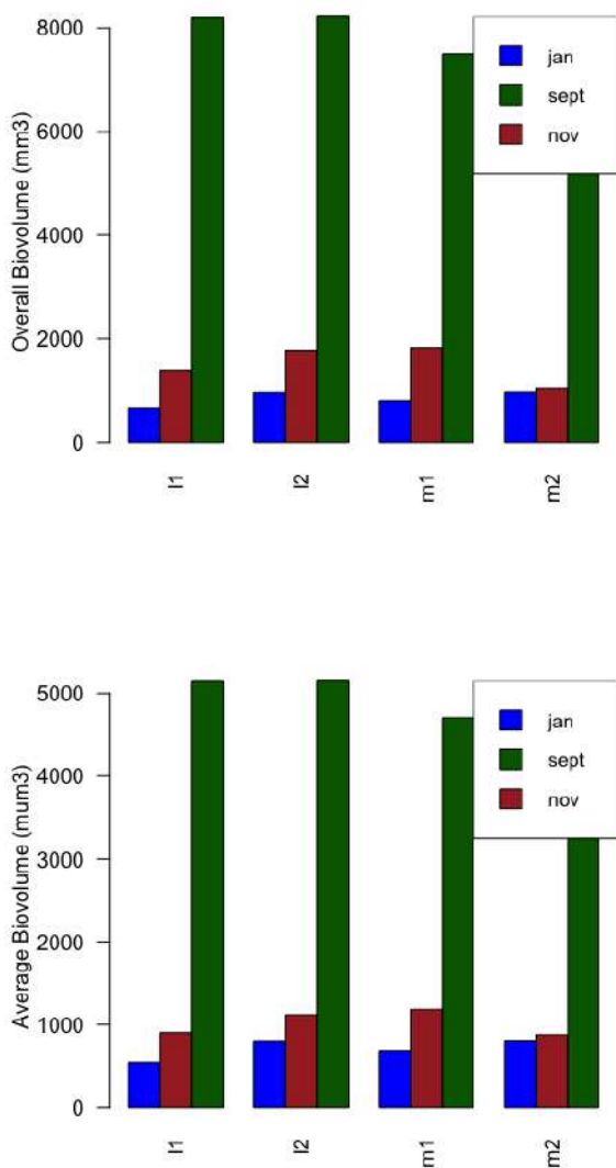
Figure 66. Overall and average biovolume of Torre Guaceto marine phytoplankton across different months.
