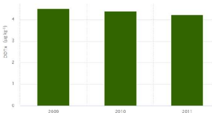
Figure 83. DDTx in shellfish samples at OT06 station in period 2009-2011.
