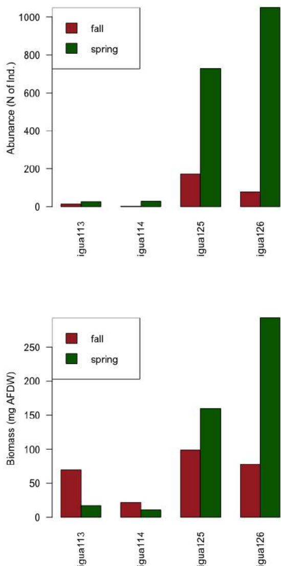
Figure 64. Individual abundances and overall biomass of Torre Guaceto Transitional Water Macrozoobenthos across different season.
