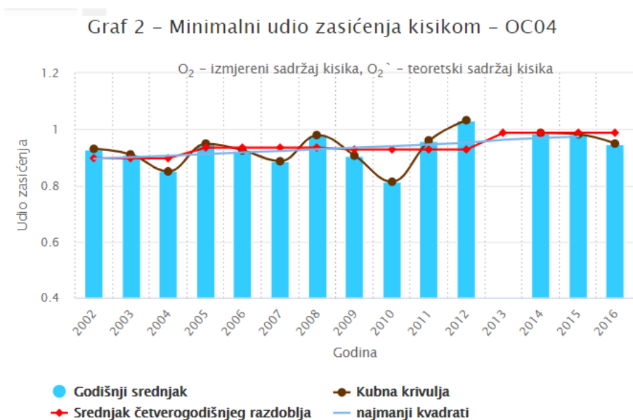
Figure 131. Minimum proportions of oxygen saturations in the bottom layer of Cetina estuary (in order of appearance: annual mean, the mean of a four-year period, cubic curve, smallest squares).
