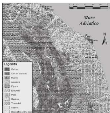
Figure 136. Lithological scheme of the region.
