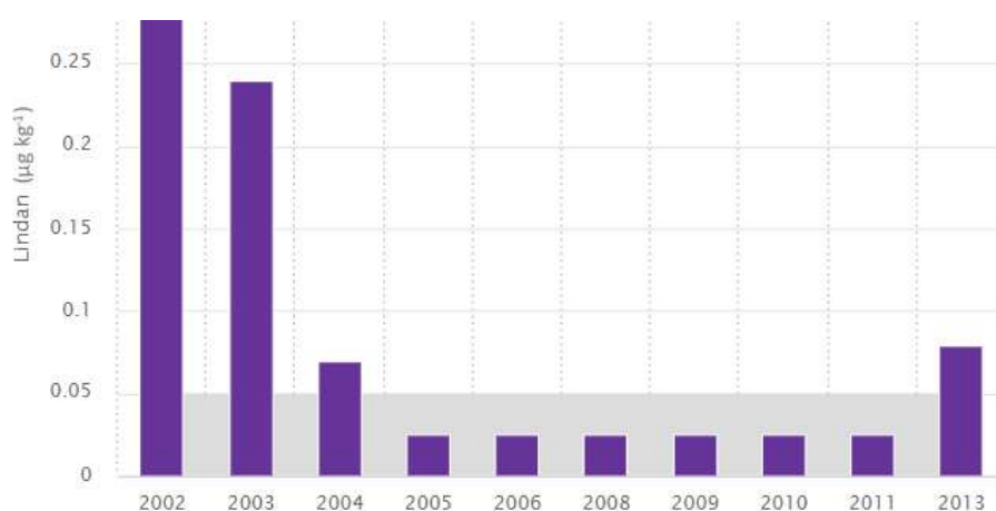
Figure 81. Lindane in shellfish samples at OT04 station in period 2002-2013 (concentrations in bivalve tissue expressed as a dry weight of 0.025 indicate that the amount is below the detection threshold (<0.05)).
