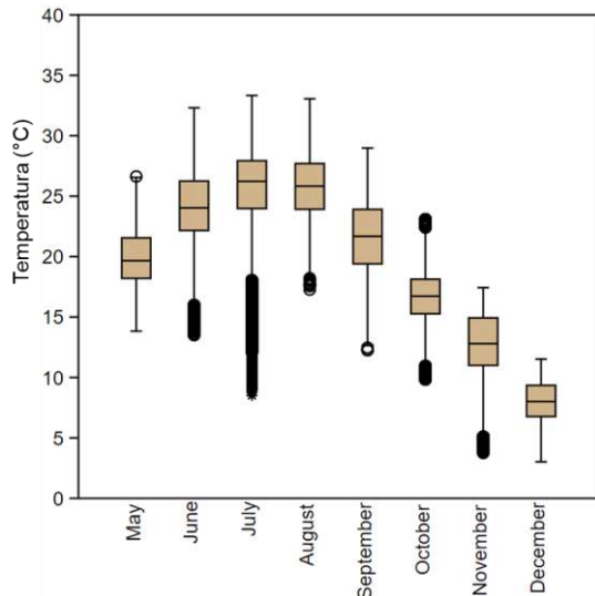
Figure 35. Water temperature values and their variability over the various months.
