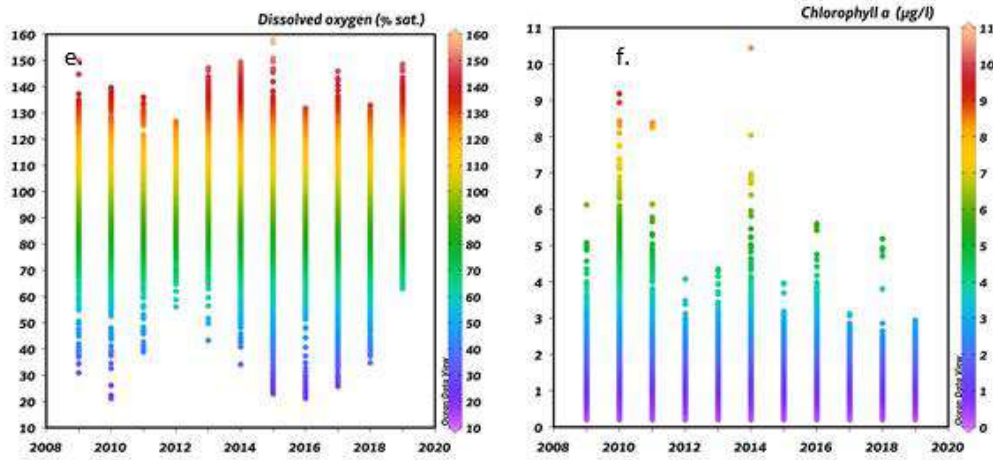
Figure 32. Graphs of physical and chemical data collected in the Gulf of Trieste (a) temperature; (b) salinity; (c) turbidity; (d) pH; (e) dissolved oxygen; (f) chlorophyll-a.
