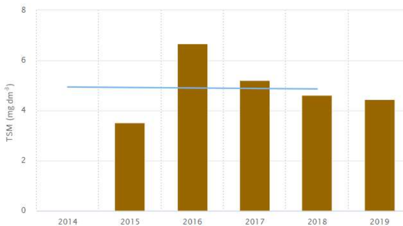
Figure 89. Total suspended matter at OCO3 station from 2014-2019.
