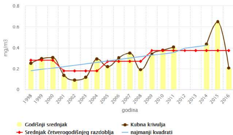
Figure 129. Average annual values of chlorophyll a concentration in the surface layer of Cetina estuary (in order of appearance: annual mean, the mean of a four-year period, cubic curve, smallest squares).
