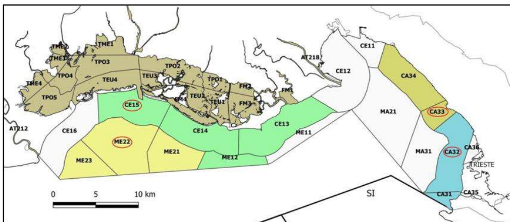
Figure 29. Regional water bodies of transitional and marine-coastal waters. The four groups for coastal marine waters are highlighted in different colours. (ArpaFVG and SNPA, Monitoraggio delle acque di transizione e marino costiere della Regione Friuli Venezia Giulia (D.Lgs. 152/2006)).
