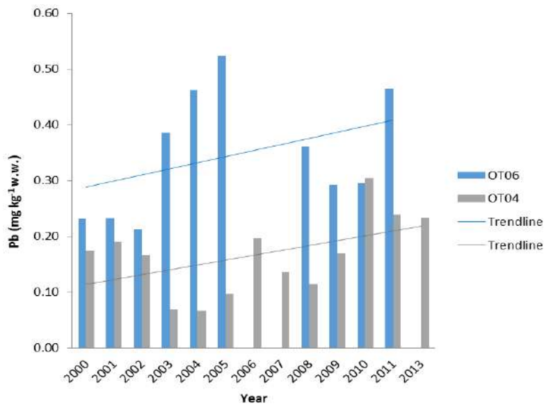
Figure 75. The concentrations of lead in shellfish samples at OT06 and OT04 stations in period 2000-2013.
