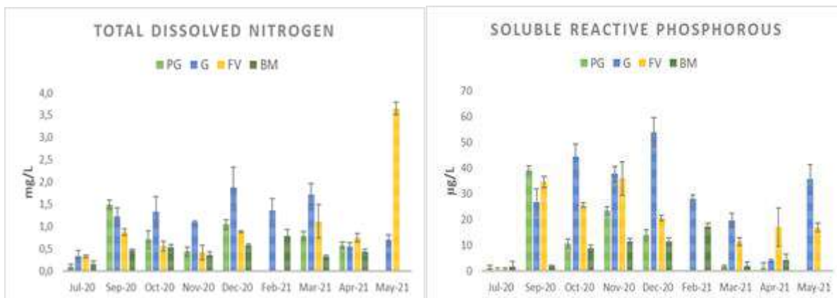
Figure 47. Total dissolved nitrogen (left) and soluble reactive phosphorous (right) concentration in the Sacca di Goro.
