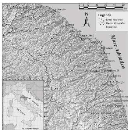
Figure 135. Orographic diagram of the region.
