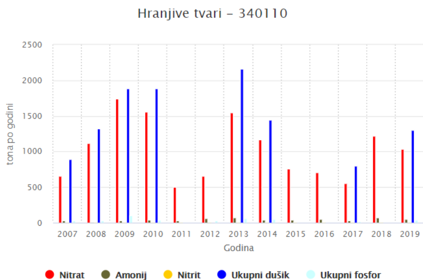
Figure 115. Annual quantities of nutrients introduced by watercourses into the coastal part of the sea (in order of appearance: nitrate, ammonium, nitrite, total nitrogen, total phosphorus).
