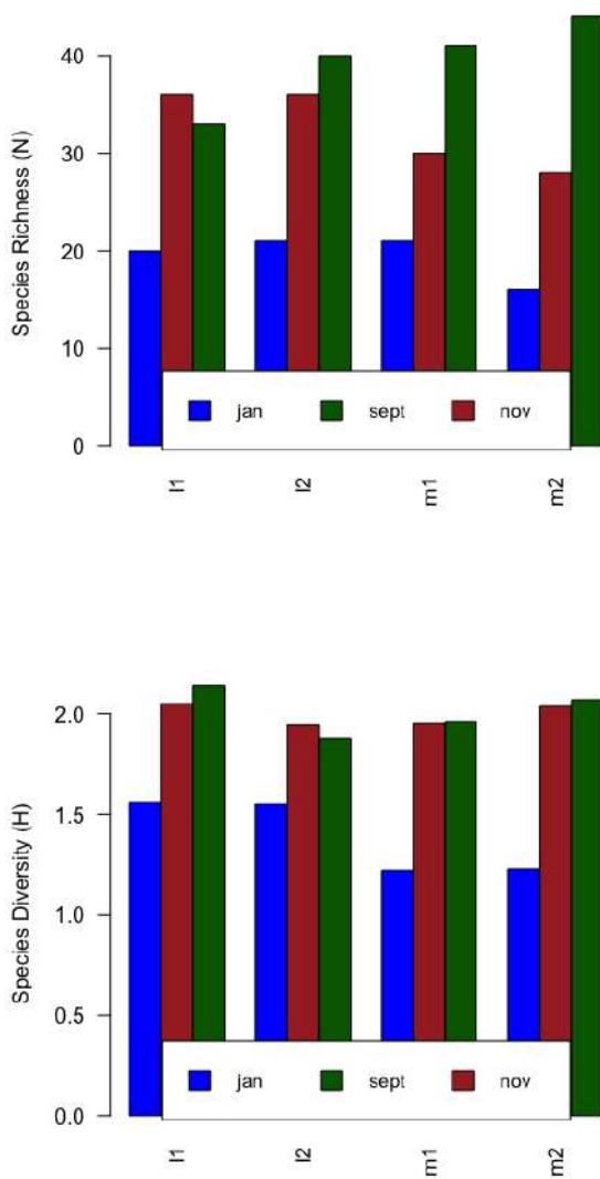
Figure 65. Species Richness and Diversity of Torre Guaceto marine phytoplankton across different months.
