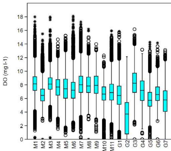
Figure 37. A comparison of the entire pool of values obtained on the different sites investigated.
