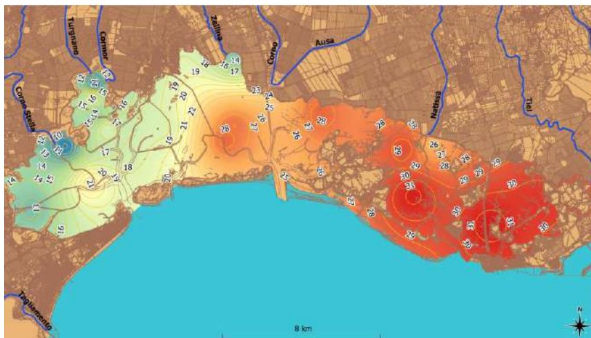
Figure 36. Interpolation of average salinity values (2013-2020 data) on the lagoon basin. The iteration between the river mouths and the lagoon mouths is highlighted on the map, as well as the different characteristics relating to the western portion (Marano Lagoon) and the eastern one (Grado Lagoon).
