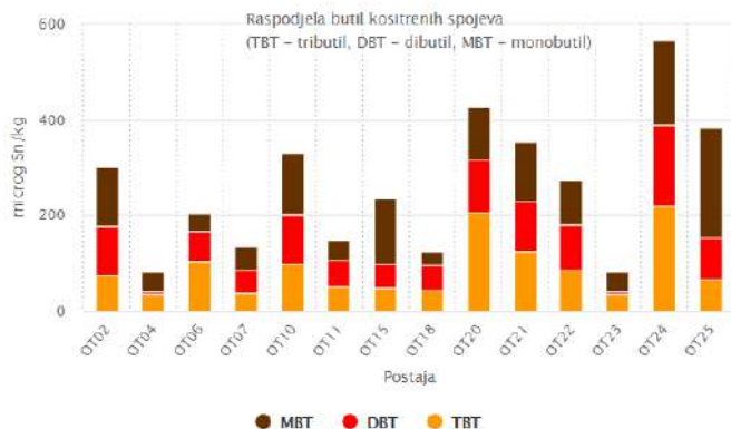
Figure 124. Average annual concentration of organotin compounds in mussels of Cetina estuary (station OT07, values: TBT = 35,8 microg/kg, DBT = 48,2 microg/kg, MBT = 50,2 microg/kg).
