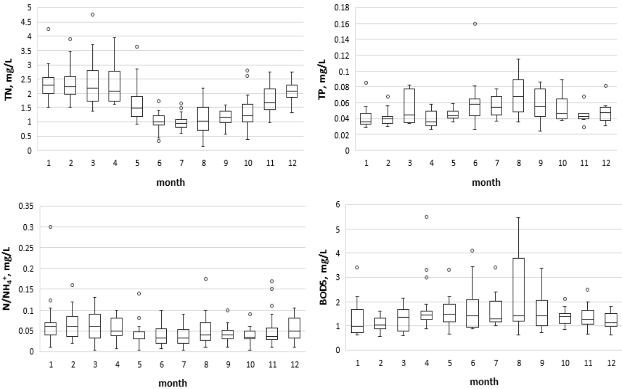
Figure 4.1.3. Seasonal changes of nutrient and BOD5 concentration in Salaca river upstream Salacgrīva.
