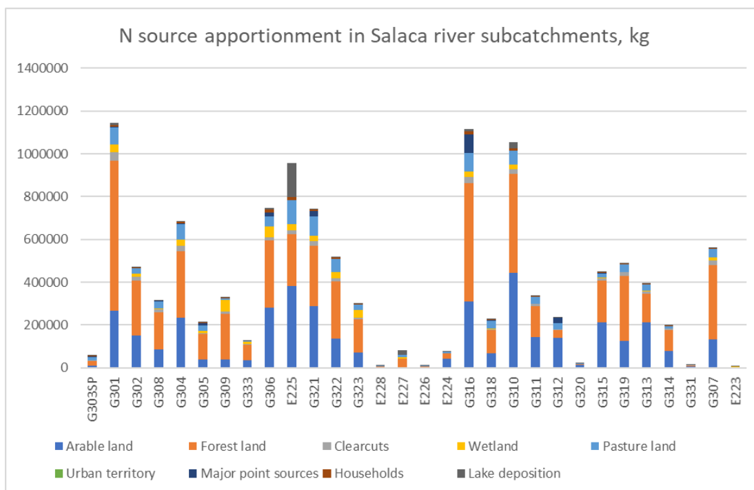
Figure 7.1.3. Salaca N source apportionment on a subcatchment level.
