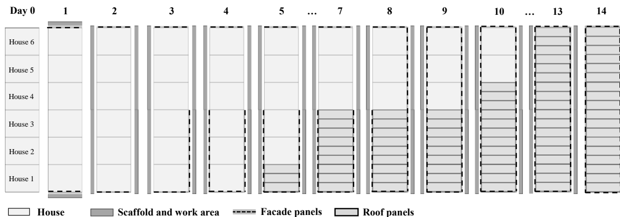
Figure 5. Process and planning of a six-dwellings terraced house.
