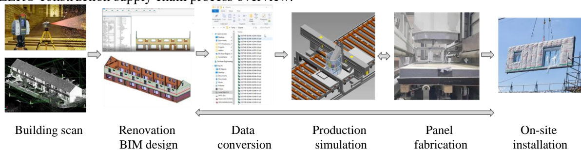
Figure 3. Future INDU-ZERO construction supply chain process overview.
