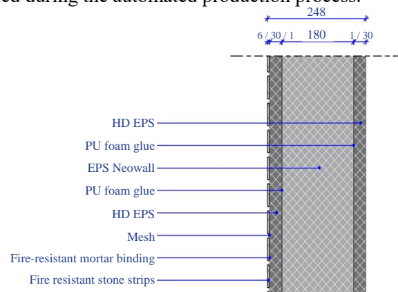
Figure 1. Assembly of the wall component design: sandwich panel.
