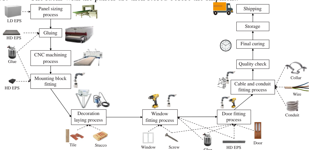
Figure 4. Smart Construction Factory production process and used machinery.
