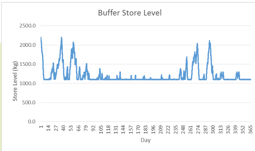
Figure 23. The buffer store level required to prevent the need for an additional compressor
