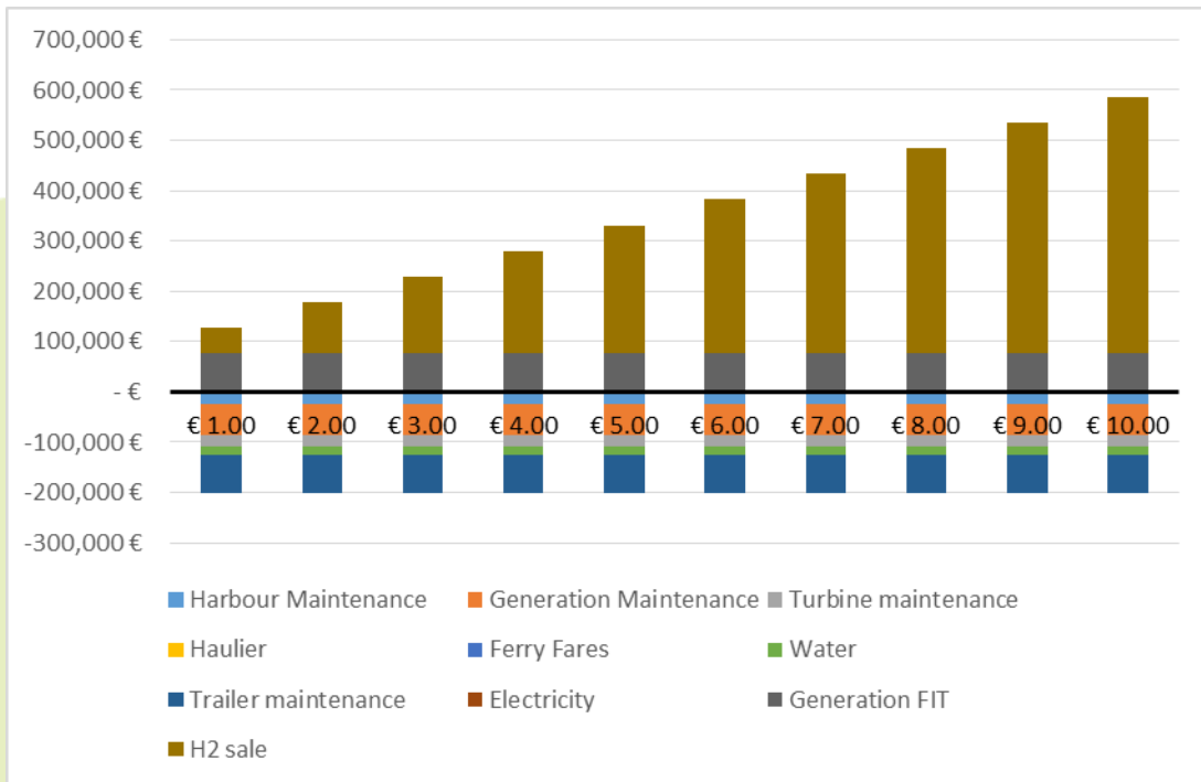
Figure 35. The breakdown of income and expenditure for the slow fill of vessels via a pipeline at Shapinsay Harbour for a range of hydrogen sale prices (€/kg)
