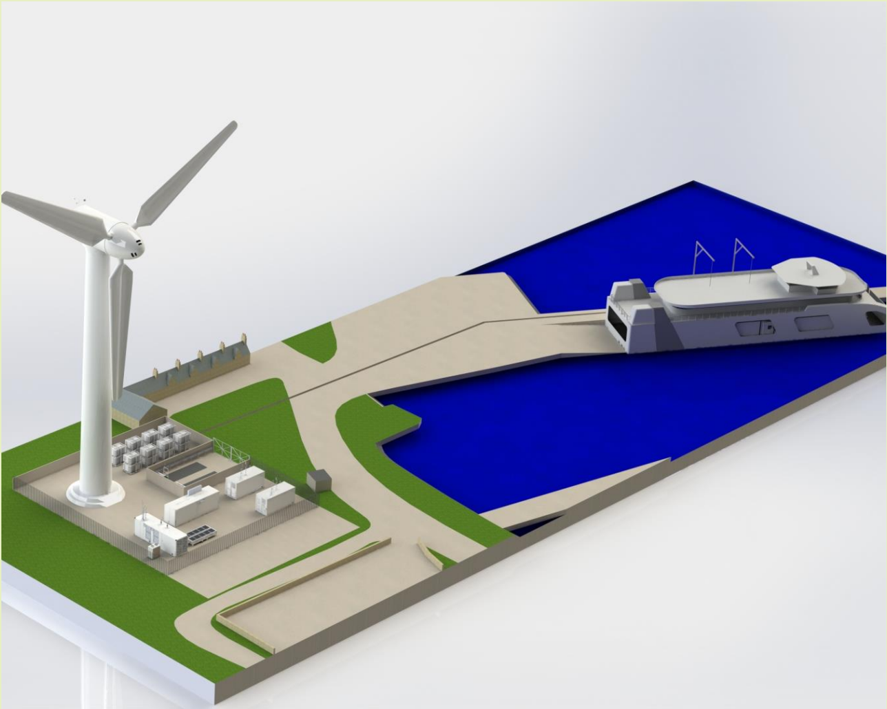
Figure 26 - Example layout of the site containing the site for the hydrogen equipment, pipeline and dispensing equipment on the harbour.
