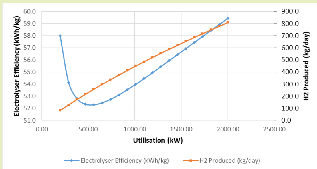
Figure 7: Indication of HGas system efficiency and H 2 production as a function of kW input when new
