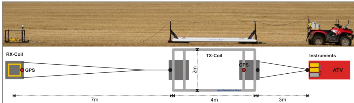
Figure 2. The tTEM system. Rx Coil are the receiver coil and Tx is the transmitter coil. The exact distance and device positions are listed in Table 1.
