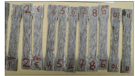
Fig. 5: Milled test samples from 1:1 model and tension test with optical strain measurement
