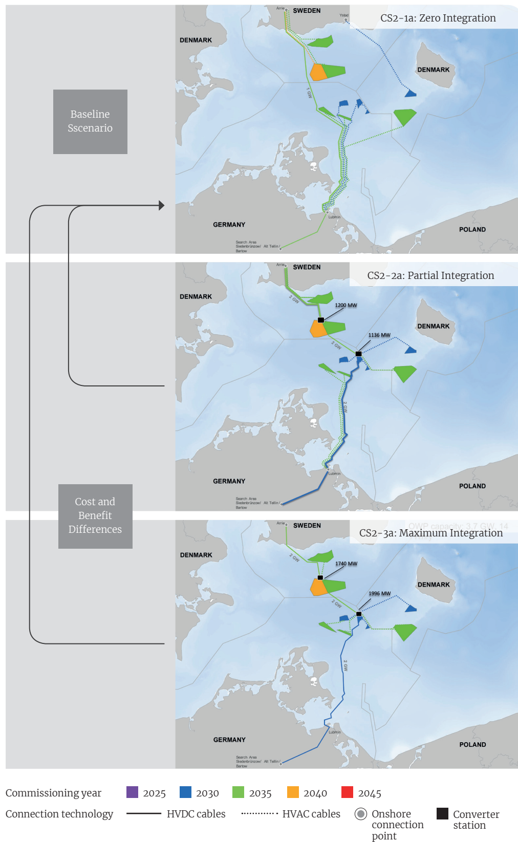
Figure 6 Case study 2 with high offshore wind installation
