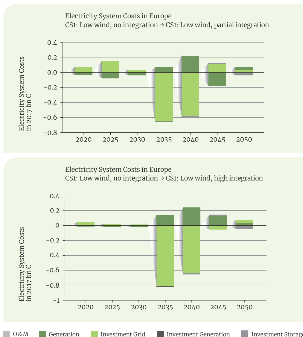
Figure 8 Total system costs: case study 1 – low wind
