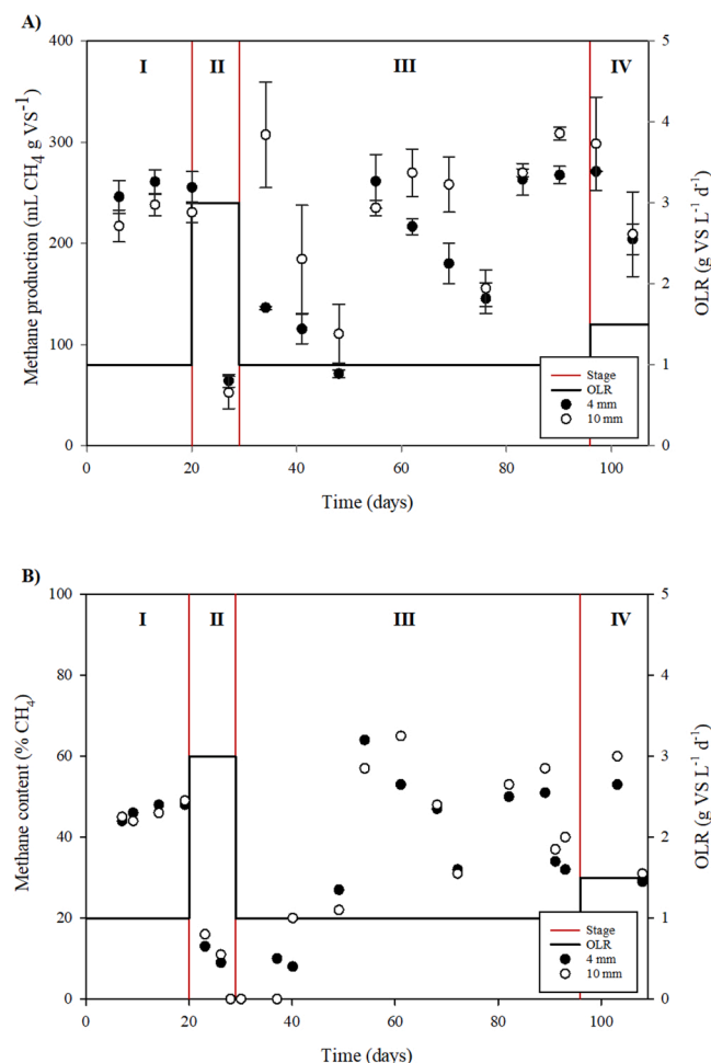
Fig. 2. A) Weekly variation of methane production (mL CH 4 g VS -1 ) and B) daily variation methane content (% CH 4 ), according to particle size, under the different organic loading rates (OLR) during the experimental time.
