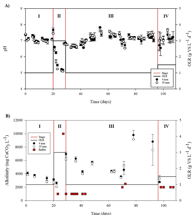
Fig. 3. Daily variation of A) pH and B) alkalinity (mg CaCO 3 L -1 ), according to particle size, under the different organic loading rates (OLR) during the experimental time.
