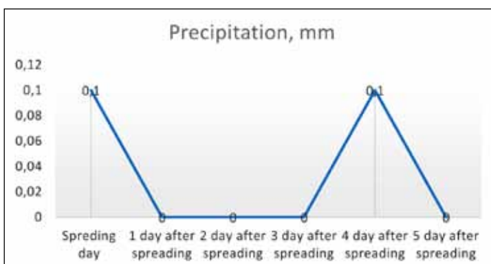
Figure 10. Precipitation, mm on field trial field (six consecutive days).
