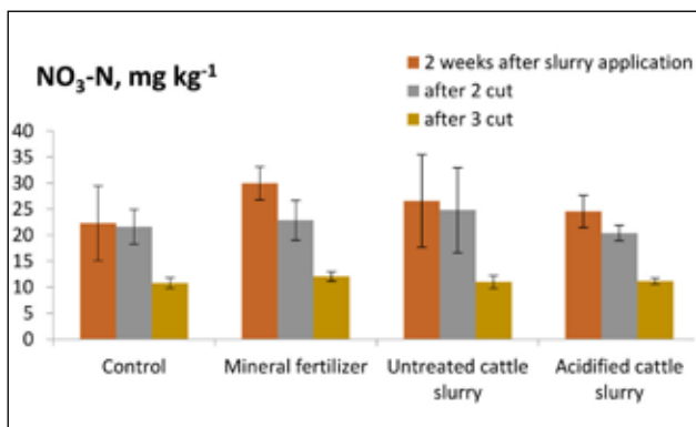
Figure 9. Amount of NO 3 -N in soil during the experiment between treatments. The error bar refers to the standard deviation of the mean (n=4).
