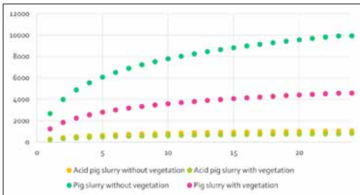
Figure 17. Ammonia cumulative emissions within twenty-four hours after the spreading of slurries g h -1 ha -1 .
