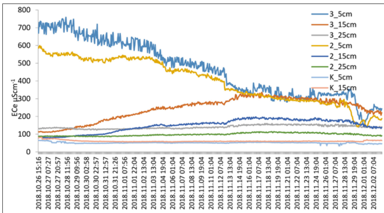
Figure 11. Depth and time dynamics of total dissolved nutrients (Ece) in soil layers due to slurry (2) and acidified slurry (3) vs. control (K) from Percostation data at Jögeva trial field, BSA project.
