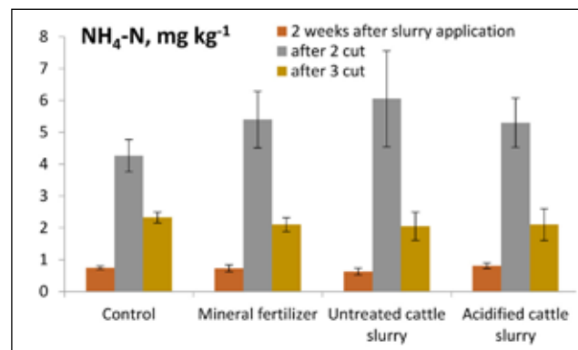
Figure 10. Amount of NH 4 -N in soil during the experiment between treatments. The error bar refers to the standard deviation of the mean (n=4).
