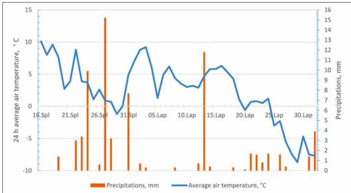
Figure 10. Average air temperature and precipitation on Jögeva trial site 16.10.2018-1.12.2018.
