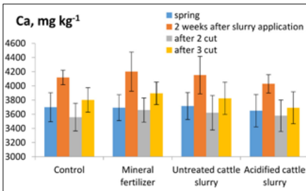
Figure 3. Amount of Ca in soil during the experiment between treatments. The error bar refers to the standard deviation of the mean (n=4).
