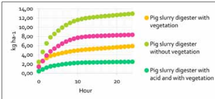
Figure 26. Cumulative ammonia emissions per hour.
