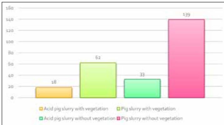
Figure 16. Ammonia emissions twenty-four hours after the slurry dispersal g h -1 ha -1 .
