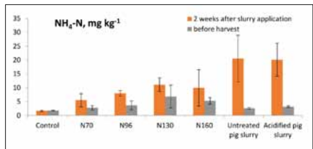
Figure 10. Amount of NH_4 -N in soil during the experiment between treatments. The error bar refers to the standard deviation of the mean ( n=4 ).
