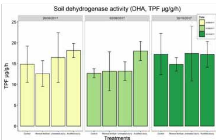
Figure 13. Soil dehydrogenase activity (DHA, TPF \mu\text{g/g/h} ). The error bar refers to the standard deviation of the mean ( n=4 ).
