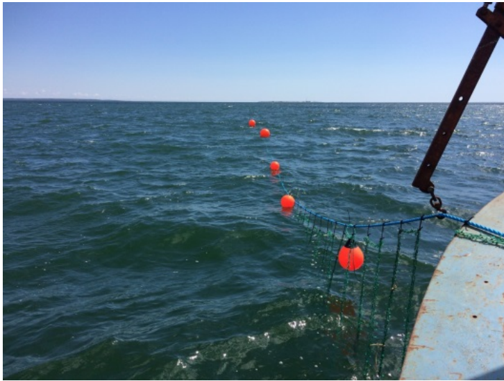
Figure 4: The pilot mussel farm at Vormsi use coils of trawl net as mussel- substrate.
